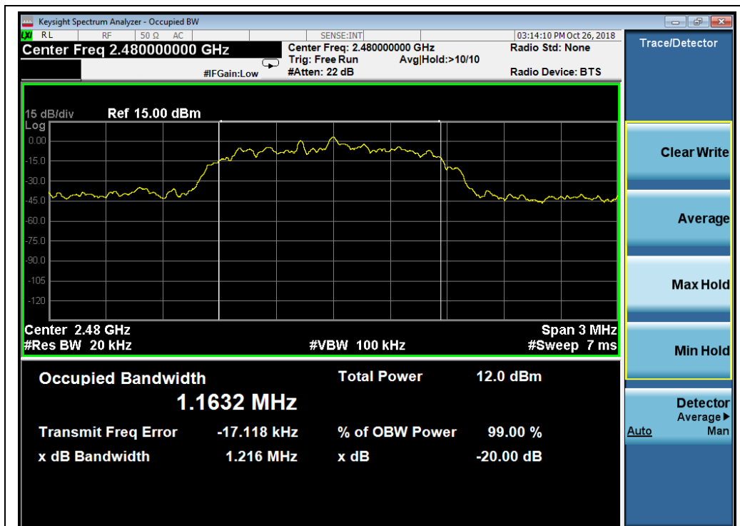
(π/4-DQPSK, Channel 78, 2480MHz)
