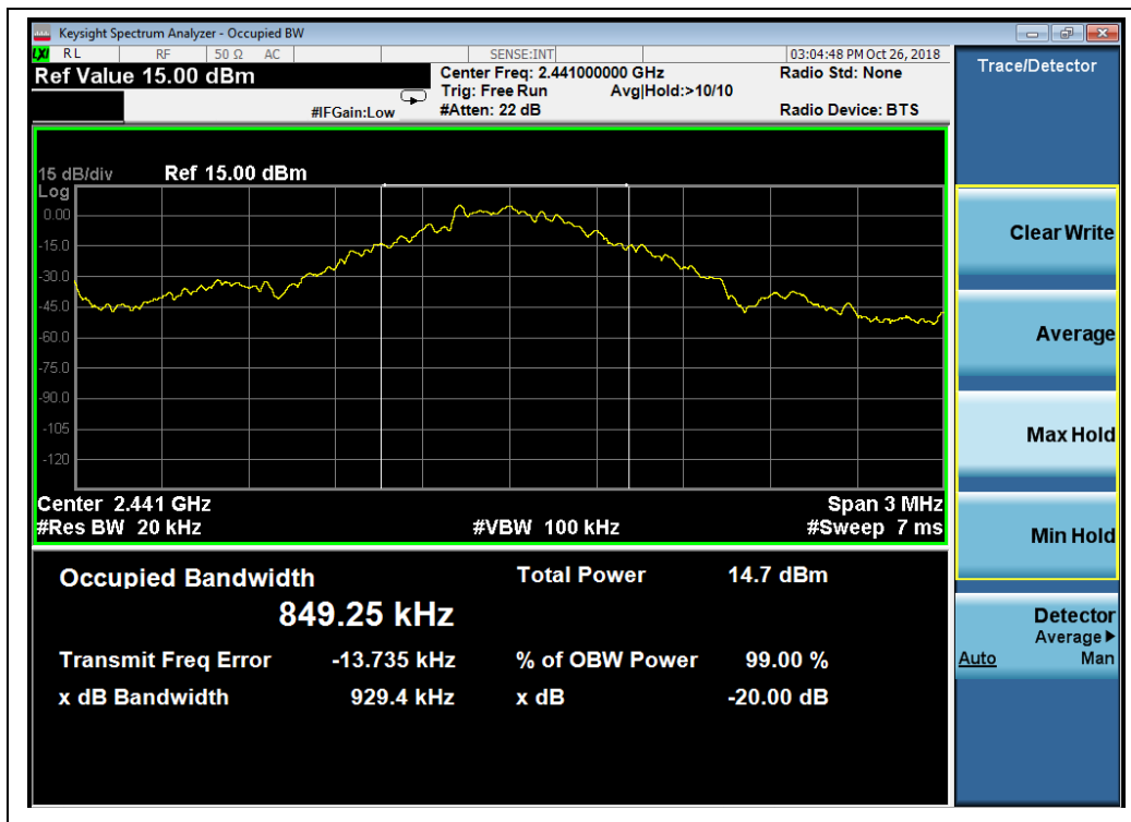
(GFSK, Channel 39, 2441MHz)
