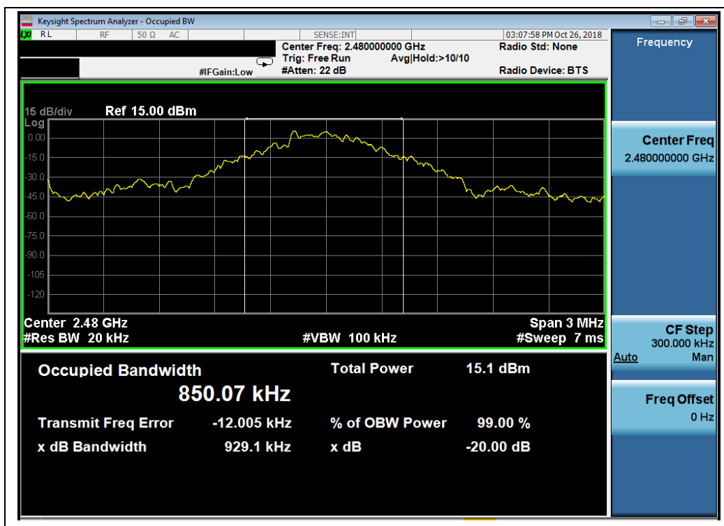
(GFSK, Channel 78, 2480MHz)
