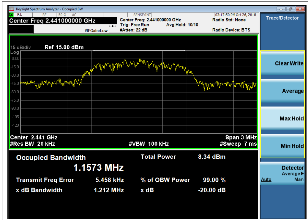
(8-DPSK, Channel 39, 2441MHz)
