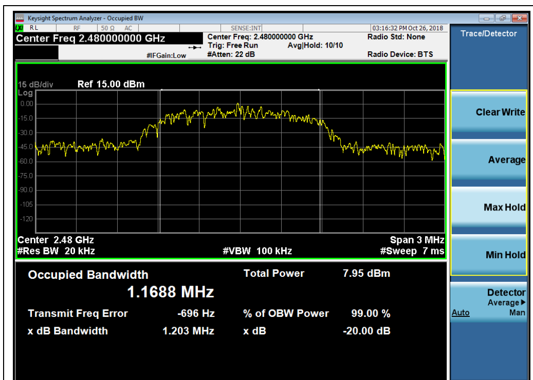
(8-DPSK, Channel 78, 2480MHz)
