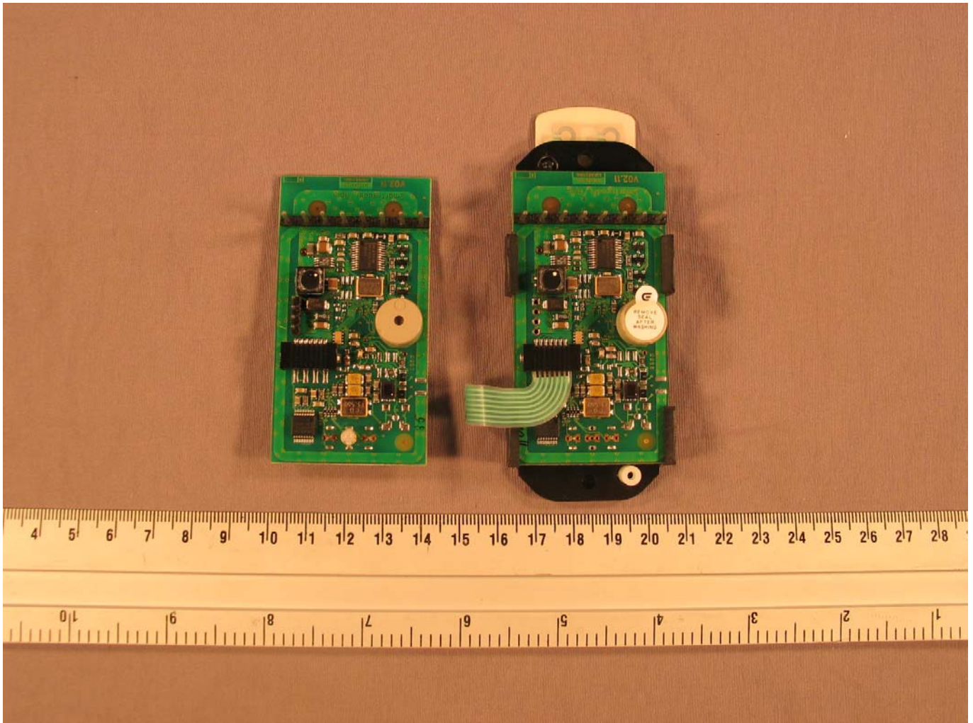
Photo 1 PCB with (right) keypad and without (left) keypad
