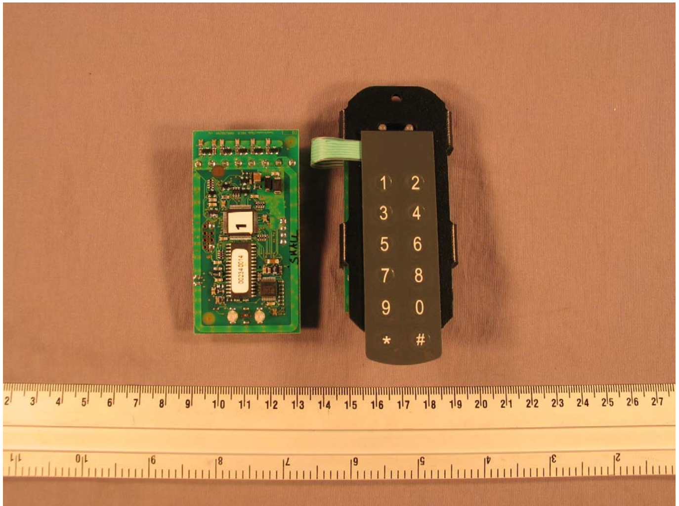
Photo 2: PCB with (right) key pad and without (left) keypad
