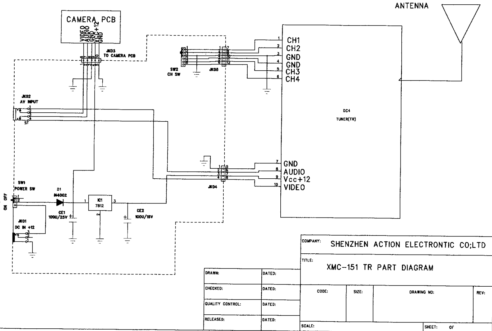
Schematic Diagram
