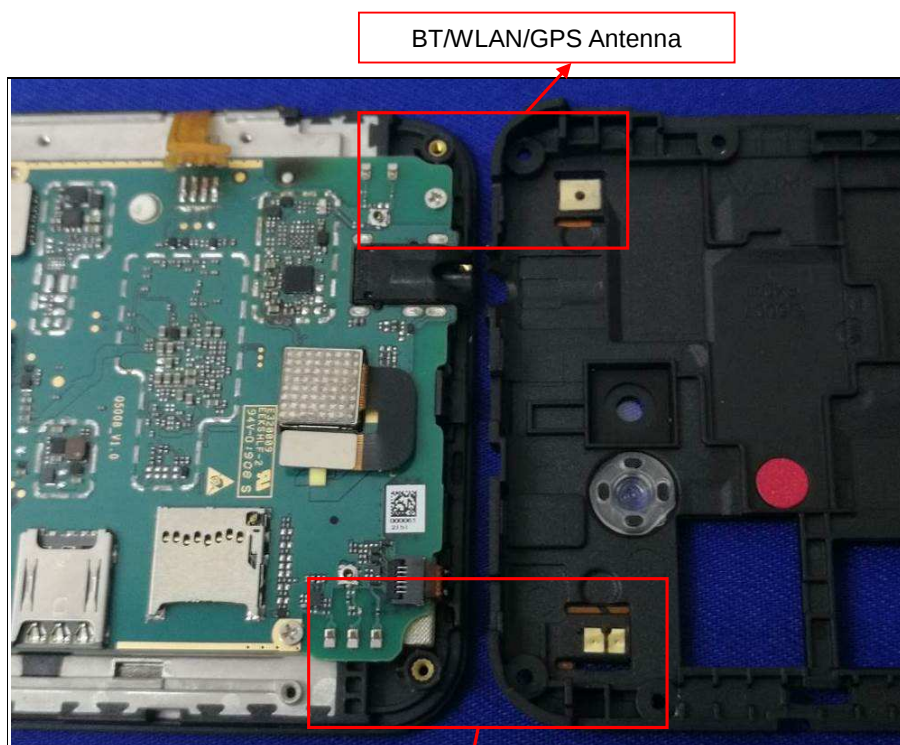
Diversity Antenna
