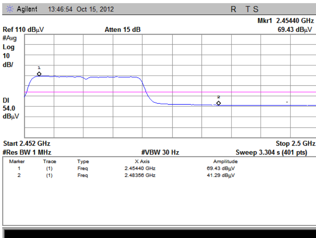
(Plot F2: Channel = 11 AVG @ 802.11n)
