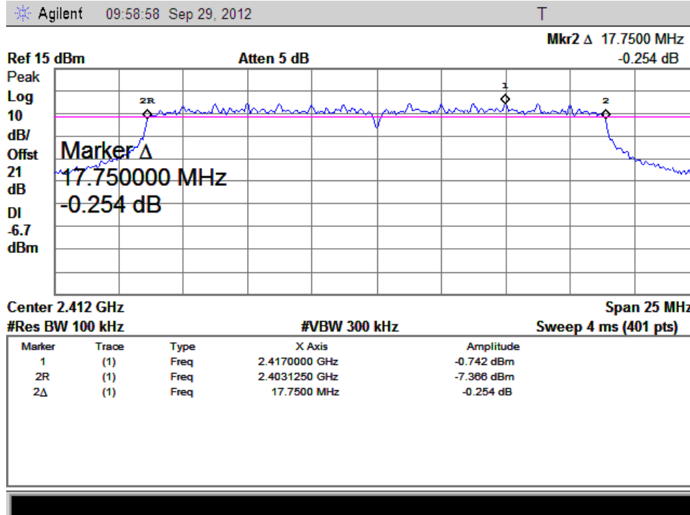
(Plot G: Channel 1: 2412MHz @ 802.11g)
