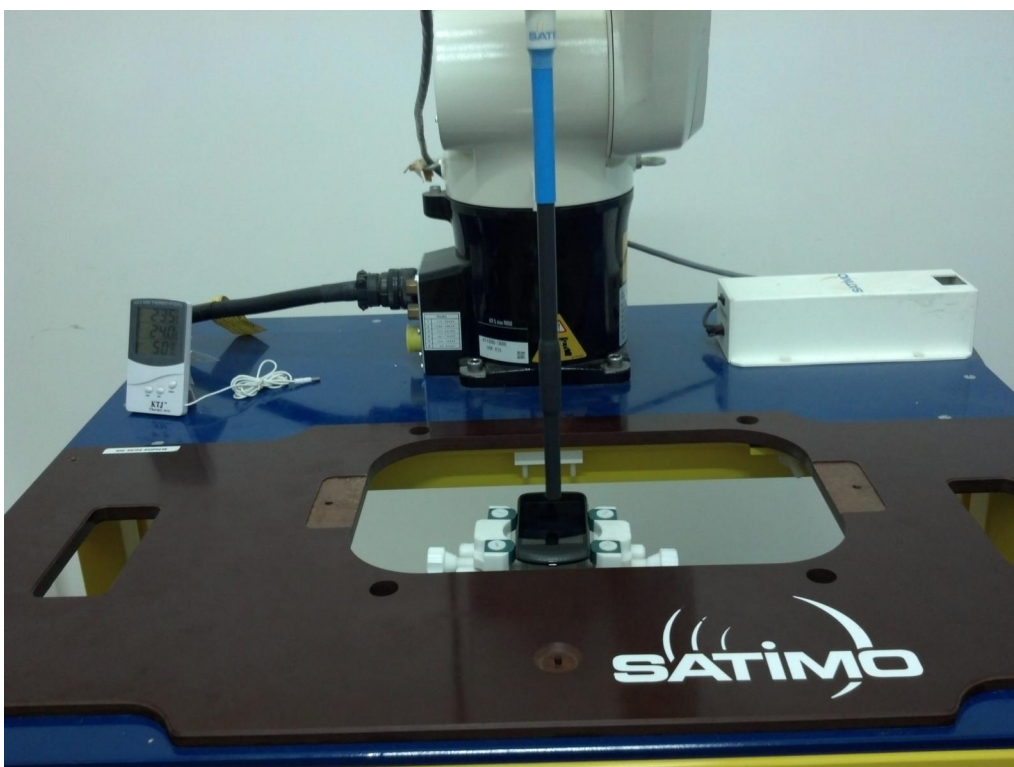
H-Field
