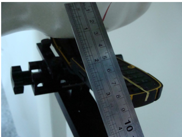
Left Tilted position - Separation distance 8.0cm between mouth and antenna
