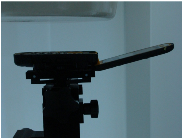
Left Cheek position - Separation distance 4.5cm between mouth and antenna
