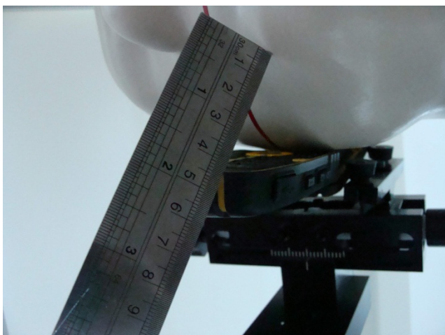
Right Cheek position - Separation distance 4.2cm between mouth and antenna
