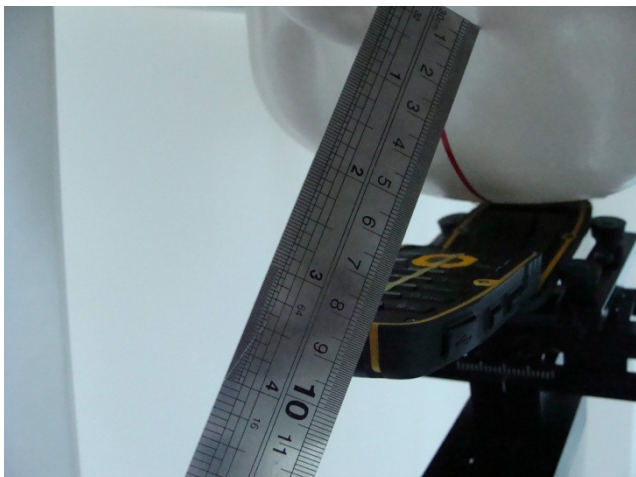
Right Tilted position - Separation distance 7.8cm between mouth and antenna
