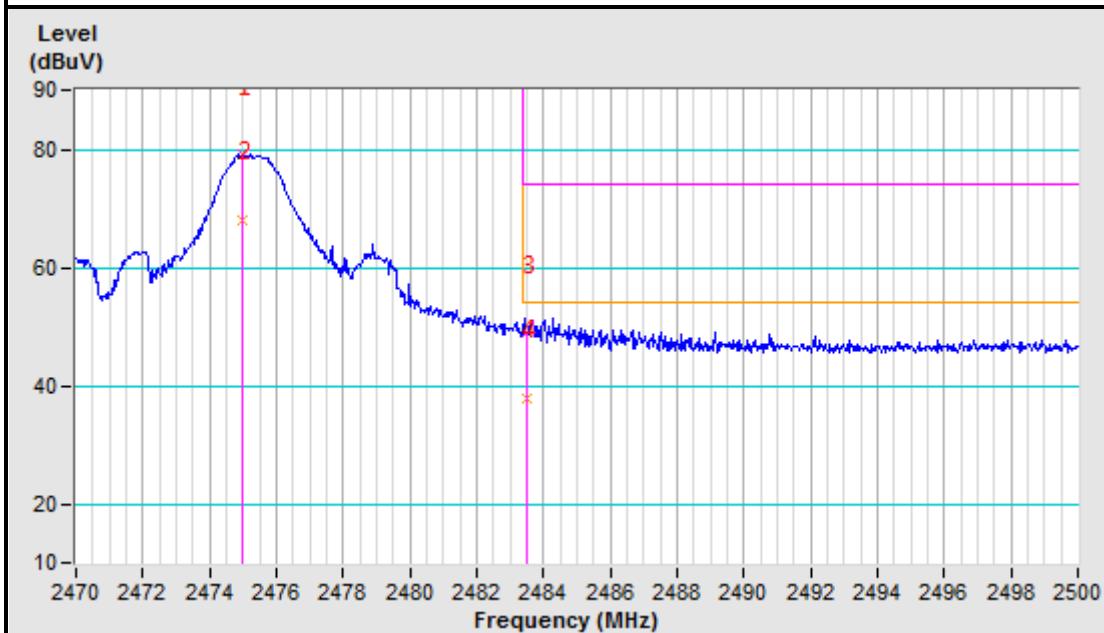
2475MHz Vertical
