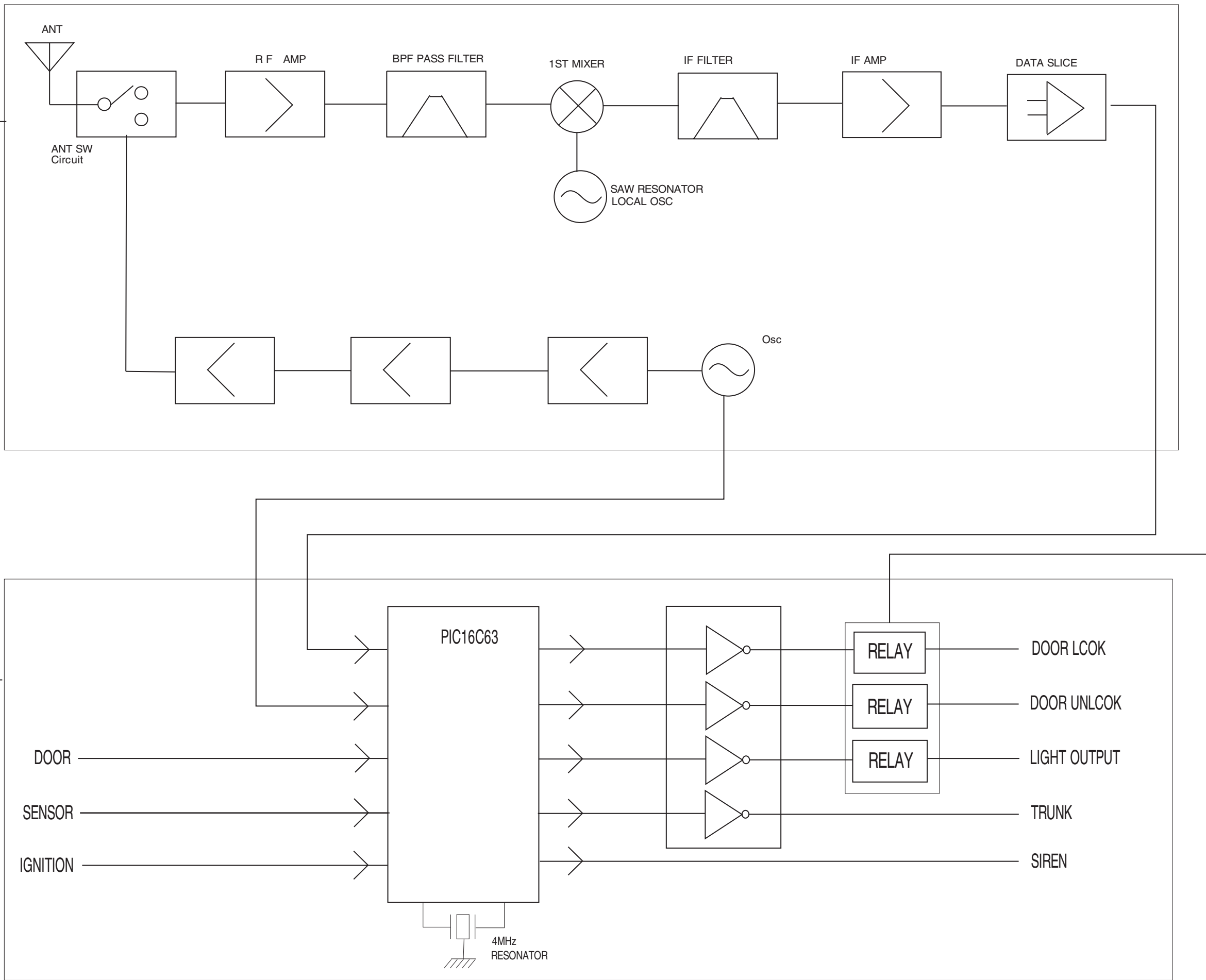
CONTROL- MODULE & TRANSCEIVER BLOCK DIAGRAM
