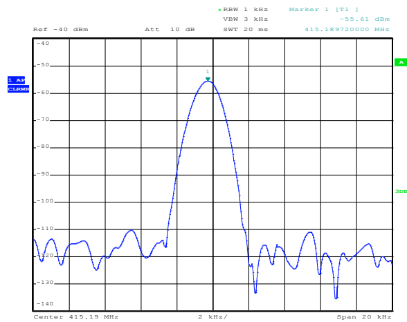
Figure 8.1-1: output power
