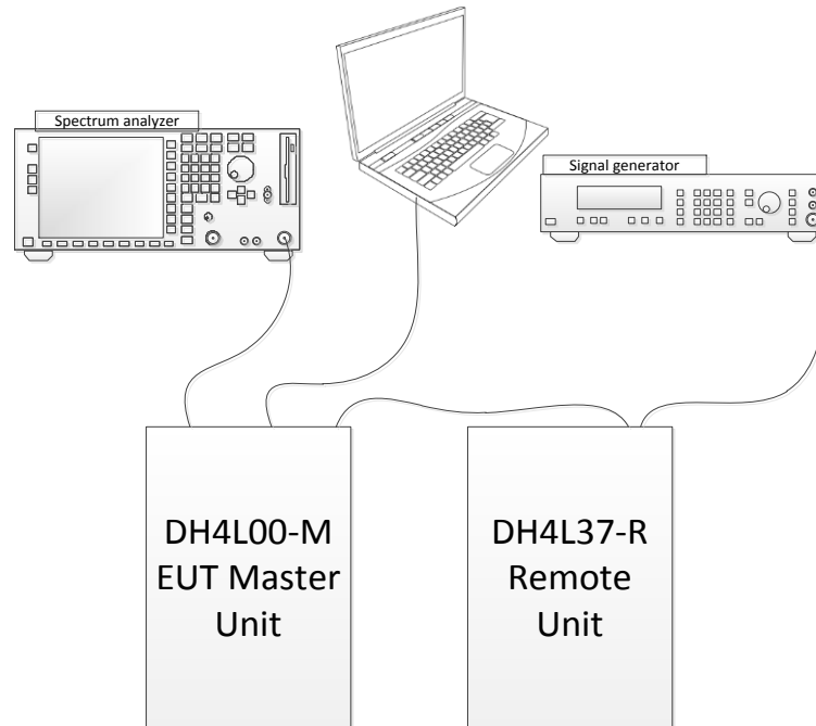
Figure 3.6-1: Setup diagram
