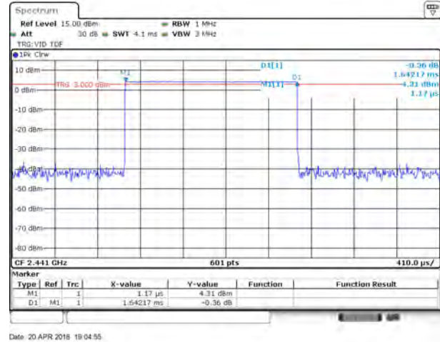
GFSK DH3
