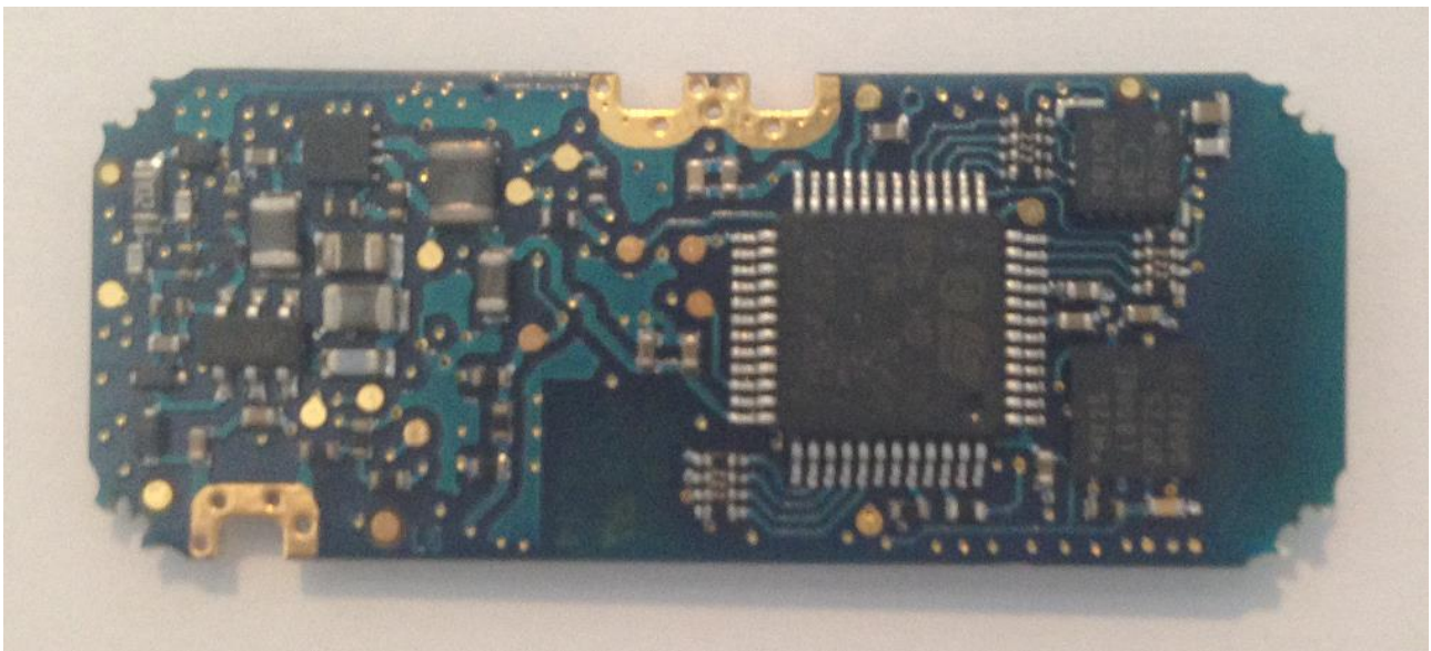
Bottom view
