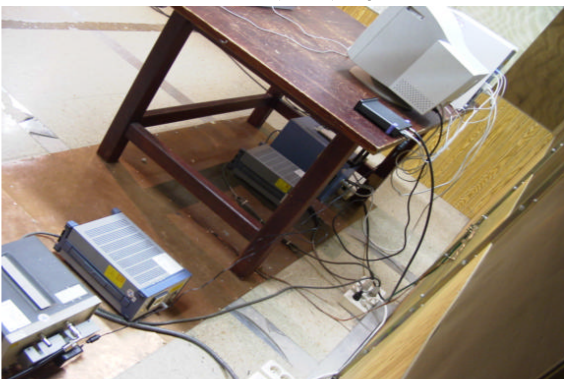
Conducted Emissions(Backview) – Ping Mode
