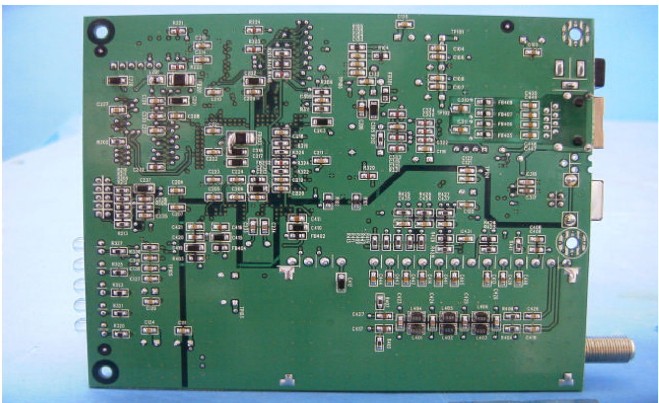
Copper Side of Mainboard
