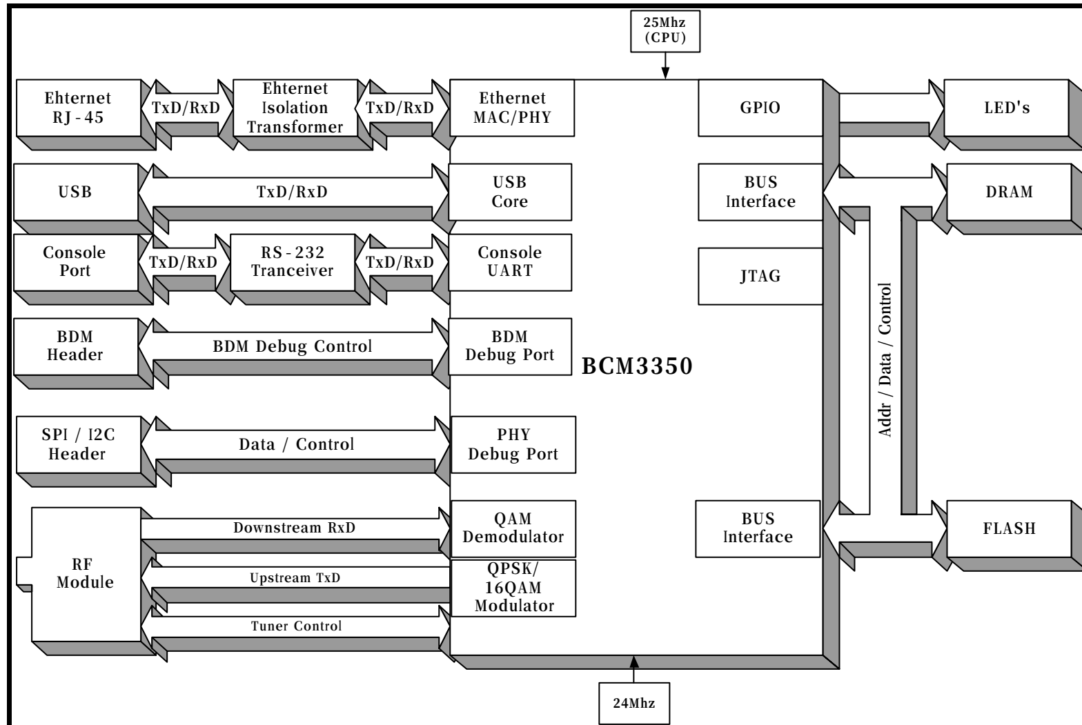
Block Diagram MNG -2000
