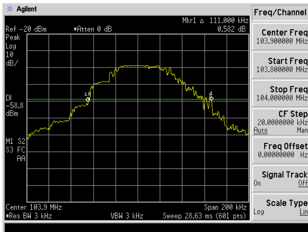
Plot 6.1.3. 20dB Bandwidth Plot (High Channel: 103.9MHz)
