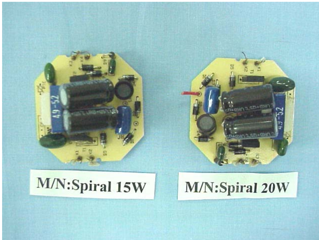
FIGURE 2 LIGHT(M/N: SPIRAL-15W, SPIRAL-20W) MAIN BOARD (COMPONENT SIDE)
