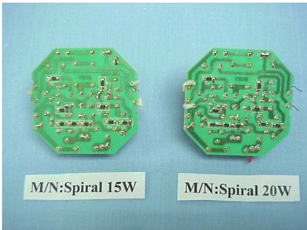
FIGURE 3 LIGHT(M/N: SPIRAL-15W, SPIRAL-20W) MAIN BOARD (SOLDERED SIDE)
