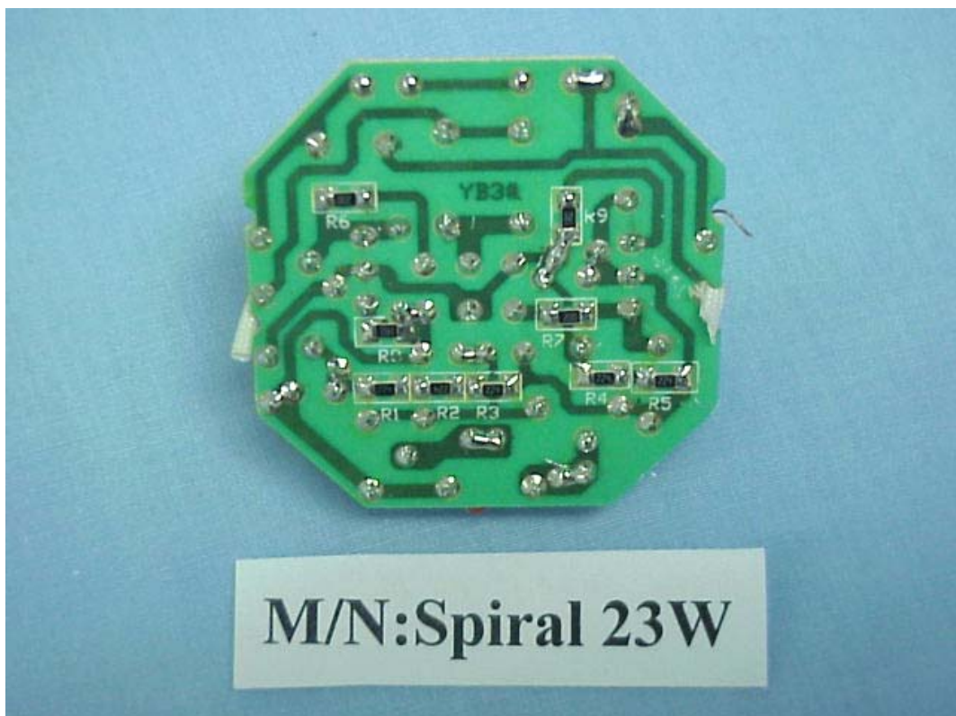
FIGURE 6 LIGHT(M/N: SPIRAL-23W) MAIN BOARD (SOLDERED SIDE)
