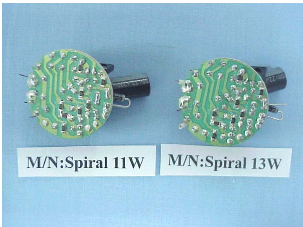
FIGURE 3 ENERGY SAVING LAMP (M/N: SPIRAL-11W, SPIRAL-13W) MAIN BOARD (SOLDERED SIDE)
