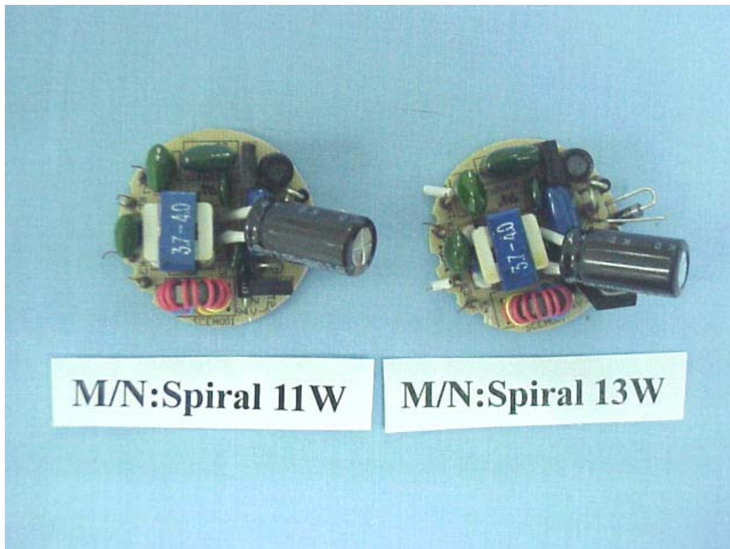
FIGURE 2 LIGHT (M/N: SPIRAL-11W, SPIRAL-13W) MAIN BOARD (COMPONENT SIDE)
