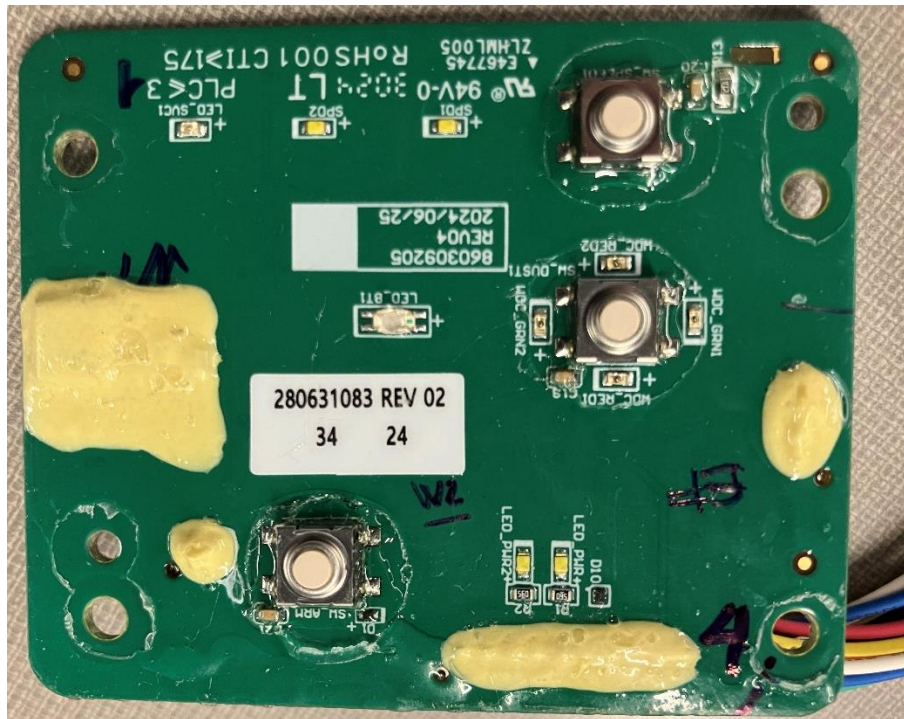
UI Board Top:
