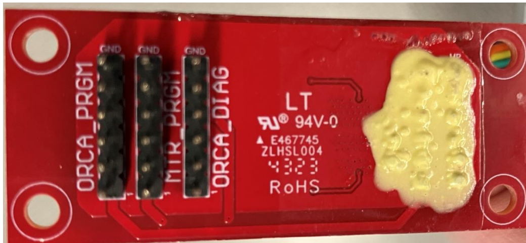
Interface Board Top:
