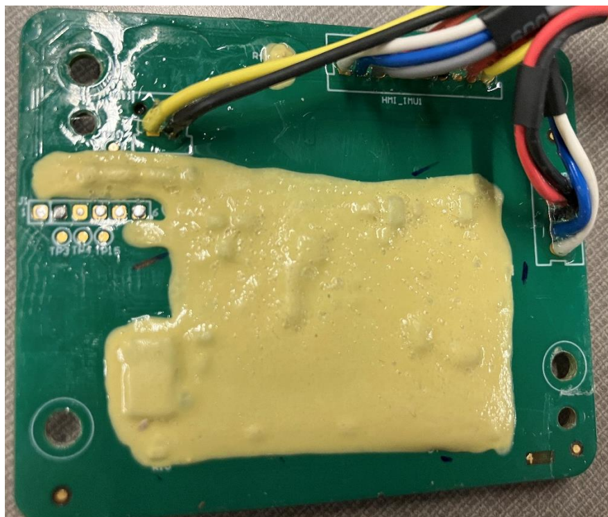
UI Board Bottom:
