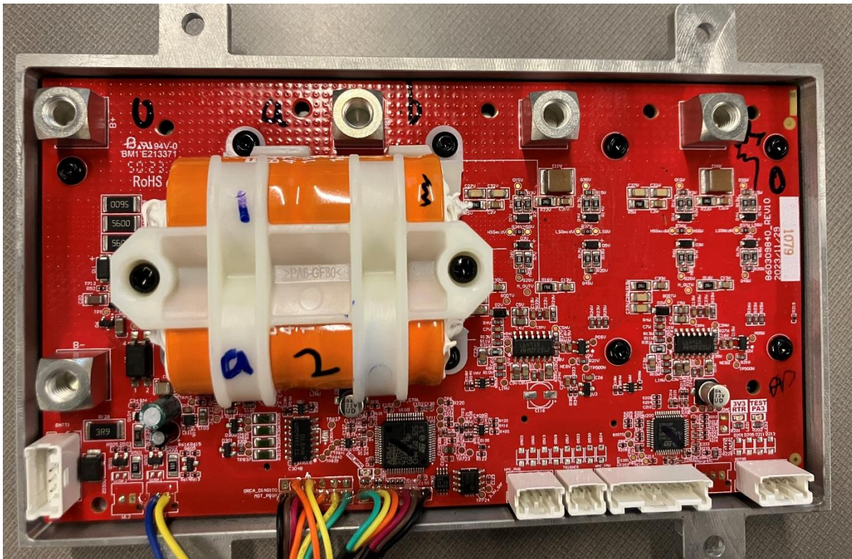
Control Board Top:
