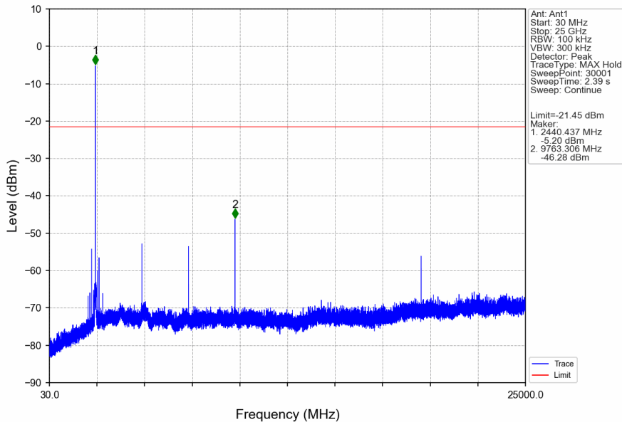
Pi/4DQPSK_2DH5_MCH_2441MHz_Ant1_NTNV
