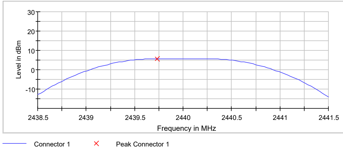
Peak Power
