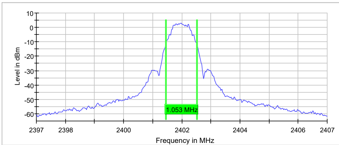
99 % Bandwidth
