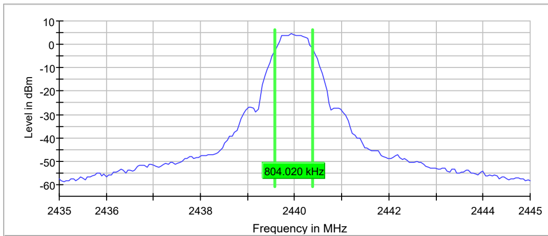
6 dB Bandwidth
