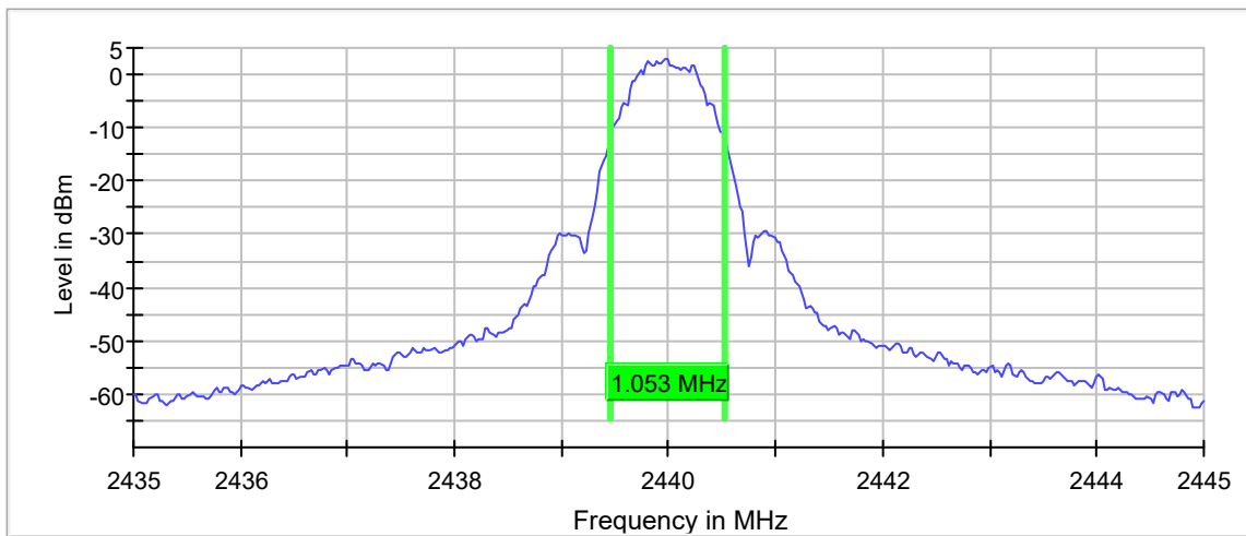
99 % Bandwidth
