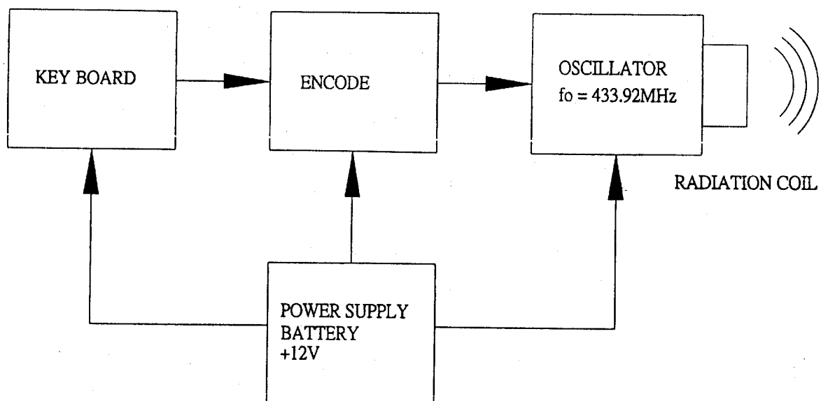
BLOCK DIAGRAM OF TRANSMITTER
