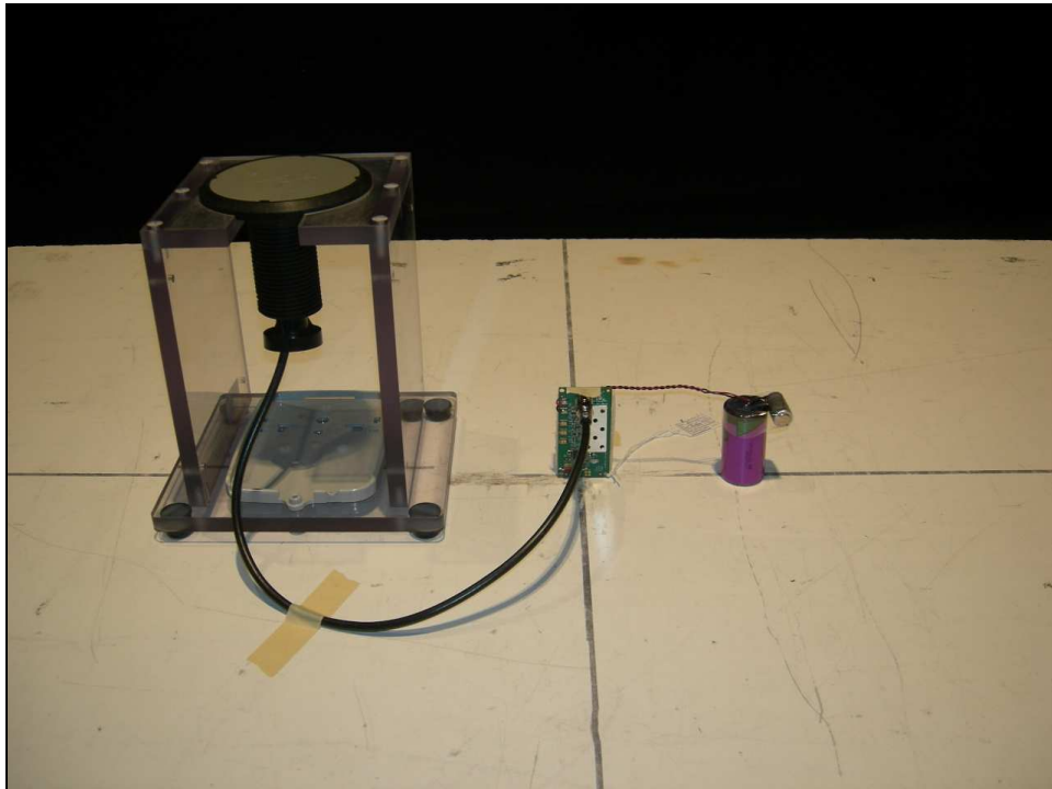
Figure 5: Radiated Emissions – External Antenna – ZPOS
