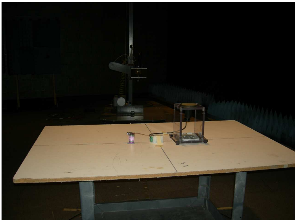
Figure 4: Radiated Emissions – External Antenna – YPOS
