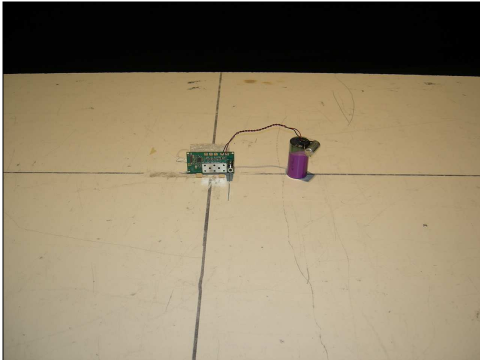
Figure 9: Radiated Emissions – Internal Antenna – YPOS
