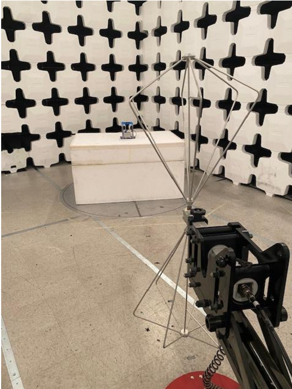
Figure 2. Radiated Emissions 30-1000 MHz
