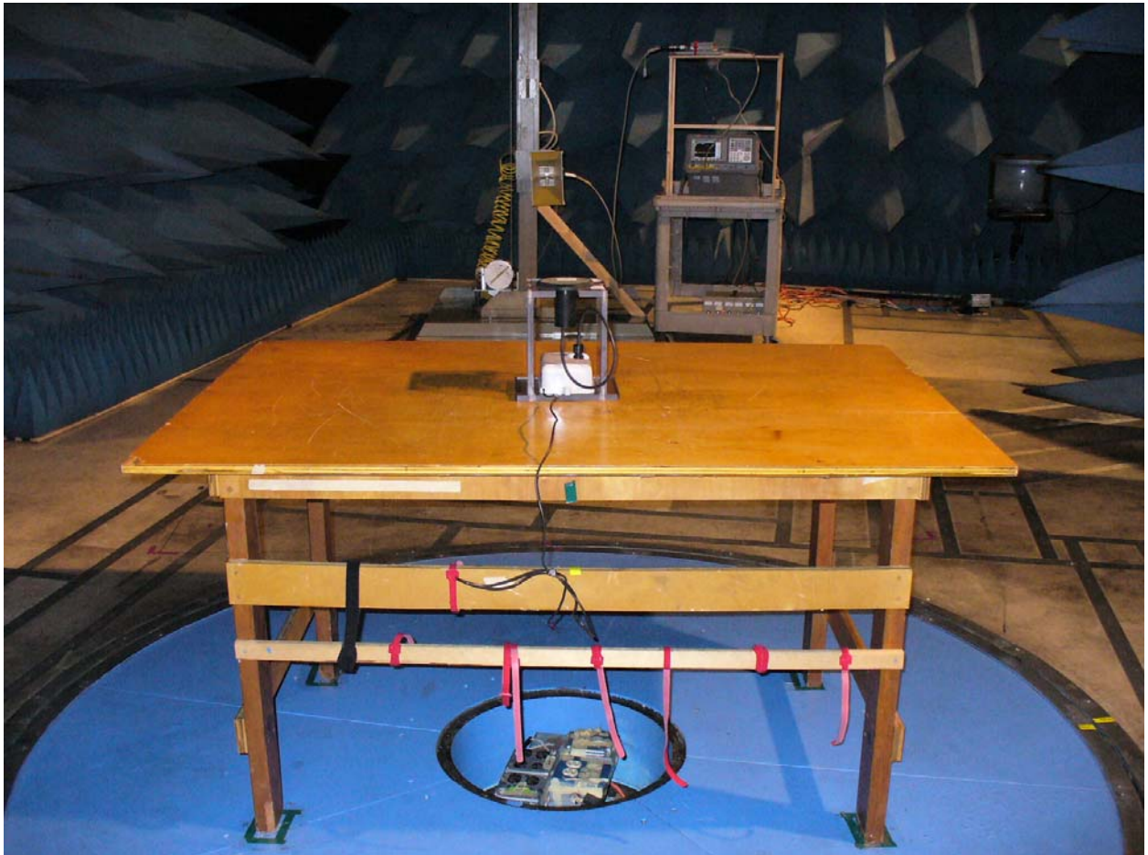
Figure 3: Radiated Emissions (External Antenna) – Back View
