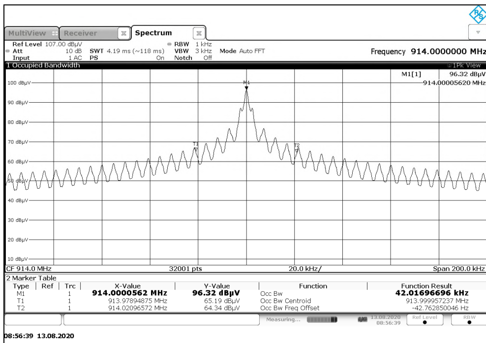
Figure 7.3.2-2: 99% Occupied Bandwidth Plot – 914MHz
