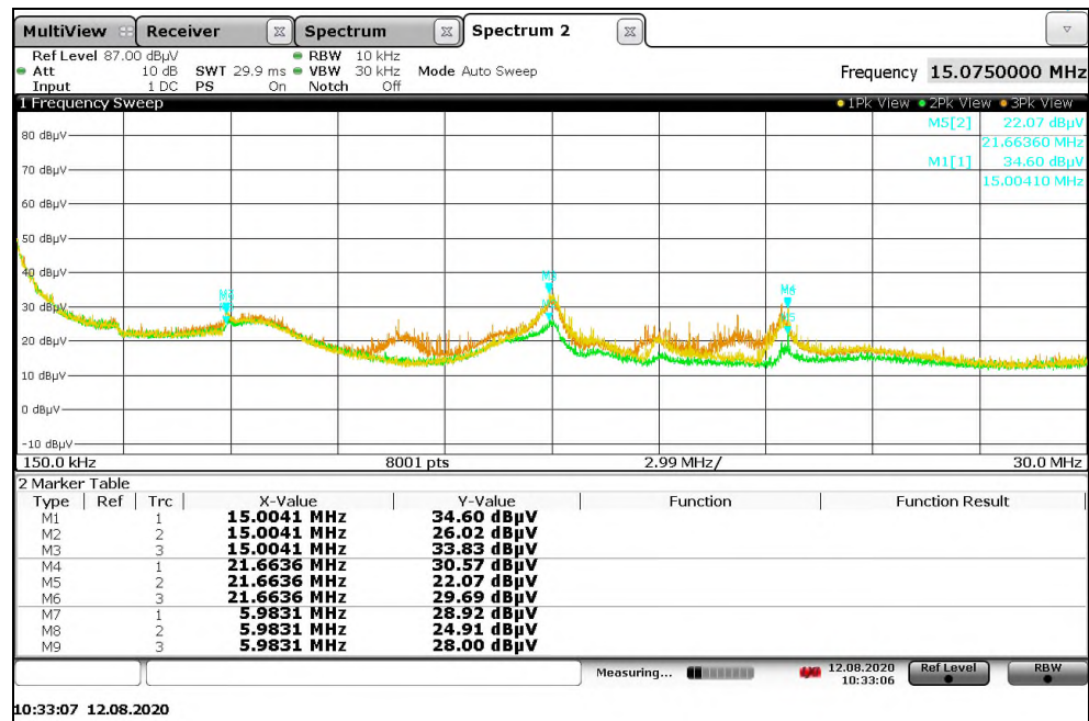
Figure A-2: Radiated Emissions – 150kHz-30MHz
