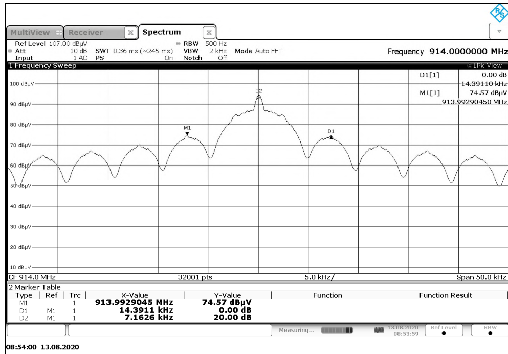
Figure 7.3.2-1: 20dB Emission Bandwidth Plot – 914MHz
