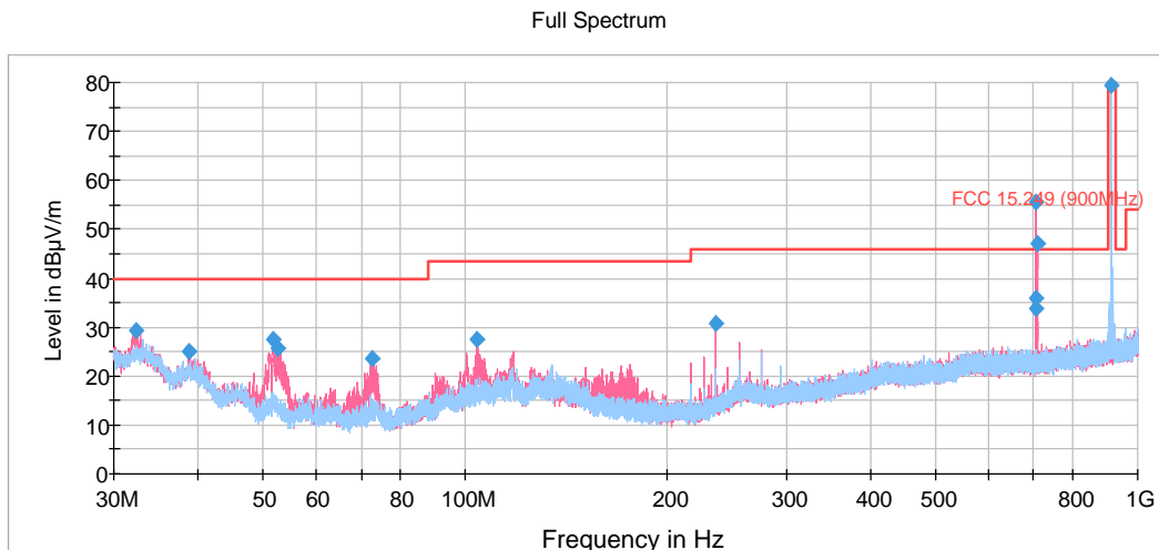
Figure A-3: Radiated Emissions – 30MHz-1GHz
