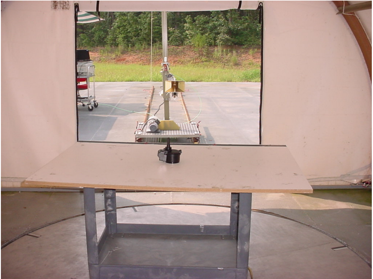
Figure 1: Test Setup – Monopole Antenna
