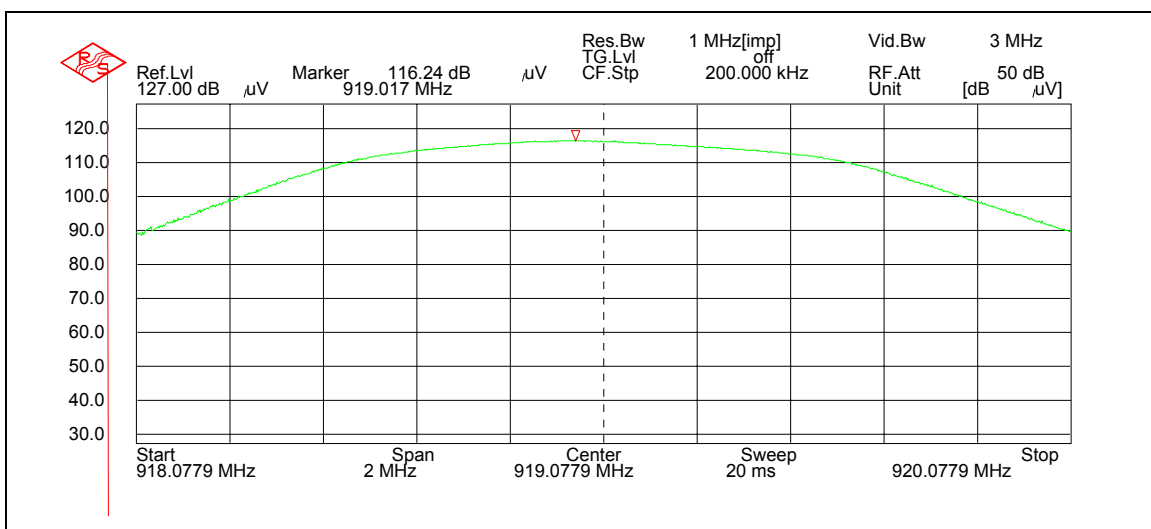
Figure 7.4-3: Output power – High Channel
