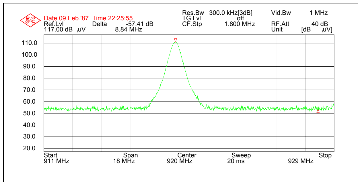
Figure 7.6.1-2: Upper Band-edge
