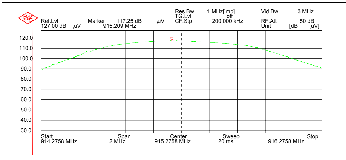
Figure 7.4-2: Output power – Mid Channel
