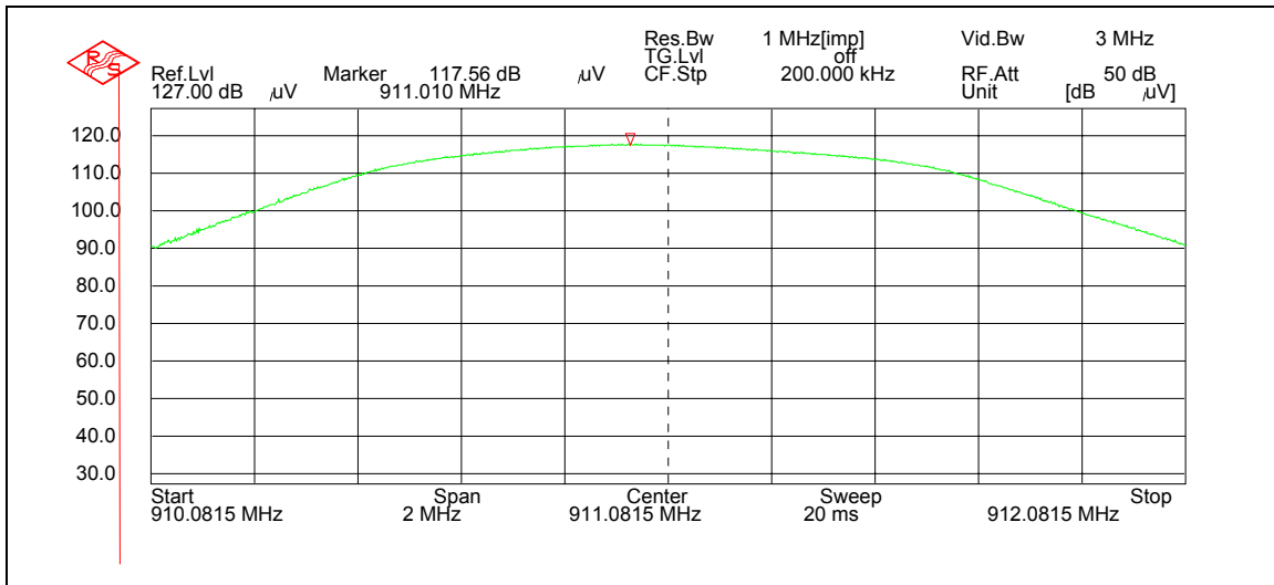
Figure 7.4-1: Output power – Low Channel
