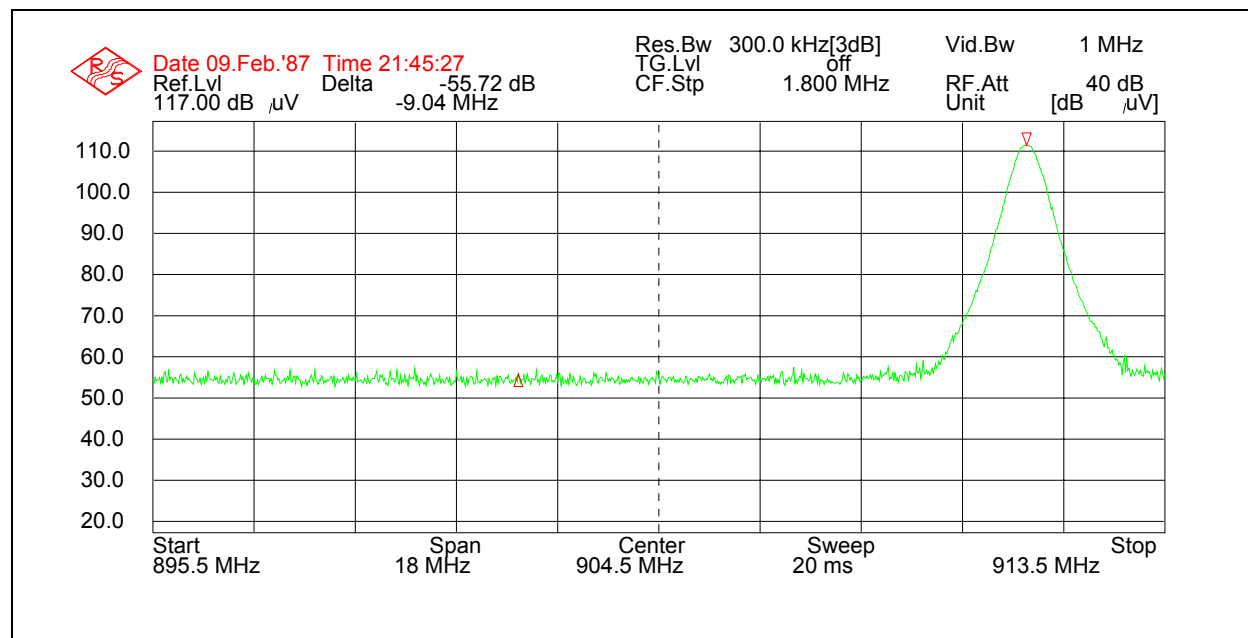
Figure 7.6.1-1: Lower Band-edge
