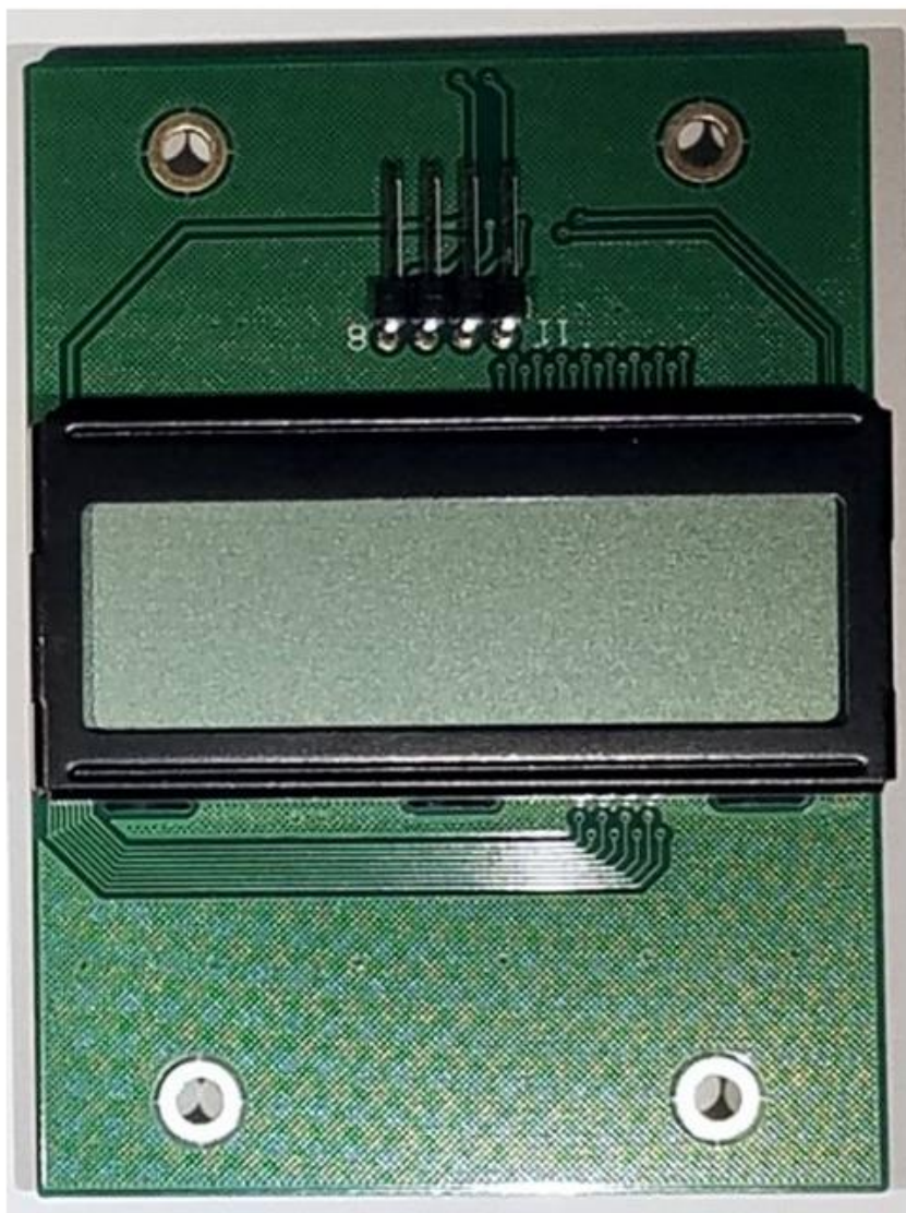
Figure 8. Top, Display Module Assembly
