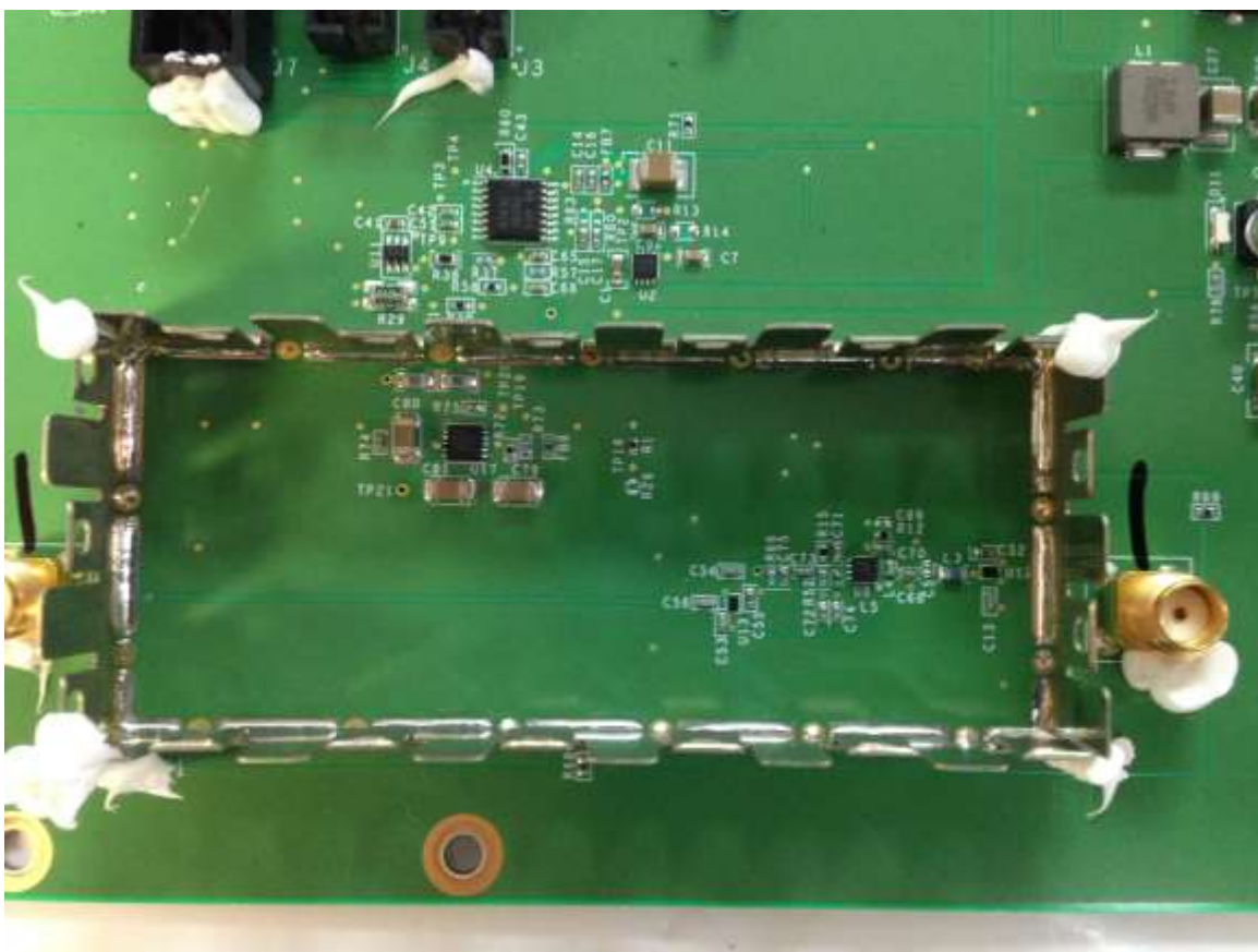
Figure 5. AIP Board, RF Circuit (Shield Removed)
