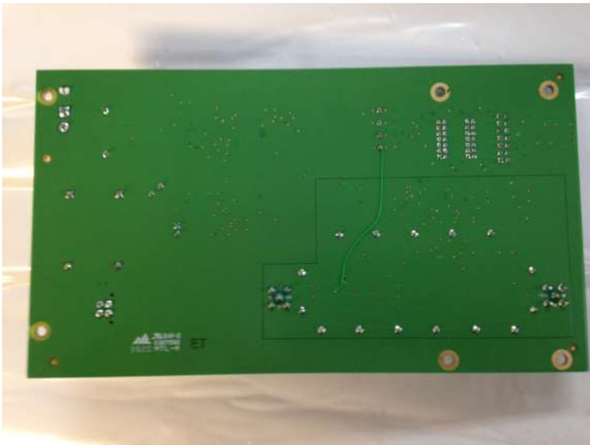
Figure 4. AIP Board Removed (Bottom View)
