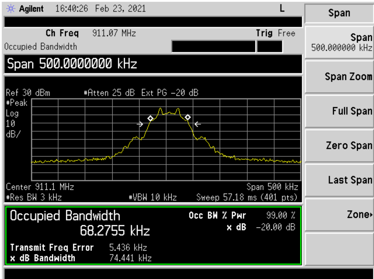
Figure 4. 20 dB and 99% Occupied Bandwidth – Low Channel (Worst Case Plot)
