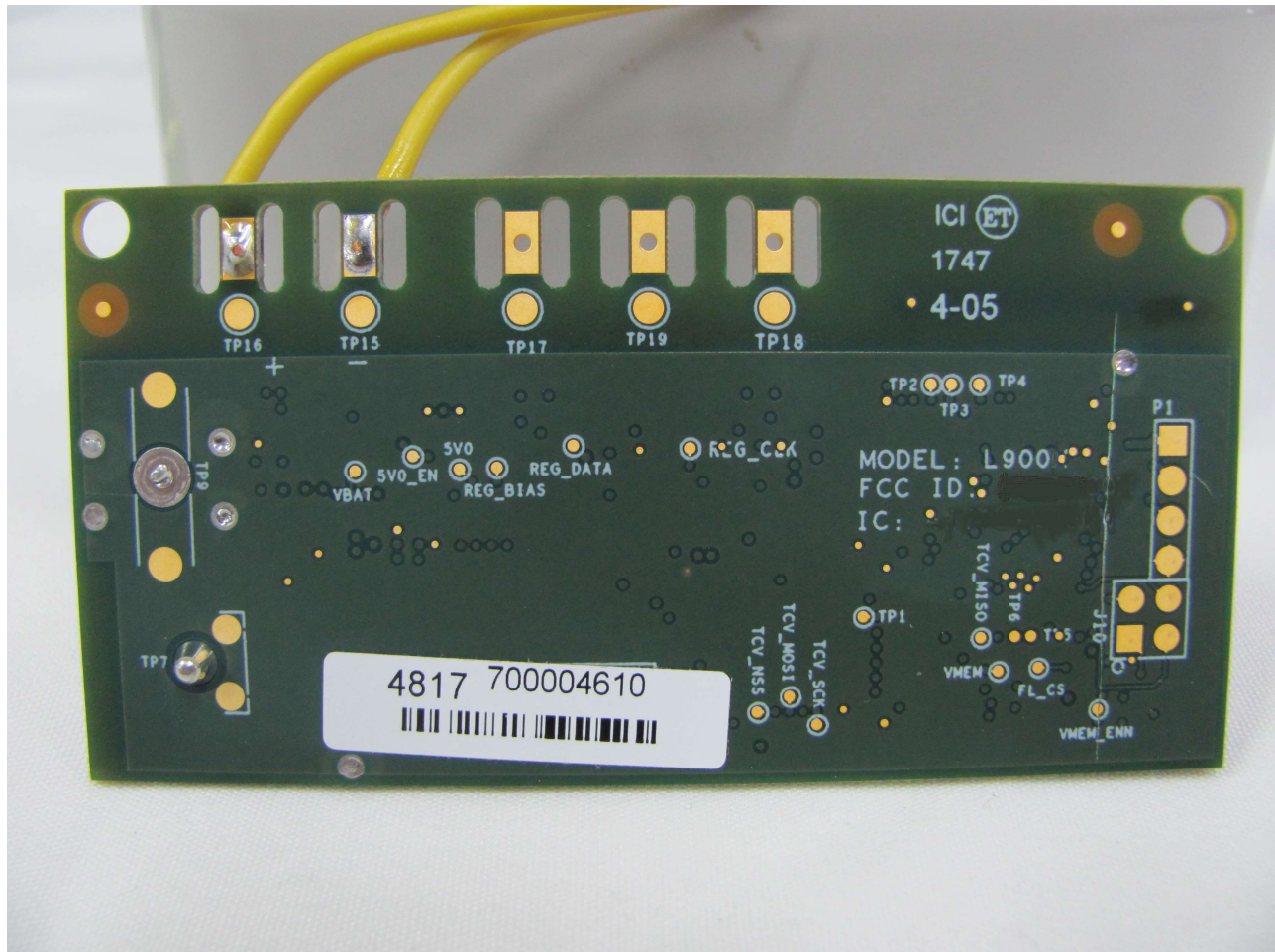
Figure 3. Bottom of Module
