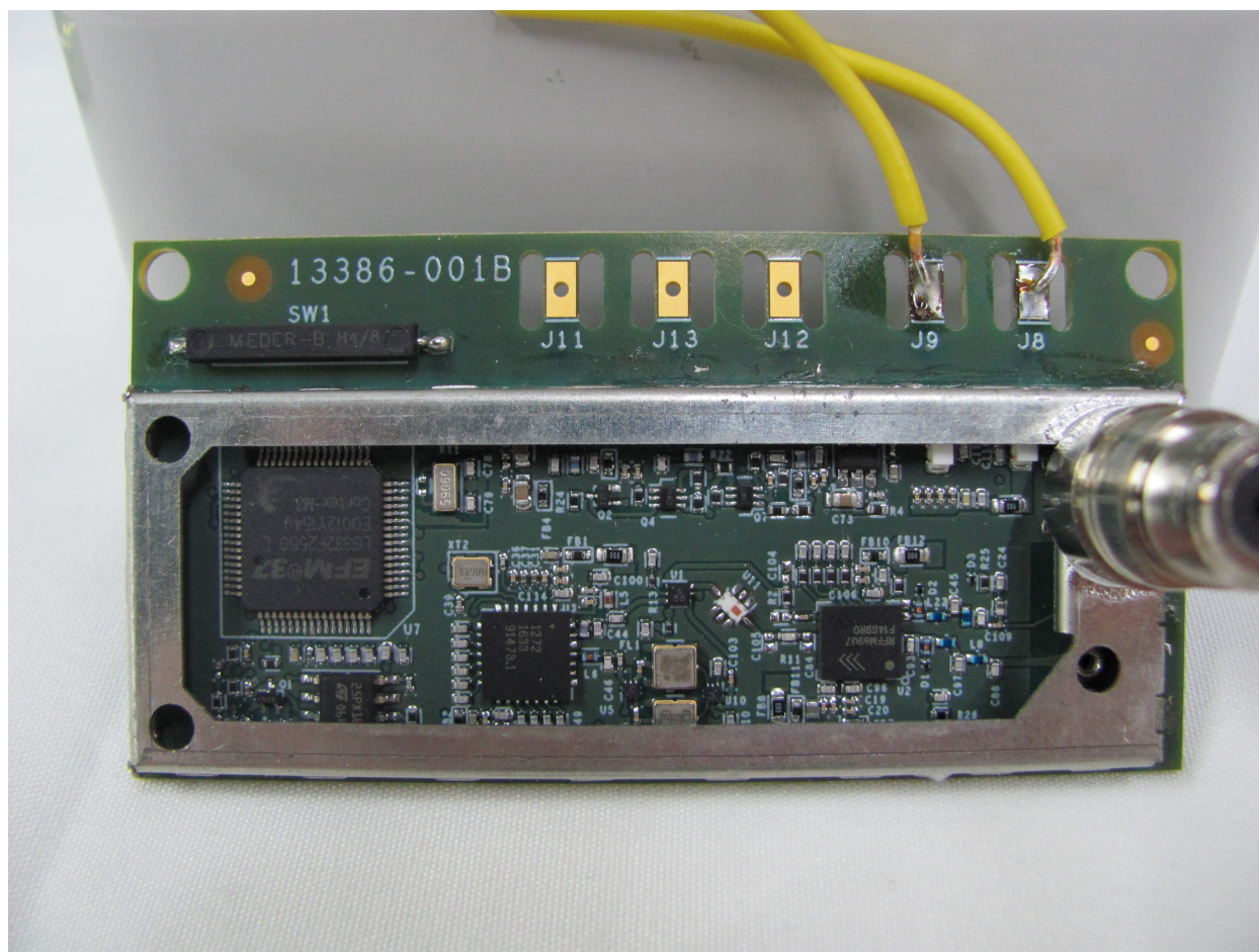
Figure 1. Top of Module, with Shield Removed
