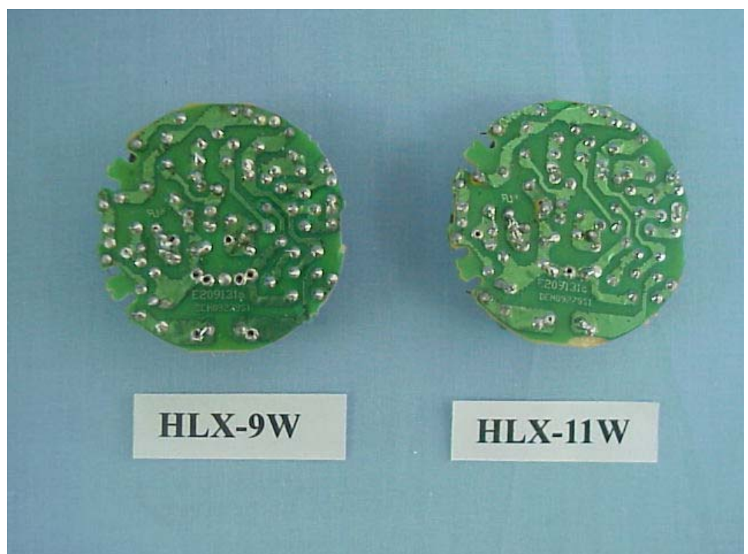
FIGURE 15 ENERGY SAVING LAMP (M/N: HLX-9W/11W) MAIN BOARD (SOLDERED SIDE)
