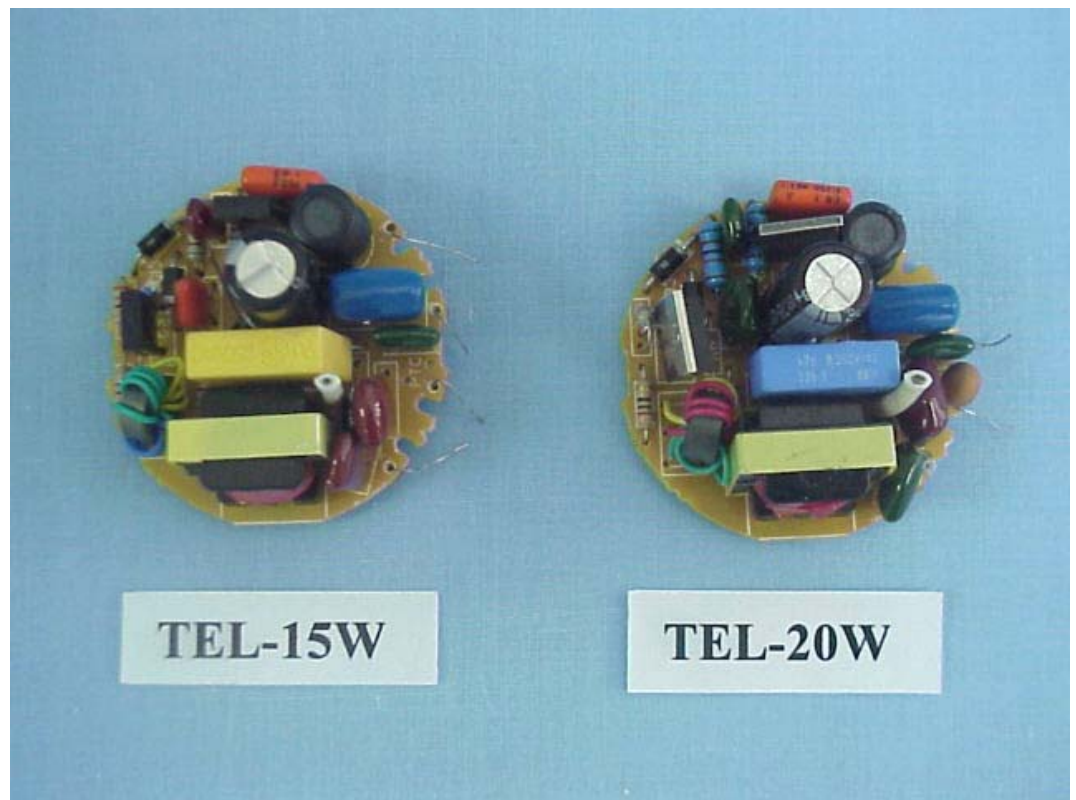
FIGURE 8 ENERGY SAVING LAMP (M/N: TEL-15W/20W) MAIN BOARD (COMPONENT SIDE)
