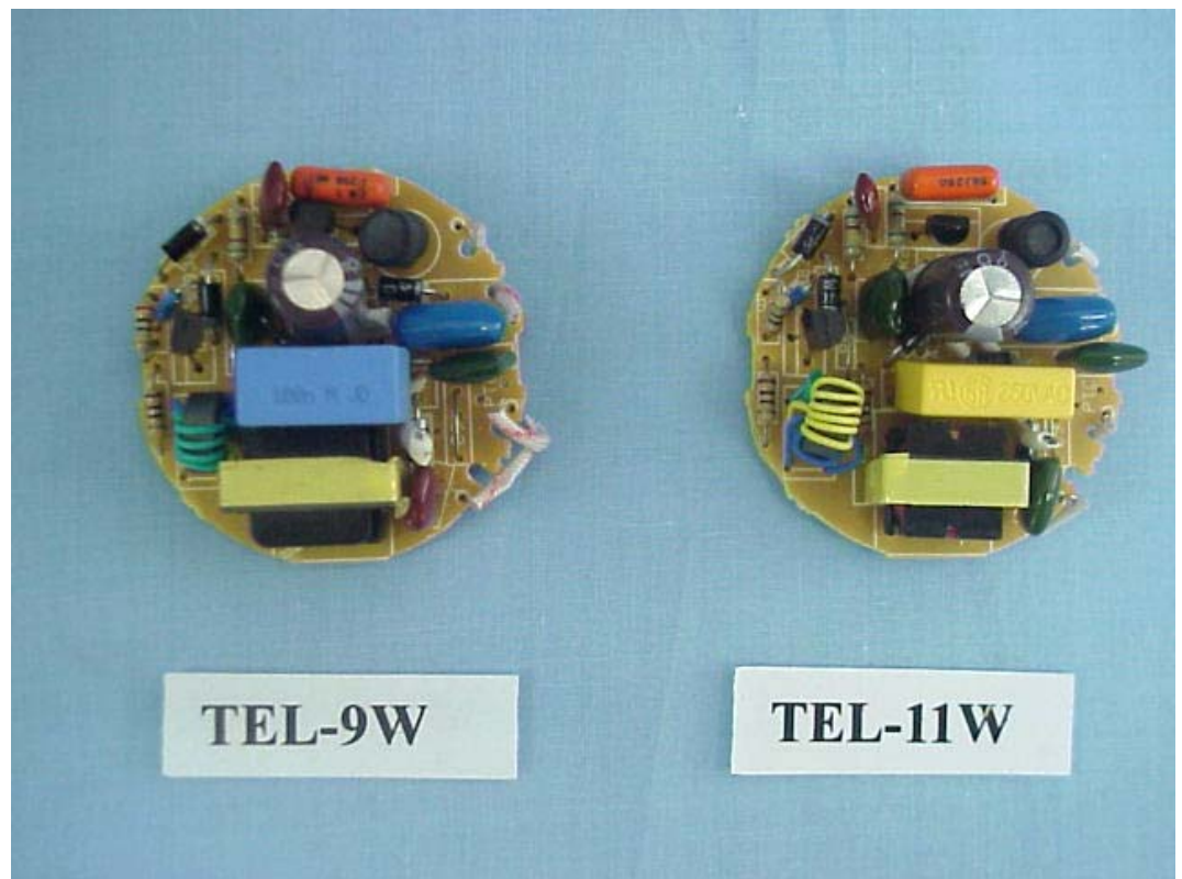
FIGURE 5 ENERGY SAVING LAMP (M/N: TEL-9W/11W) MAIN BOARD (COMPONENT SIDE)
