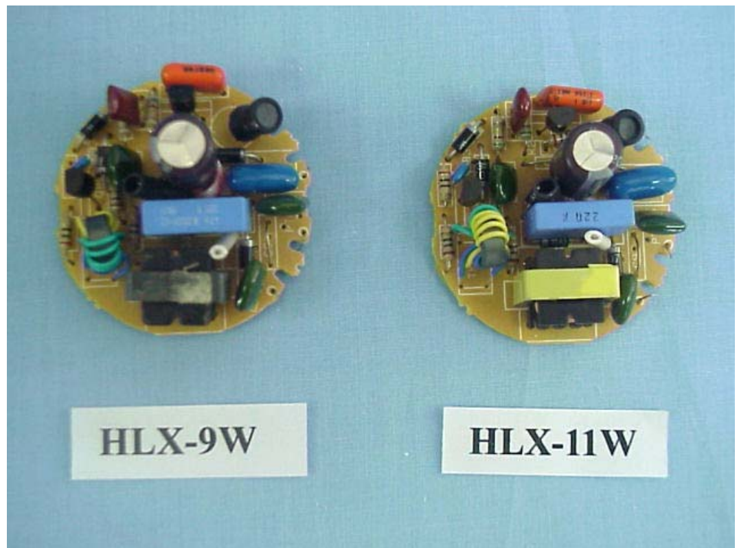
FIGURE 14 ENERGY SAVING LAMP (M/N: HLX-9W/11W) MAIN BOARD (COMPONENT SIDE)
