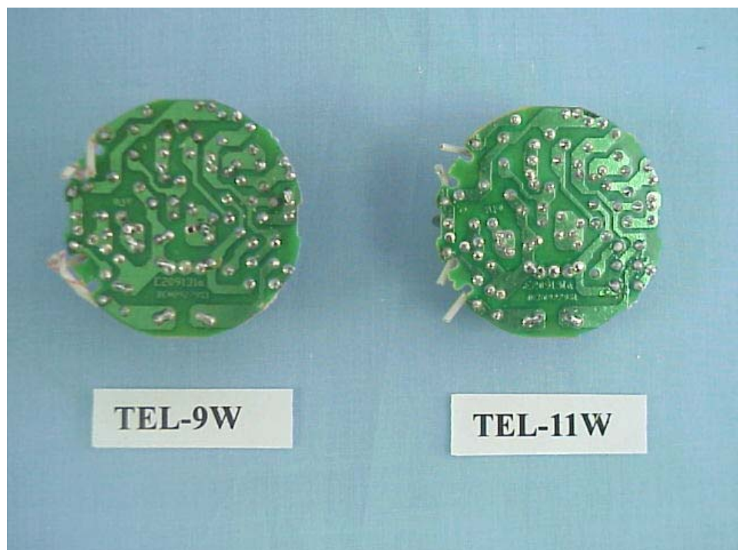
FIGURE 6 ENERGY SAVING LAMP (M/N: TEL-9W/11W) MAIN BOARD (SOLDERED SIDE)
