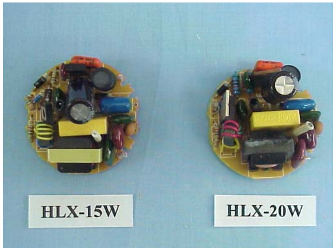
FIGURE 17 ENERGY SAVING LAMP (M/N: HLX-15W/20W) MAIN BOARD (COMPONENT SIDE)
