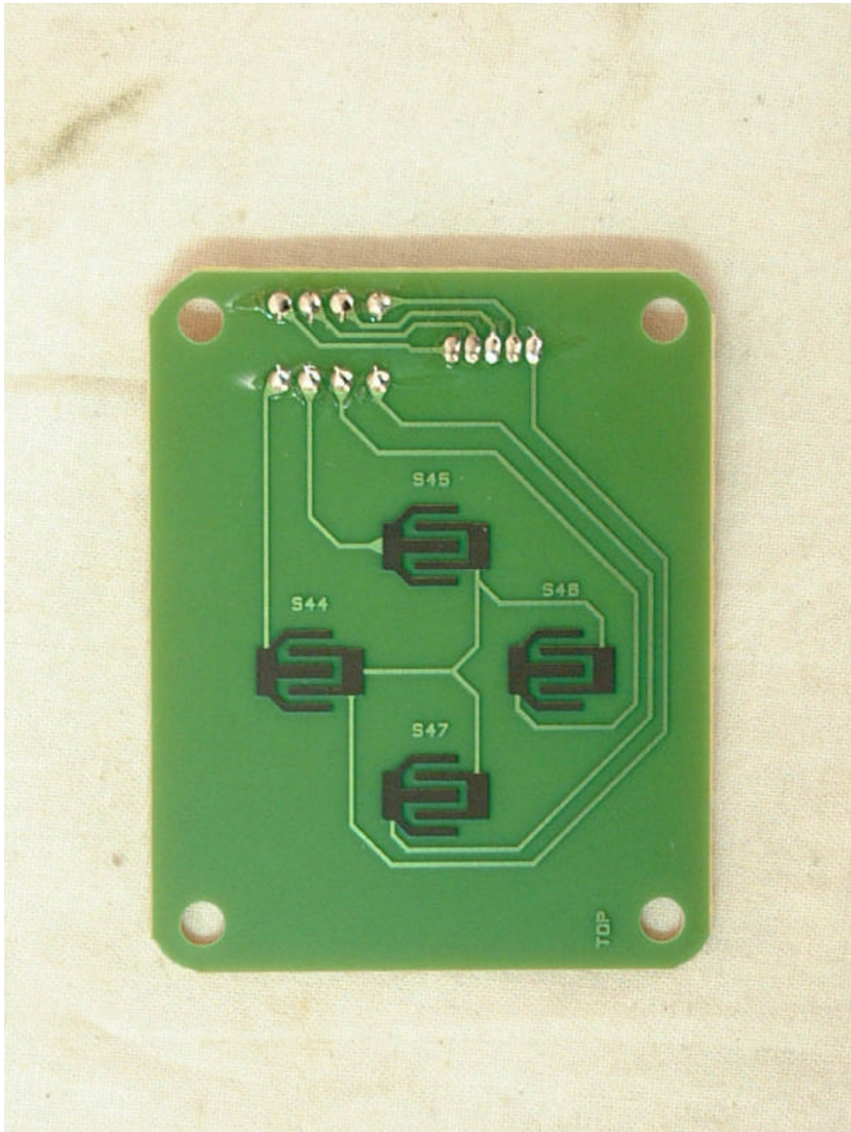
<REAR VIEW OF NAVIGATION BOARD >
