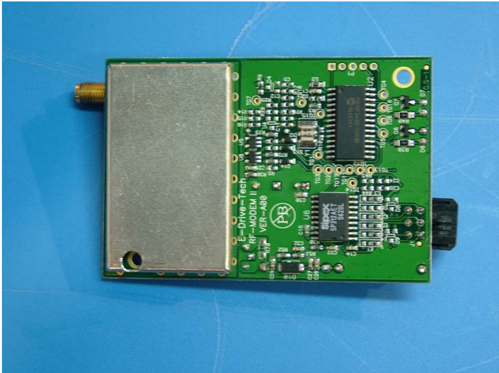
Bottom View, w/ RF Shielding
