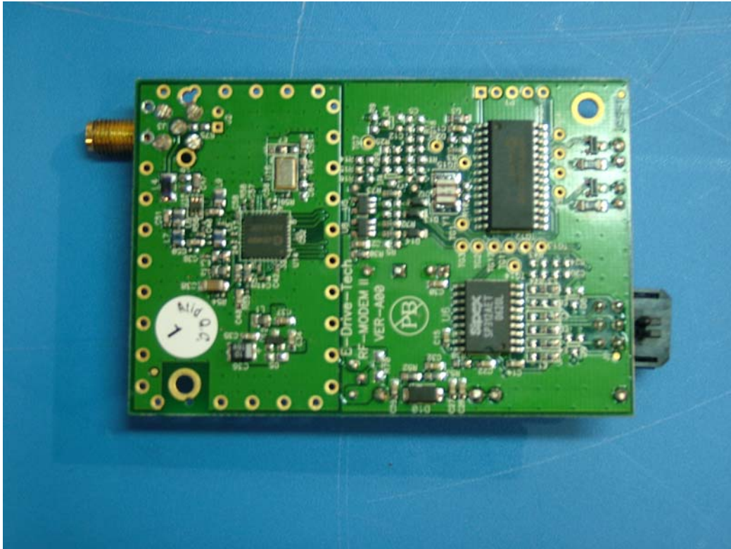
Bottom View, RF Shielding removed
