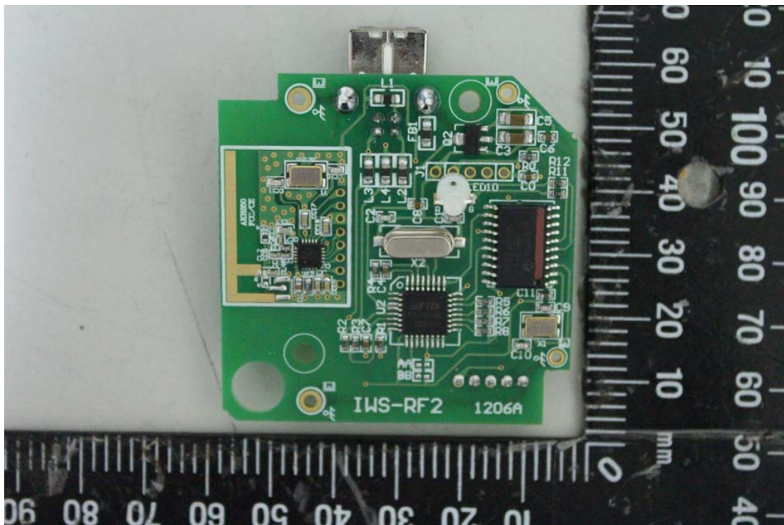
05 Front view of PCB
