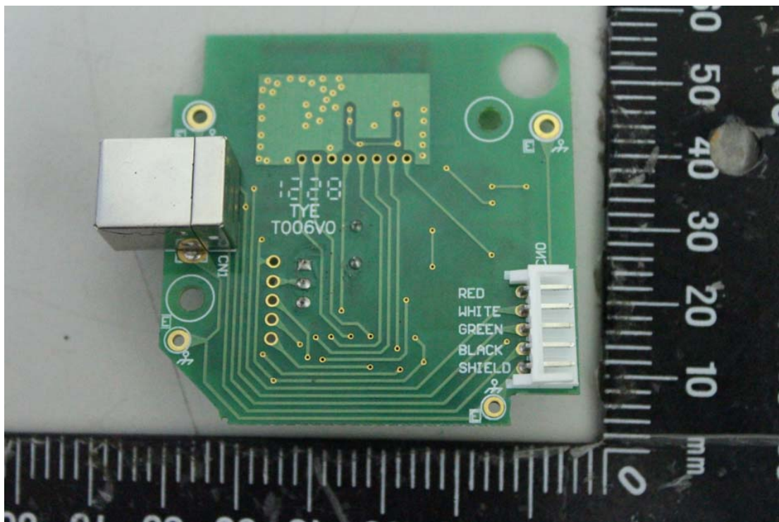
06 Rear view of PCB
