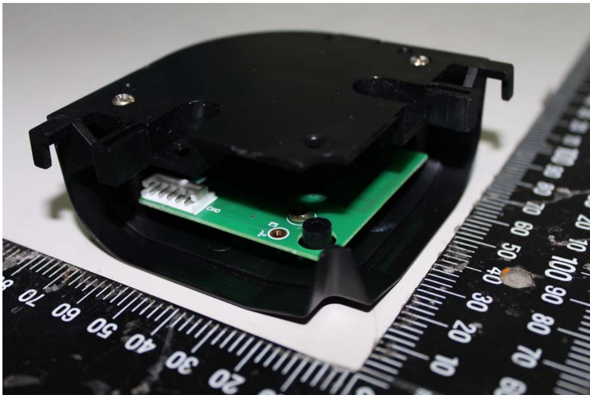
03 Rear view of EUT
