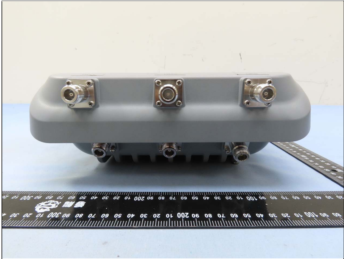
External Antenna
