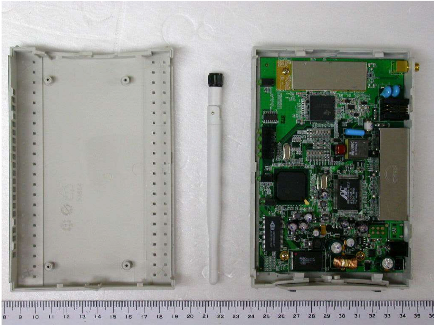
Reverse SMA connector, dipole antenna
