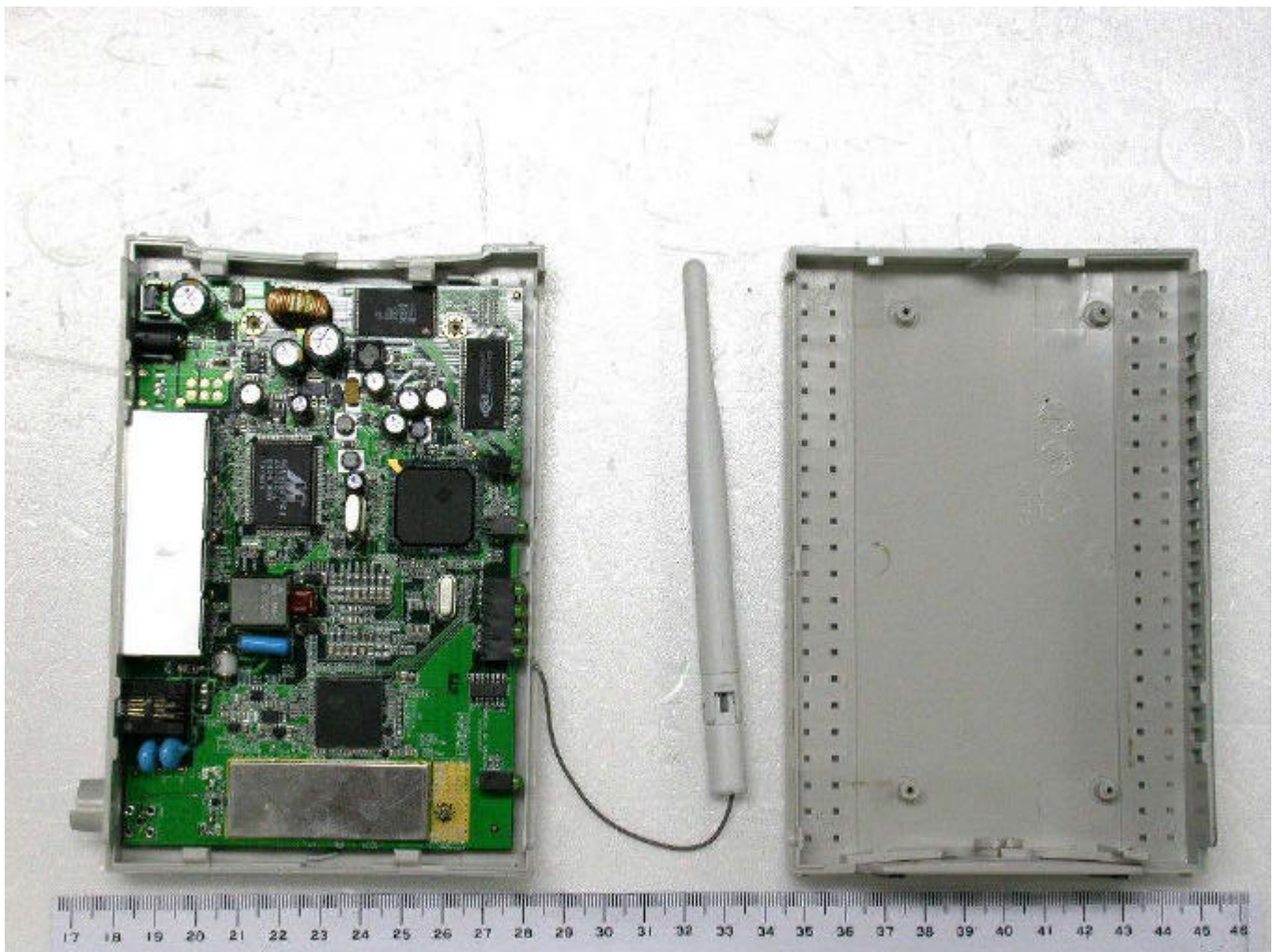
Integral dipole antenna
