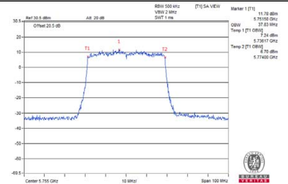
802.11ax (40MHz) / Chain 3 / CH 151
