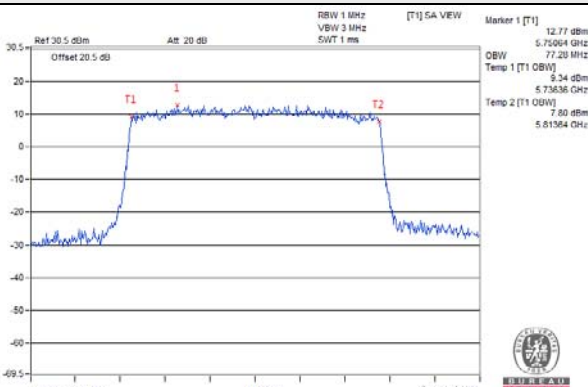
802.11ax (80MHz) / Chain 3 / CH 155
