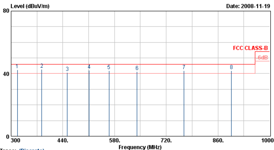
Trace: (Discrete)
