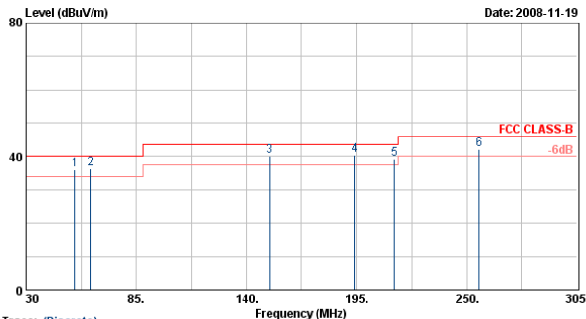
Trace: (Discrete)
