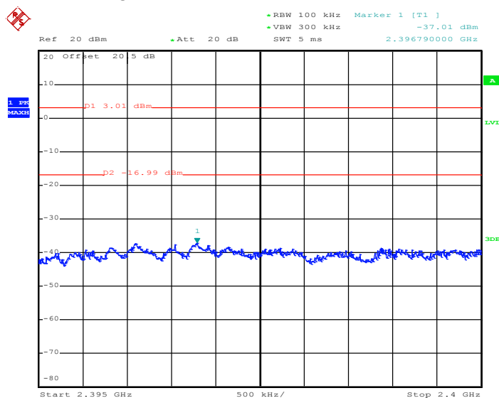
Low Band Edge Plot on 802.11b Channel 01- Chain A
