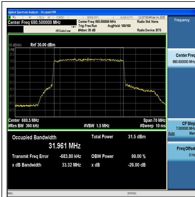
NTNV-n71-PC3-15-35-L-DFT-16QAM-Outer_Full-Ant1-PASS
