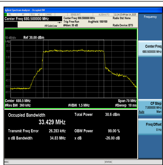
NTNV-n71-PC3-15-35-M-CP-16QAM-Outer_Full-Ant1-PASS
