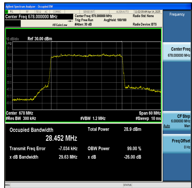
NTNV-n71-PC3-15-30-L-DFT-256QAM-Outer_Full-Ant1-PASS
