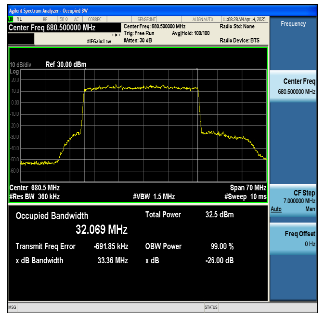
NTNV-n71-PC3-15-35-L-CP-QPSK-Outer_Full-Ant1-PASS
