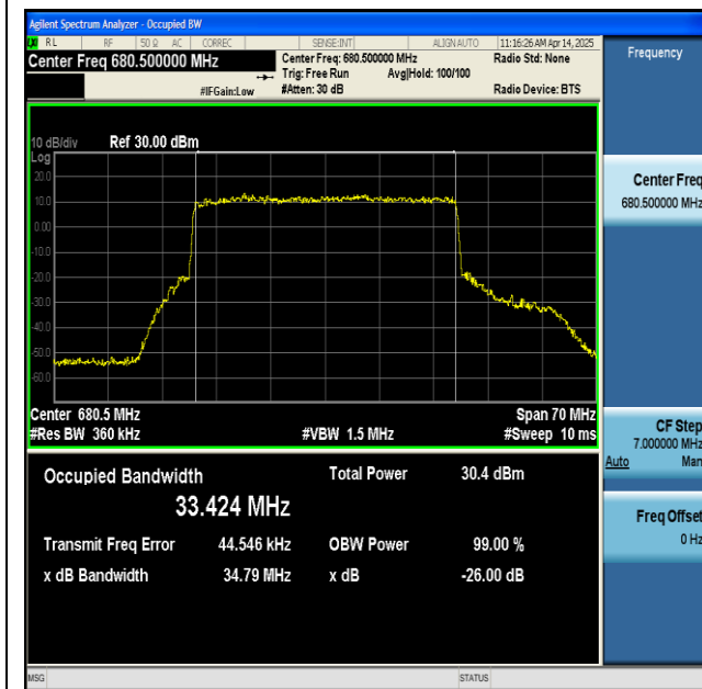
NTNV-n71-PC3-15-35-H-CP-16QAM-Outer_Full-Ant1-PASS
