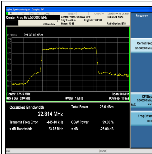
NTNV-n71-PC3-15-25-L-DFT-256QAM-Outer_Full-Ant1-PASS
