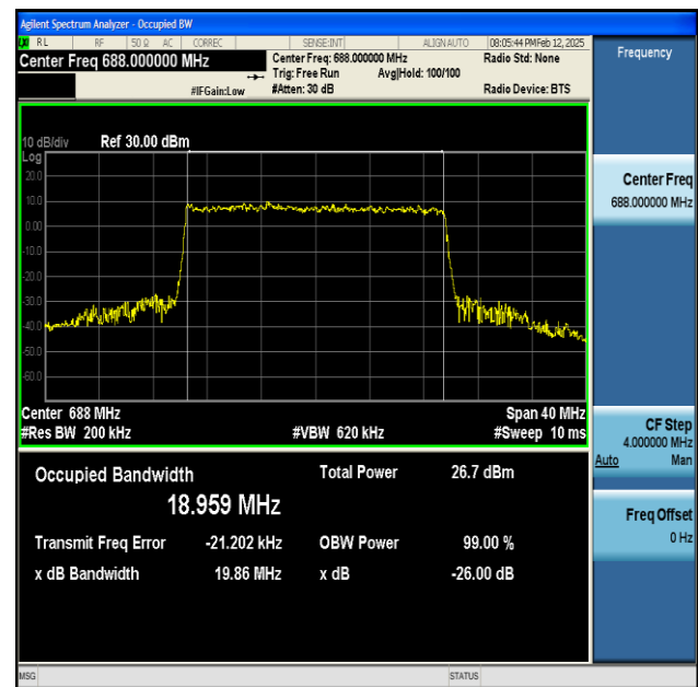
NTNV-n71-PC3-15-20-H-CP-256QAM-Outer_Full-Ant1-PASS
