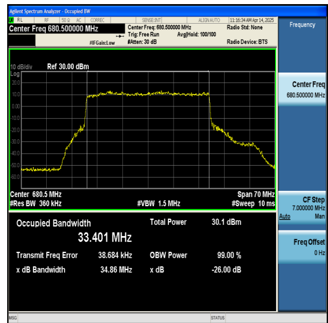
NTNV-n71-PC3-15-35-H-CP-64QAM-Outer_Full-Ant1-PASS
