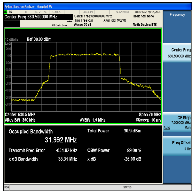
NTNV-n71-PC3-15-35-H-DFT-64QAM-Outer_Full-Ant1-PASS
