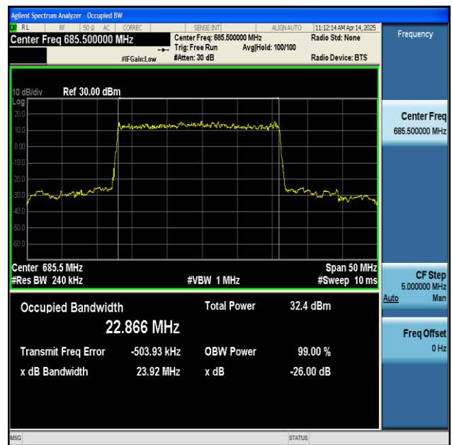
NTNV-n71-PC3-15-25-H-DFT-QPSK-Outer_Full-Ant1-PASS
