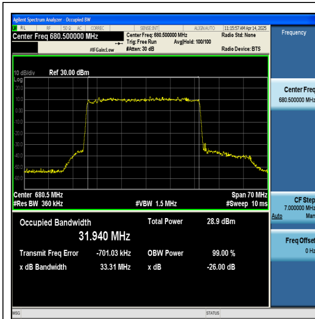
NTNV-n71-PC3-15-35-H-DFT-256QAM-Outer_Full-Ant1-PASS
