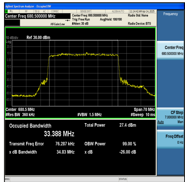
NTNV-n71-PC3-15-35-M-CP-256QAM-Outer_Full-Ant1-PASS
