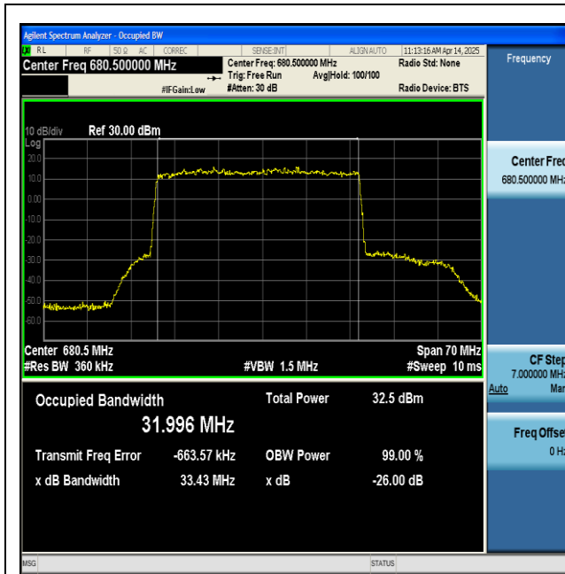
NTNV-n71-PC3-15-35-M-DFT-QPSK-Outer_Full-Ant1-PASS
