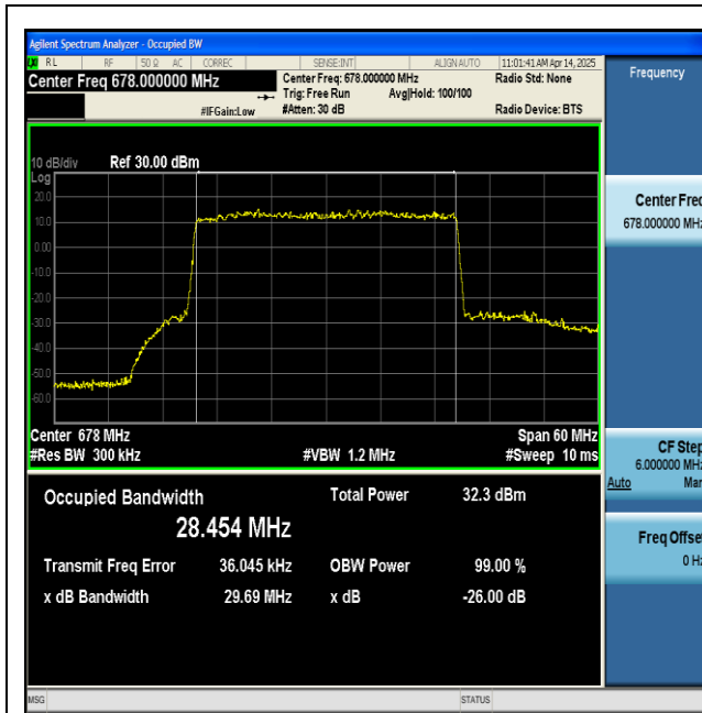
NTNV-n71-PC3-15-30-L-DFT-QPSK-Outer_Full-Ant1-PASS
