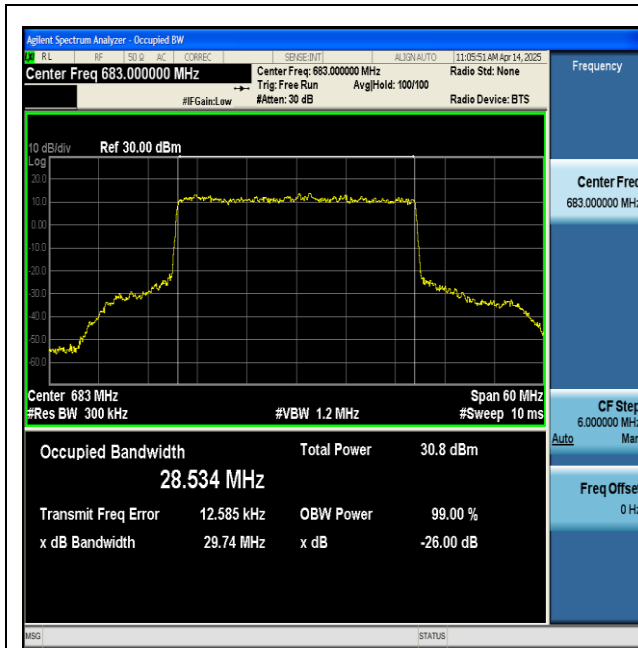
NTNV-n71-PC3-15-30-H-DFT-64QAM-Outer_Full-Ant1-PASS
