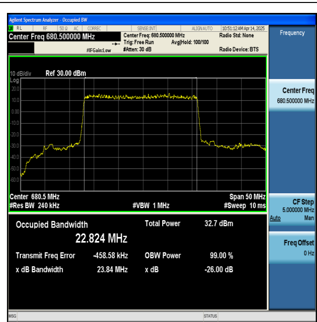
NTNV-n71-PC3-15-25-M-DFT-BPSK-Outer_Full-Ant1-PASS
