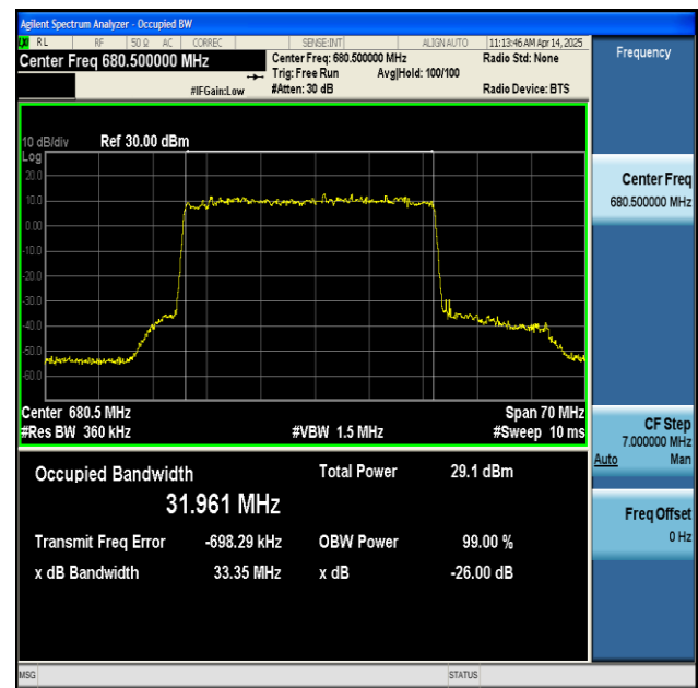
NTNV-n71-PC3-15-35-M-DFT-256QAM-Outer_Full-Ant1-PASS
