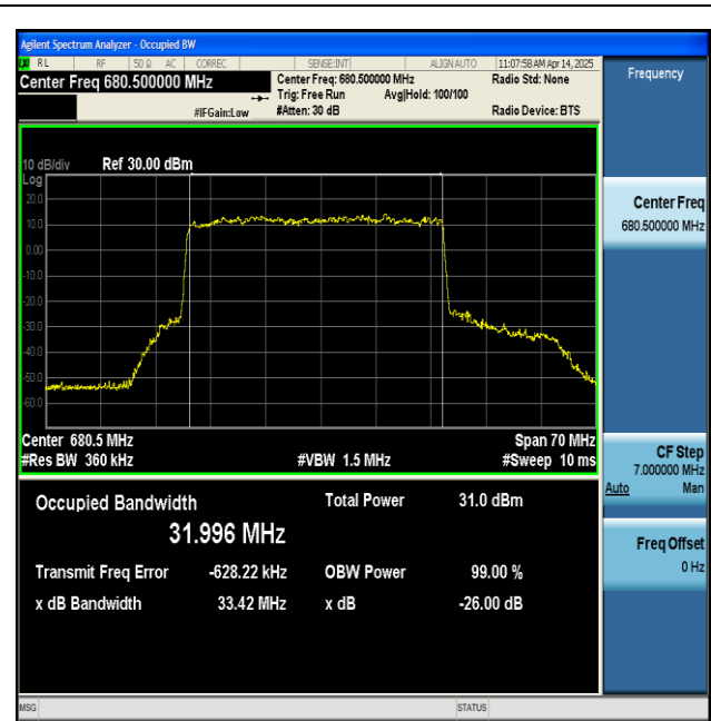
NTNV-n71-PC3-15-35-L-DFT-64QAM-Outer_Full-Ant1-PASS
