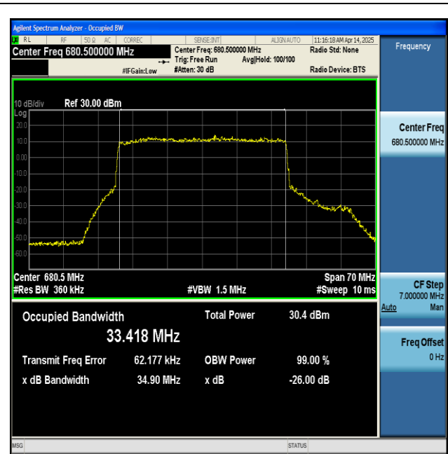
NTNV-n71-PC3-15-35-H-CP-QPSK-Outer_Full-Ant1-PASS
