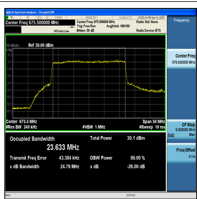
NTNV-n71-PC3-15-25-L-CP-QPSK-Outer_Full-Ant1-PASS
