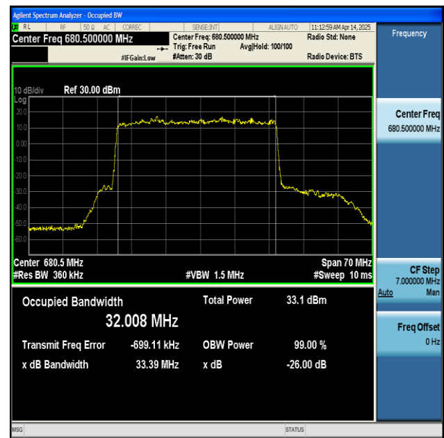
NTNV-n71-PC3-15-35-M-DFT-BPSK-Outer_Full-Ant1-PASS
