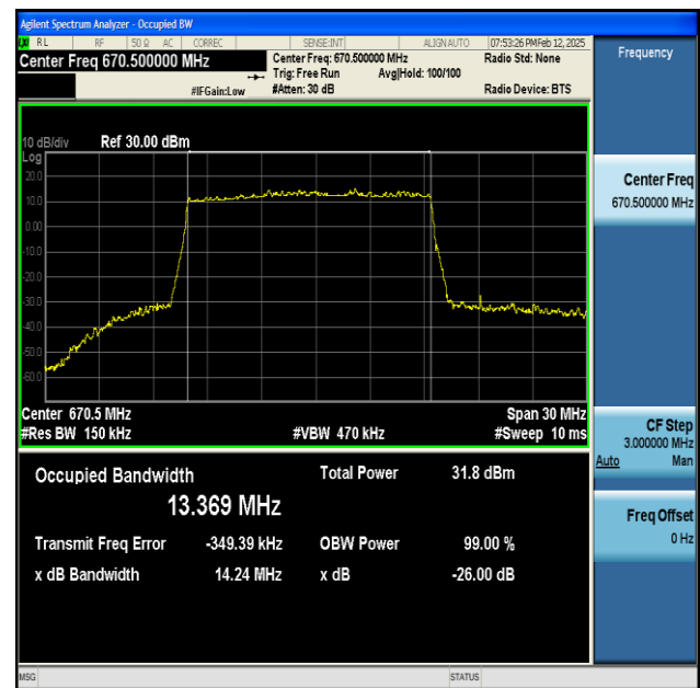
NTNV-n71-PC3-15-15-L-DFT-QPSK-Outer_Full-Ant1-PASS
