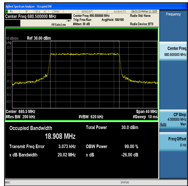
NTNV-n71-PC3-15-20-M-CP-QPSK-Outer_Full-Ant1-PASS
