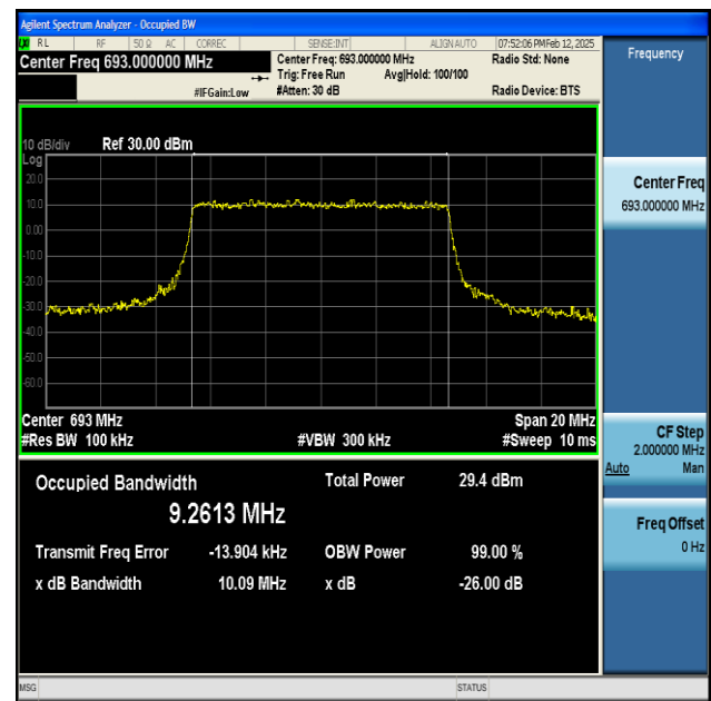
NTNV-n71-PC3-15-10-H-CP-16QAM-Outer_Full-Ant1-PASS
