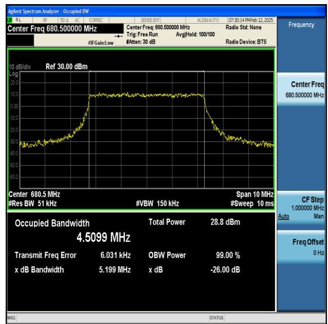
NTNV-n71-PC3-15-5-M-CP-16QAM-Outer_Full-Ant1-PASS
