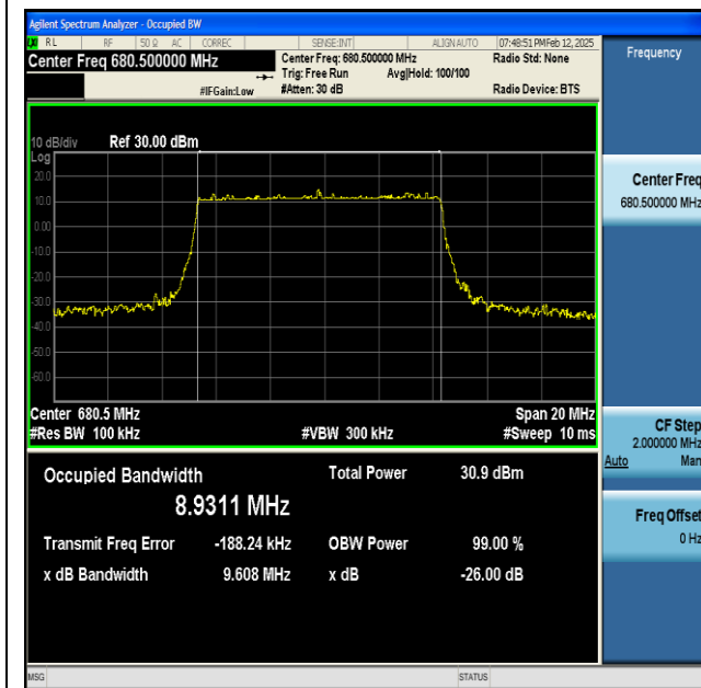
NTNV-n71-PC3-15-10-M-DFT-16QAM-Outer_Full-Ant1-PASS
