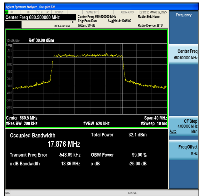
NTNV-n71-PC3-15-20-M-DFT-QPSK-Outer_Full-Ant1-PASS
