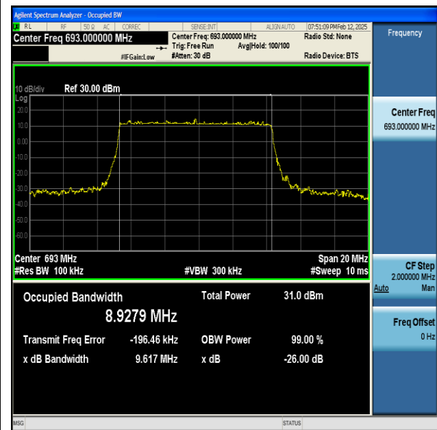
NTNV-n71-PC3-15-10-H-DFT-16QAM-Outer_Full-Ant1-PASS
