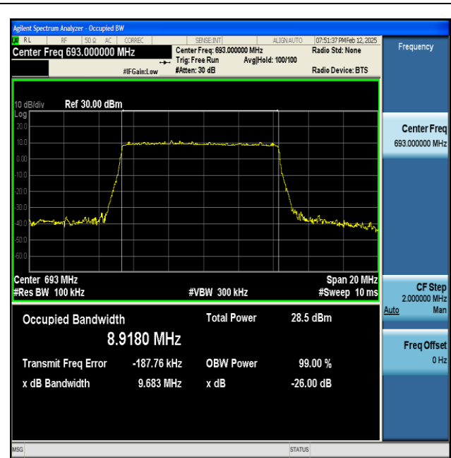
NTNV-n71-PC3-15-10-H-DFT-256QAM-Outer_Full-Ant1-PASS
