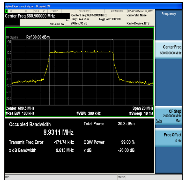
NTNV-n71-PC3-15-10-M-DFT-64QAM-Outer_Full-Ant1-PASS
