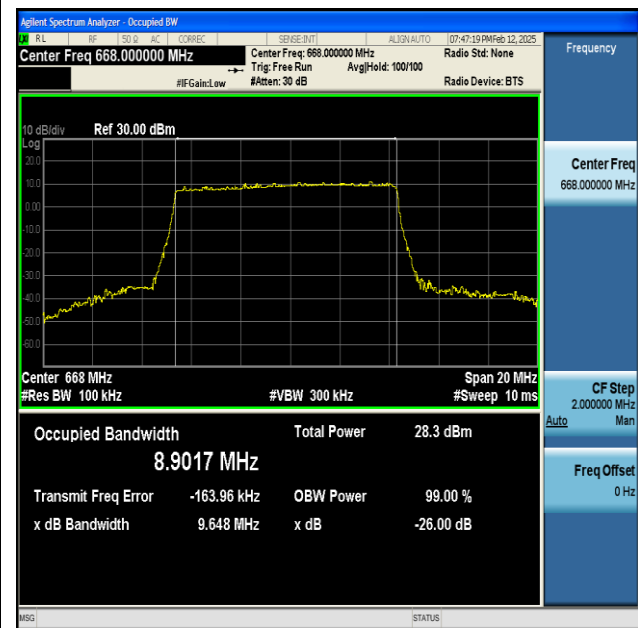
NTNV-n71-PC3-15-10-L-DFT-256QAM-Outer_Full-Ant1-PASS
