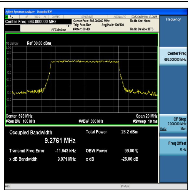
NTNV-n71-PC3-15-10-H-CP-256QAM-Outer_Full-Ant1-PASS
