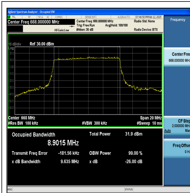
NTNV-n71-PC3-15-10-L-DFT-QPSK-Outer_Full-Ant1-PASS
