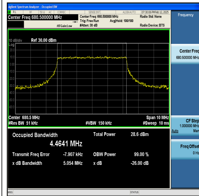
NTNV-n71-PC3-15-5-M-CP-QPSK-Outer_Full-Ant1-PASS
