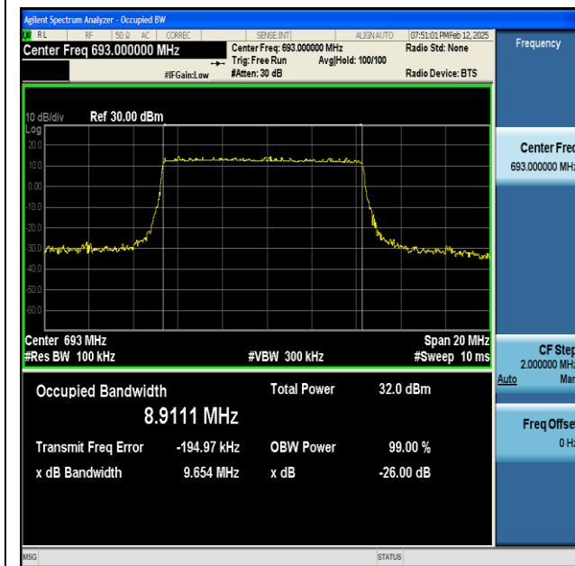
NTNV-n71-PC3-15-10-H-DFT-QPSK-Outer_Full-Ant1-PASS
