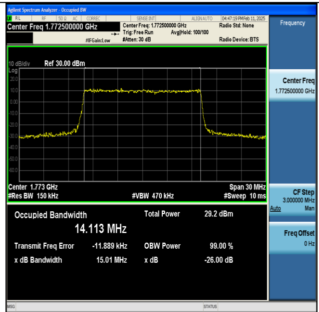
NTNV-n66-PC3-15-15-H-CP-QPSK-Outer_Full-Ant1-PASS
