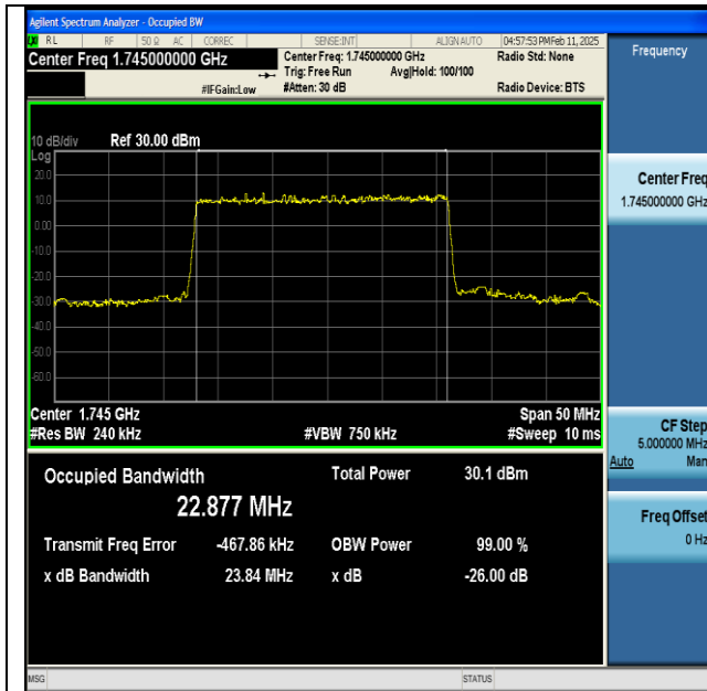
NTNV-n66-PC3-15-25-M-DFT-64QAM-Outer_Full-Ant1- PASS
