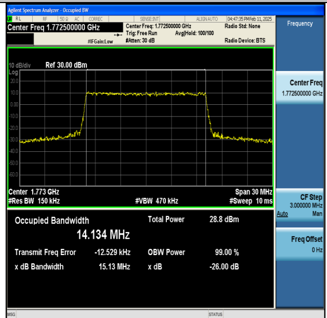
NTNV-n66-PC3-15-15-H-CP-64QAM-Outer_Full-Ant1-PASS
