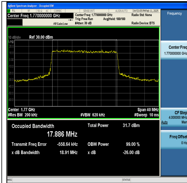
NTNV-n66-PC3-15-20-H-DFT-QPSK-Outer_Full-Ant1- PASS
