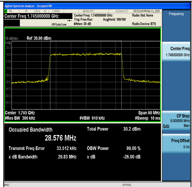
NTNV-n66-PC3-15-30-M-DFT-64QAM-Outer_Full-Ant1- PASS
