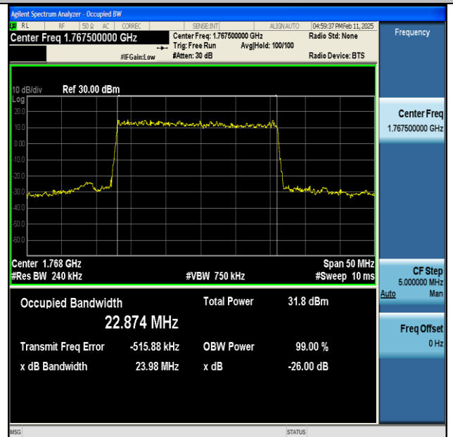
NTNV-n66-PC3-15-25-H-DFT-QPSK-Outer_Full-Ant1- PASS
