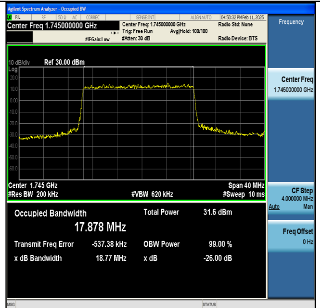
NTNV-n66-PC3-15-20-M-DFT-QPSK-Outer_Full-Ant1- PASS
