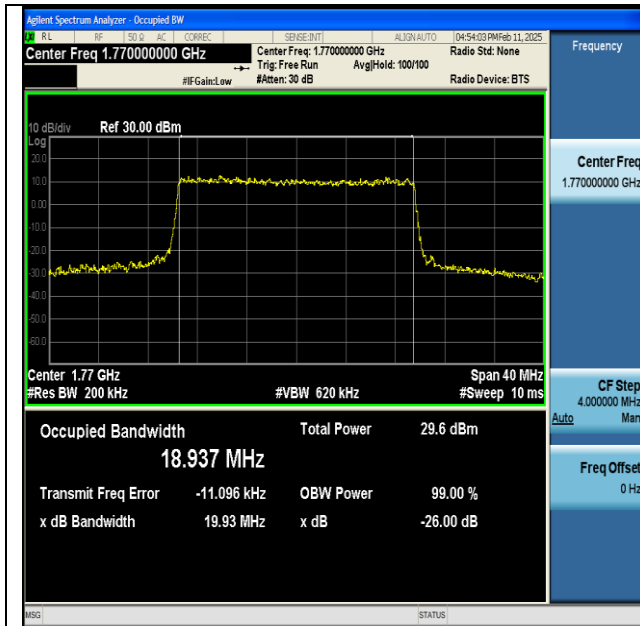
NTNV-n66-PC3-15-20-H-CP-QPSK-Outer_Full-Ant1-PASS
