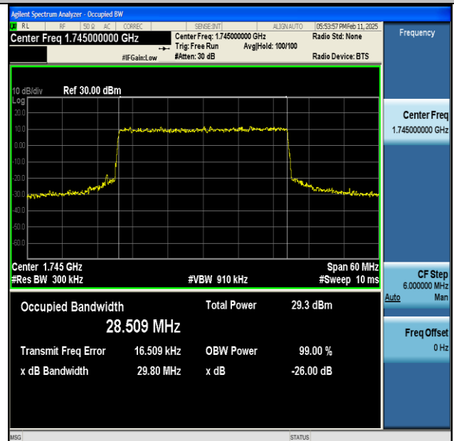
NTNV-n66-PC3-15-30-M-CP-64QAM-Outer_Full-Ant1-PASS
