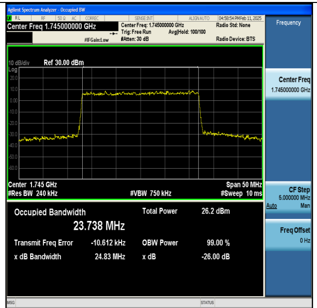
NTNV-n66-PC3-15-25-M-CP-256QAM-Outer_Full-Ant1- PASS
