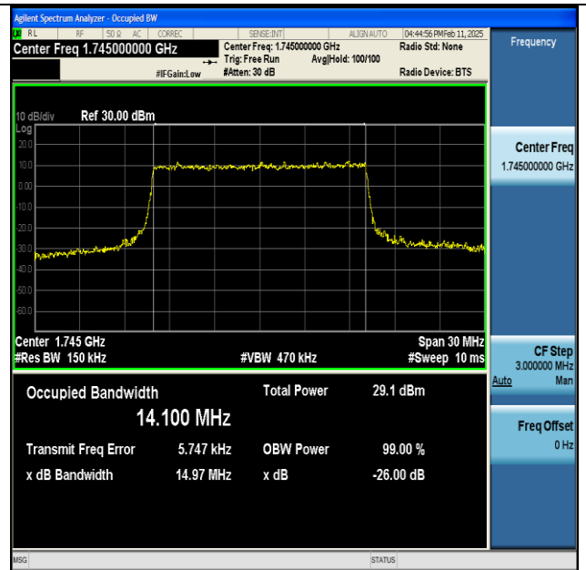
NTNV-n66-PC3-15-15-M-CP-16QAM-Outer_Full-Ant1-PASS
