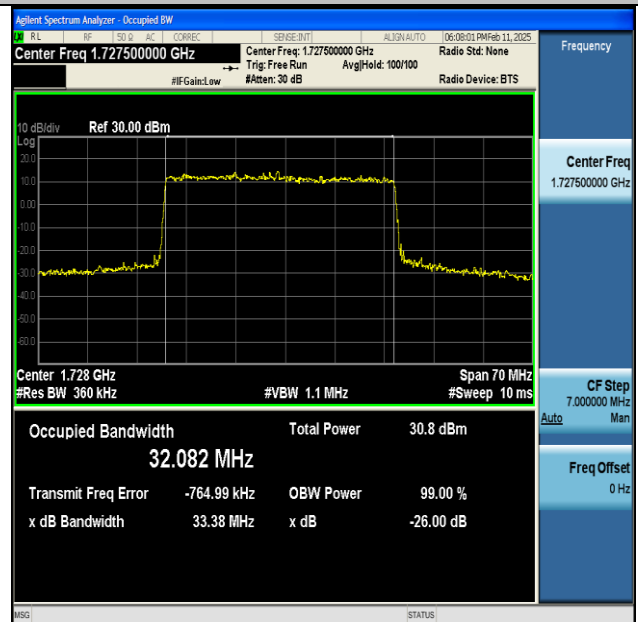
NTNV-n66-PC3-15-35-L-DFT-16QAM-Outer_Full-Ant1- PASS
