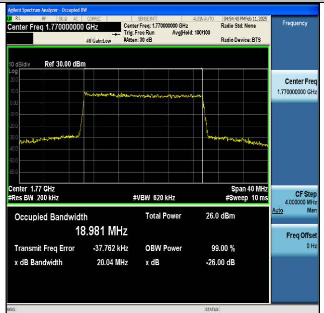
NTNV-n66-PC3-15-20-H-CP-256QAM-Outer_Full-Ant1-PASS
