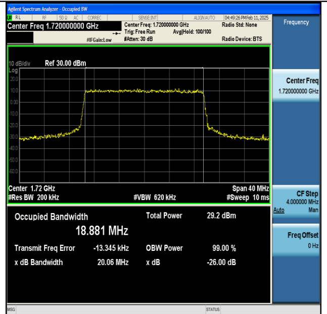
NTNV-n66-PC3-15-20-L-CP-16QAM-Outer_Full-Ant1- PASS
