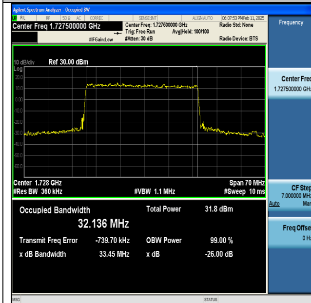
NTNV-n66-PC3-15-35-L-DFT-QPSK-Outer_Full-Ant1- PASS
