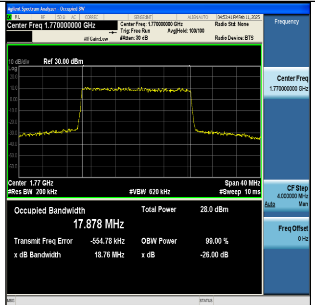
NTNV-n66-PC3-15-20-H-DFT-256QAM-Outer_Full-Ant1- PASS
