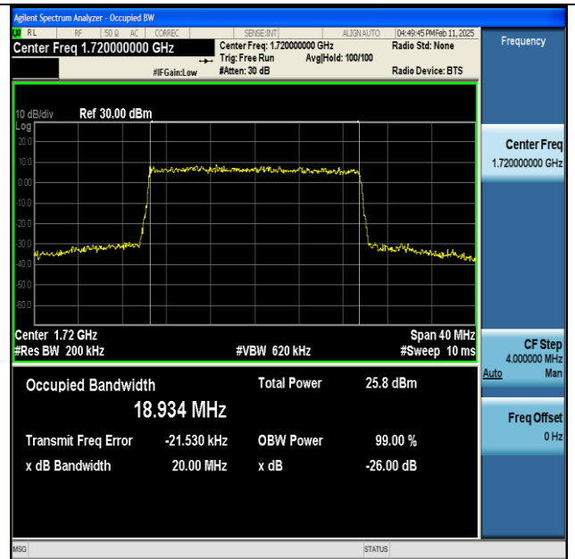
NTNV-n66-PC3-15-20-L-CP-256QAM-Outer_Full-Ant1- PASS
