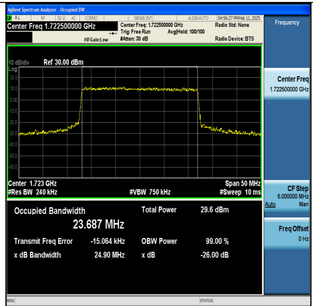
NTNV-n66-PC3-15-25-L-CP-QPSK-Outer_Full-Ant1-PASS
