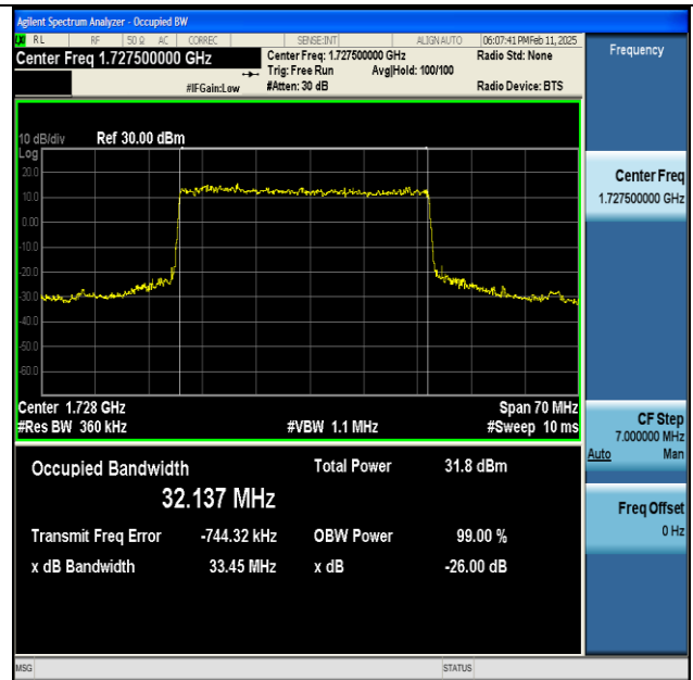
NTNV-n66-PC3-15-35-L-DFT-BPSK-Outer_Full-Ant1- PASS
