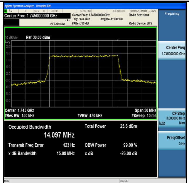
NTNV-n66-PC3-15-15-M-CP-256QAM-Outer_Full-Ant1-PASS
