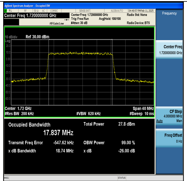
NTNV-n66-PC3-15-20-L-DFT-256QAM-Outer_Full-Ant1- PASS
