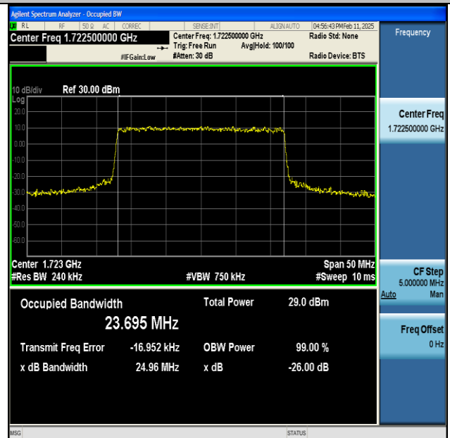
NTNV-n66-PC3-15-25-L-CP-64QAM-Outer_Full-Ant1-PASS
