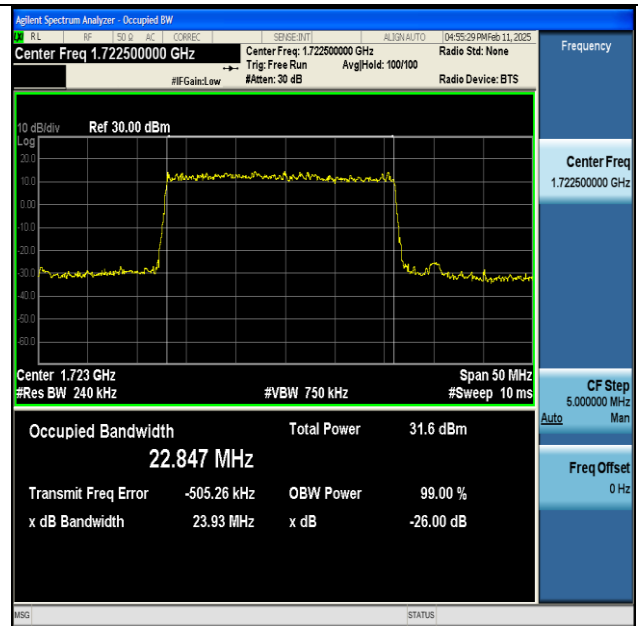
NTNV-n66-PC3-15-25-L-DFT-QPSK-Outter_Full-Ant1- PASS
