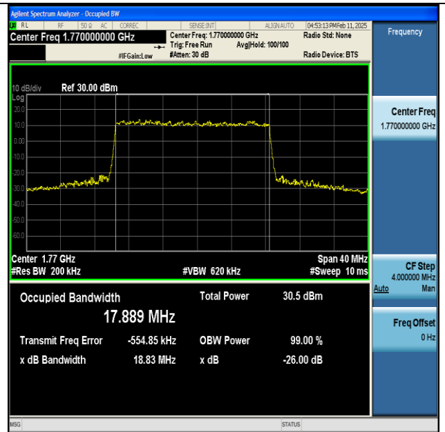
NTNV-n66-PC3-15-20-H-DFT-16QAM-Outer_Full-Ant1- PASS
