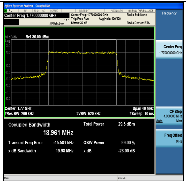
NTNV-n66-PC3-15-20-H-CP-16QAM-Outer_Full-Ant1-PASS
