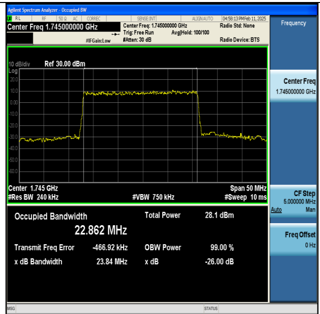
NTNV-n66-PC3-15-25-M-DFT-256QAM-Outer_Full-Ant1- PASS
