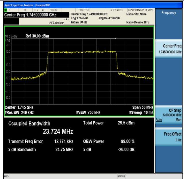
NTNV-n66-PC3-15-25-M-CP-16QAM-Outer_Full-Ant1- PASS
