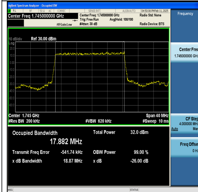
NTNV-n66-PC3-15-20-M-DFT-BPSK-Outer_Full-Ant1- PASS
