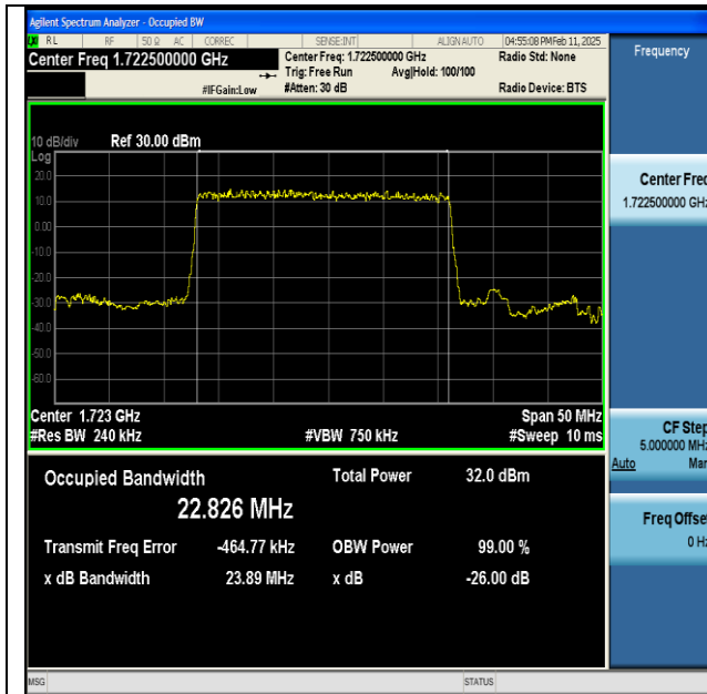
NTNV-n66-PC3-15-25-L-DFT-BPSK-Outter_Full-Ant1- PASS
