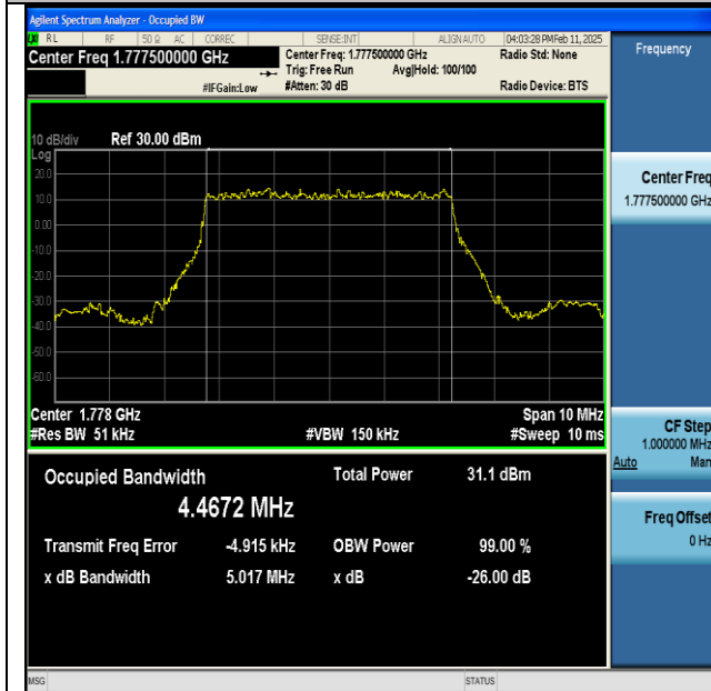
NTNV-n66-PC3-15-5-H-DFT-BPSK-Outer_Full-Ant1-PASS
