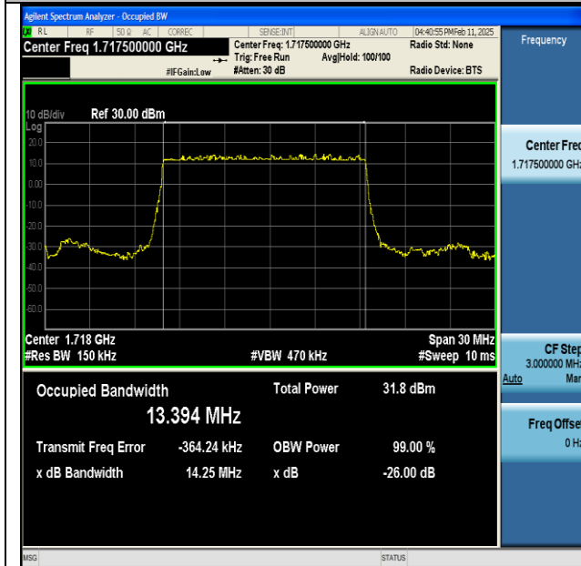
NTNV-n66-PC3-15-15-L-DFT-BPSK-Outer_Full-Ant1- PASS
