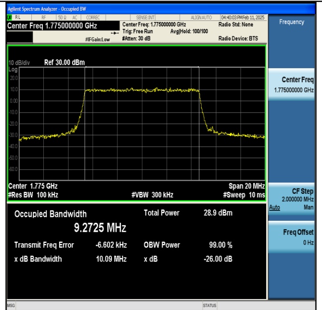
NTNV-n66-PC3-15-10-H-CP-16QAM-Outer_Full-Ant1- PASS
