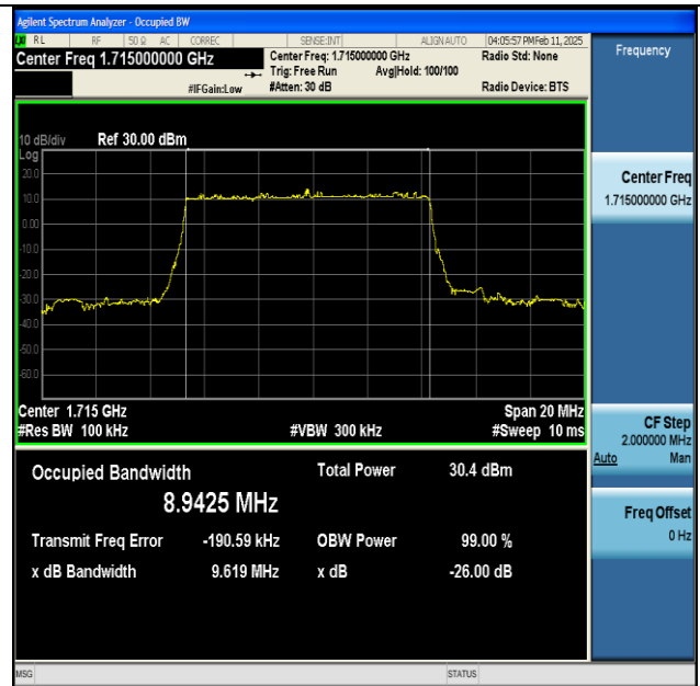
NTNV-n66-PC3-15-10-L-DFT-16QAM-Outer_Full-Ant1- PASS
