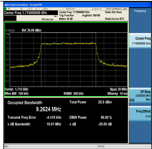
NTNV-n66-PC3-15-10-L-CP-16QAM-Outer_Full-Ant1-PASS
