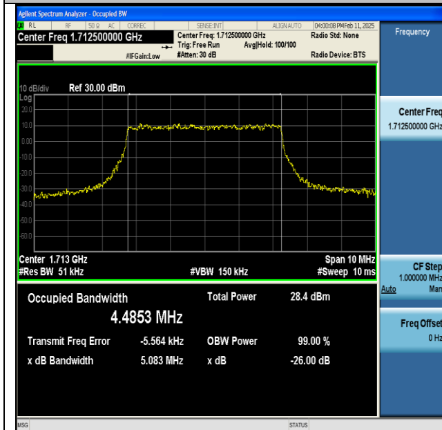
NTNV-n66-PC3-15-5-L-CP-16QAM-Outer_Full-Ant1-PASS
