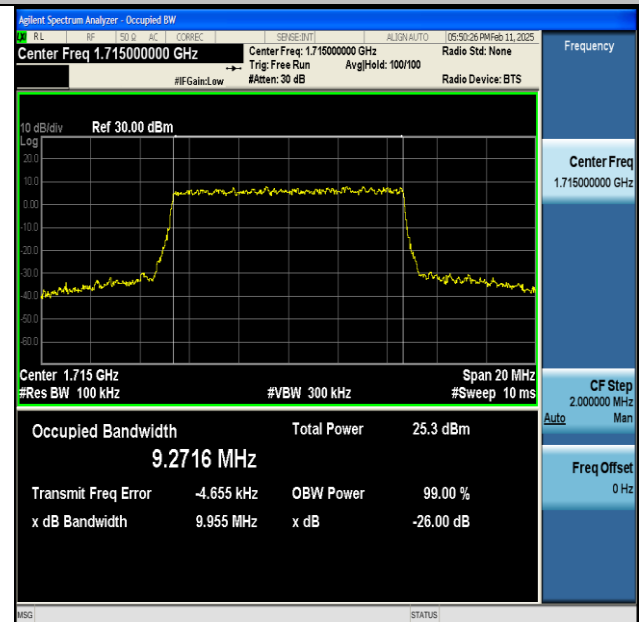
NTNV-n66-PC3-15-10-L-CP-256QAM-Outer_Full-Ant1-PASS
