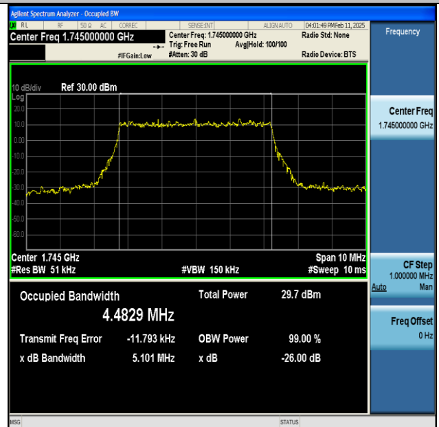
NTNV-n66-PC3-15-5-M-DFT-16QAM-Outer_Full-Ant1-PASS
