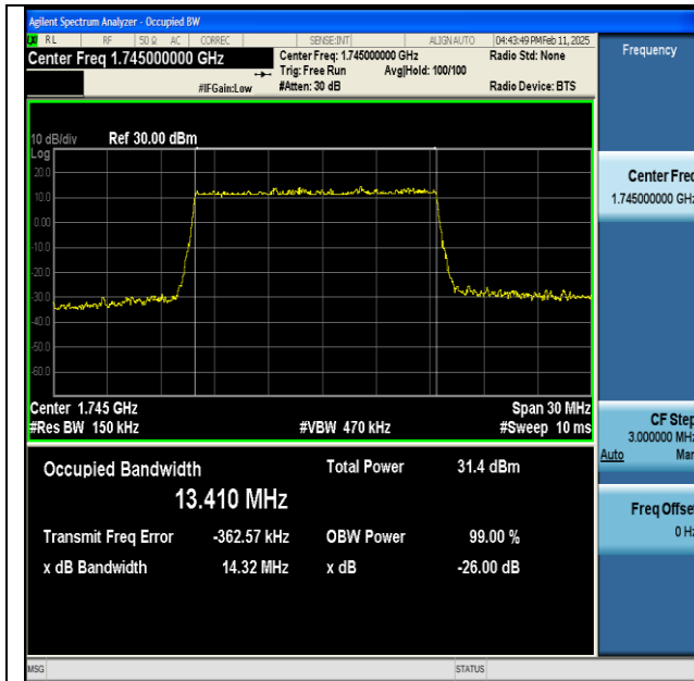
NTNV-n66-PC3-15-15-M-DFT-QPSK-Outer_Full-Ant1- PASS
