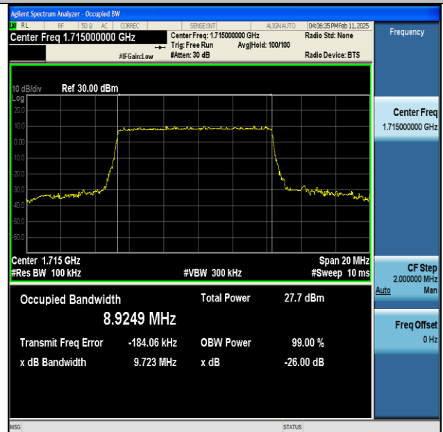
NTNV-n66-PC3-15-10-L-DFT-256QAM-Outer_Full-Ant1- PASS
