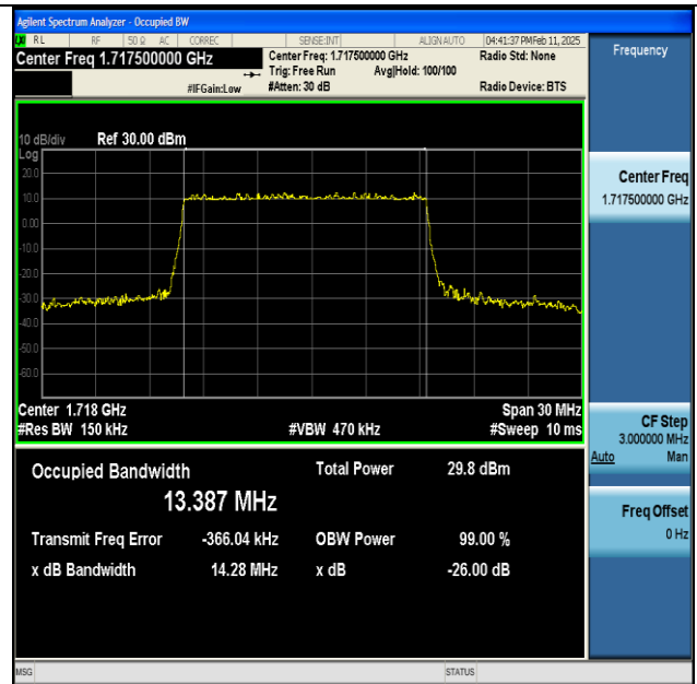
NTNV-n66-PC3-15-15-L-DFT-64QAM-Outer_Full-Ant1- PASS
