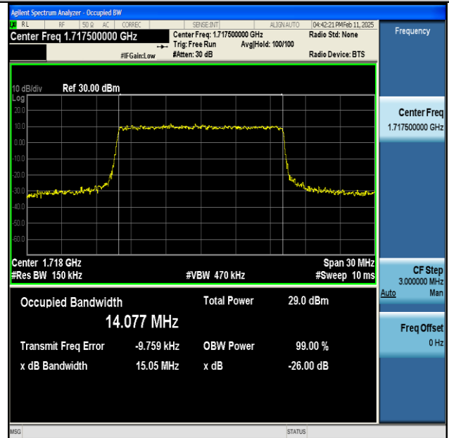
NTNV-n66-PC3-15-15-L-DFT-64QAM-Outer_Full-Ant1- PASS
