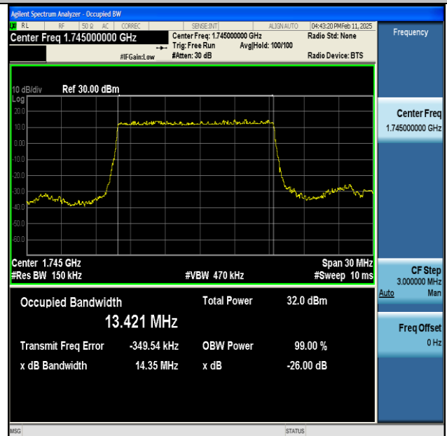
NTNV-n66-PC3-15-15-M-DFT-BPSK-Outer_Full-Ant1- PASS
