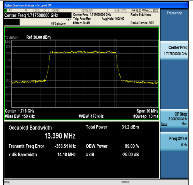
NTNV-n66-PC3-15-15-L-DFT-QPSK-Outer_Full-Ant1- PASS
