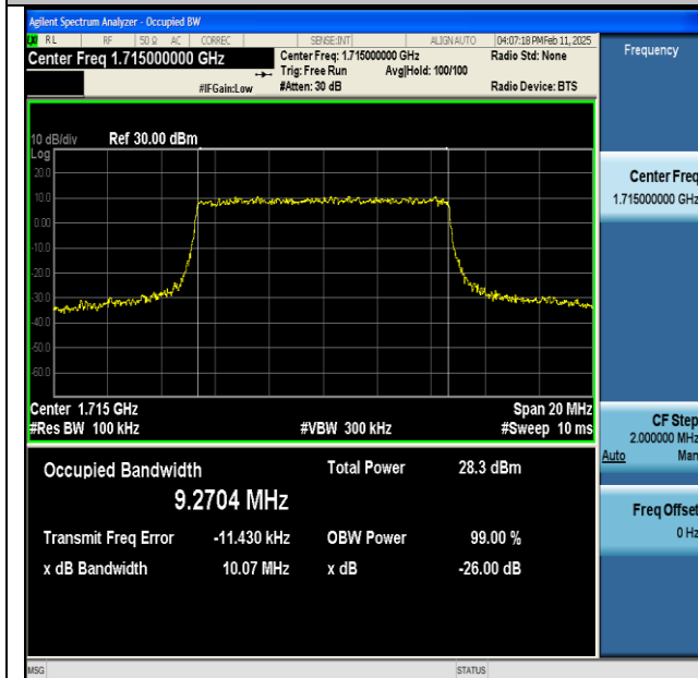
NTNV-n66-PC3-15-10-L-CP-64QAM-Outer_Full-Ant1-PASS
