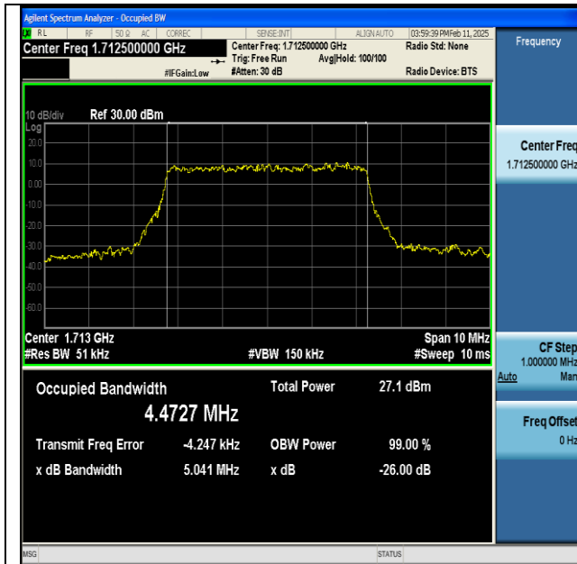
NTNV-n66-PC3-15-5-L-DFT-256QAM-Outer_Full-Ant1-PASS
