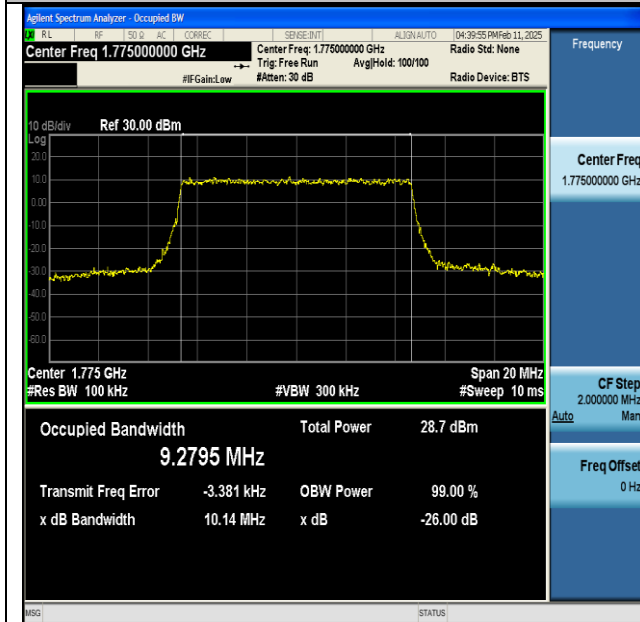
NTNV-n66-PC3-15-10-H-DFT-64QAM-Outer_Full-Ant1- PASS
