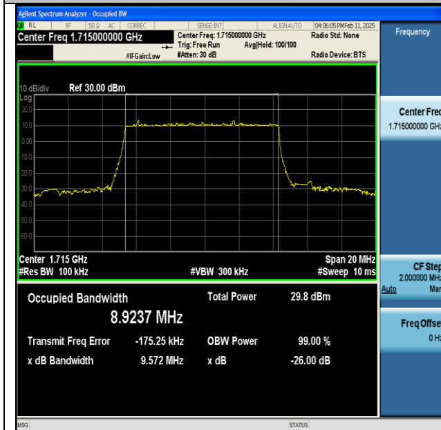
NTNV-n66-PC3-15-10-L-DFT-64QAM-Outer_Full-Ant1- PASS
