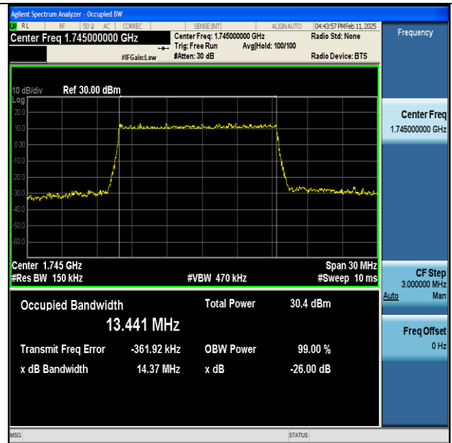
NTNV-n66-PC3-15-15-M-DFT-16QAM-Outer_Full-Ant1- PASS
