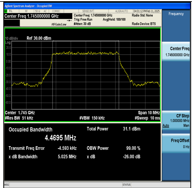
NTNV-n66-PC3-15-5-M-DFT-BPSK-Outer_Full-Ant1-PASS
