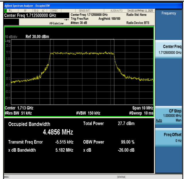
NTNV-n66-PC3-15-5-L-CP-64QAM-Outer_Full-Ant1-PASS
