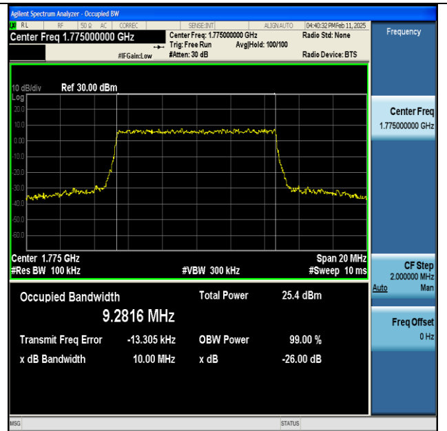
NTNV-n66-PC3-15-10-H-CP-256QAM-Outer_Full-Ant1- PASS
