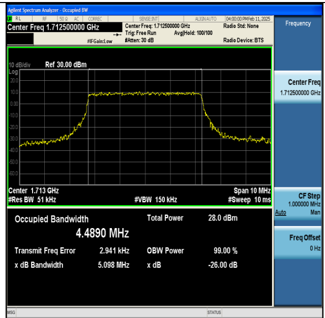
NTNV-n66-PC3-15-5-L-CP-QPSK-Outer_Full-Ant1-PASS
