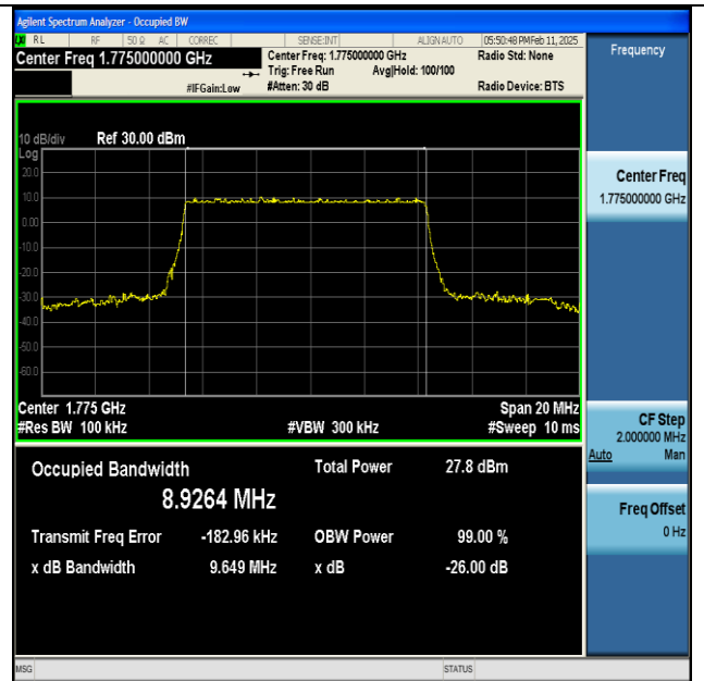
NTNV-n66-PC3-15-10-H-DFT-256QAM-Outer_Full-Ant1- PASS
