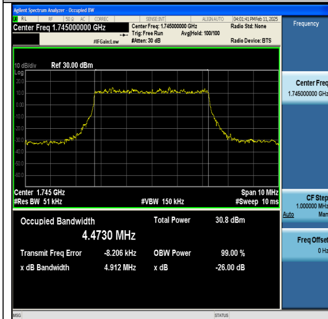
NTNV-n66-PC3-15-5-L-CP-256QAM-Outer_Full-Ant1-PASS
