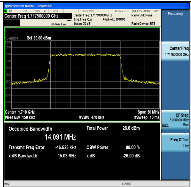
NTNV-n66-PC3-15-15-L-CP-64QAM-Outer_Full-Ant1- PASS
