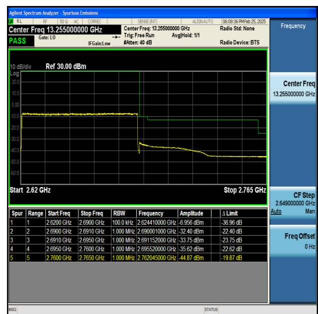
NTNV-n41-PC2-30-70-H-CP-QPSK-Outer_Full-PASS
