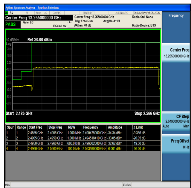
NTNV-n41-PC2-30-70-L-CP-QPSK-Outer_Full-PASS
