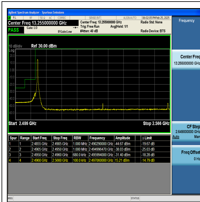
NTNV-n41-PC2-30-70-L-DFT-BPSK-Edge_1RB_Left-PASS
