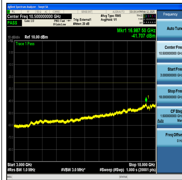
NTNV-n41-PC2-30-100-H-CP-QPSK-Edge_1RB_Left-3000-18000-PASS
