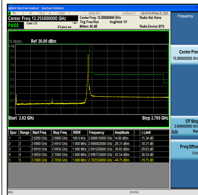
NTNV-n41-PC2-30-70-H-CP-QPSK-Edge_1RB_Right-PASS
