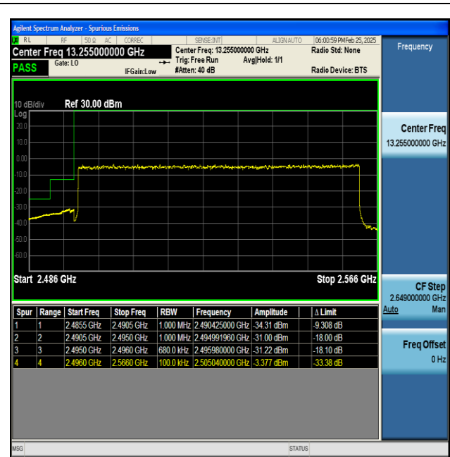
NTNV-n41-PC2-30-70-L-DFT-BPSK-Outer_Full-PASS
