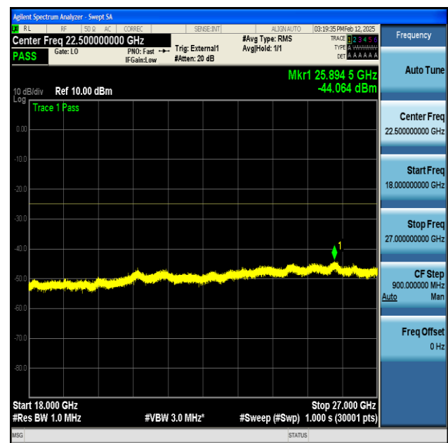
NTNV-n41-PC2-30-100-H-CP-QPSK-Edge_1RB_Left-18000-27000-PASS
