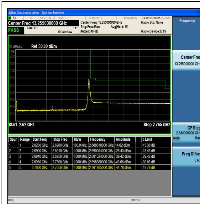
NTNV-n41-PC2-30-70-H-DFT-BPSK-Edge_1RB_Right-PASS
