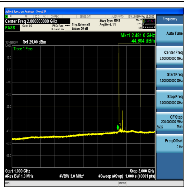
NTNV-n41-PC2-30-100-L-CP-QPSK-Edge_1RB_Left-1000-3000-PASS
