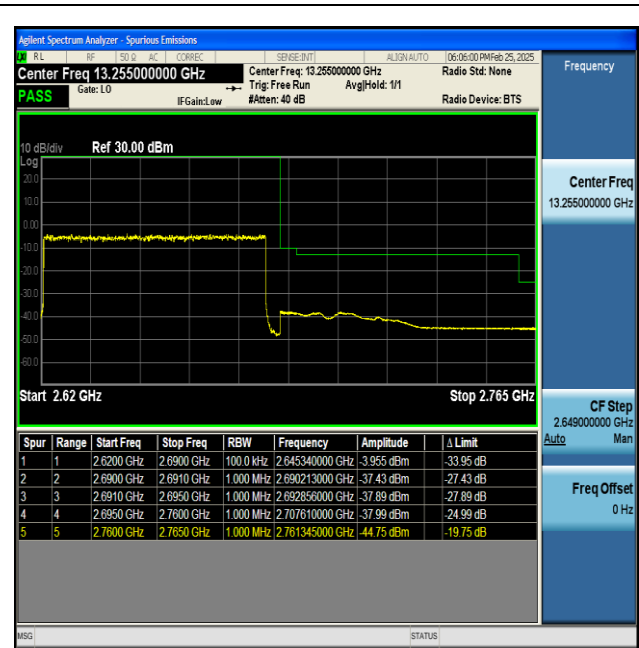
NTNV-n41-PC2-30-70-H-DFT-BPSK-Outer_Full-PASS
