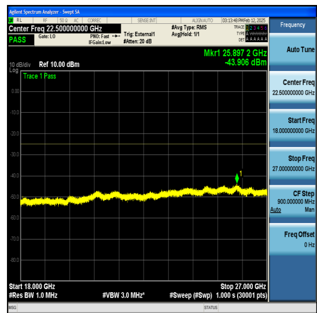
NTNV-n41-PC2-30-100-L-CP-QPSK-Edge_1RB_Left-18000-27000-PASS
