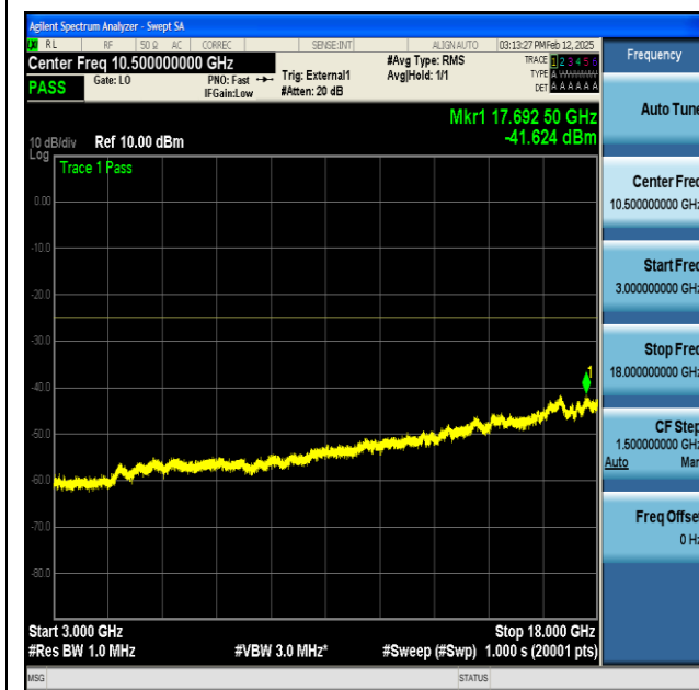
NTNV-n41-PC2-30-100-L-CP-QPSK-Edge_1RB_Left-3000-18000-PASS
