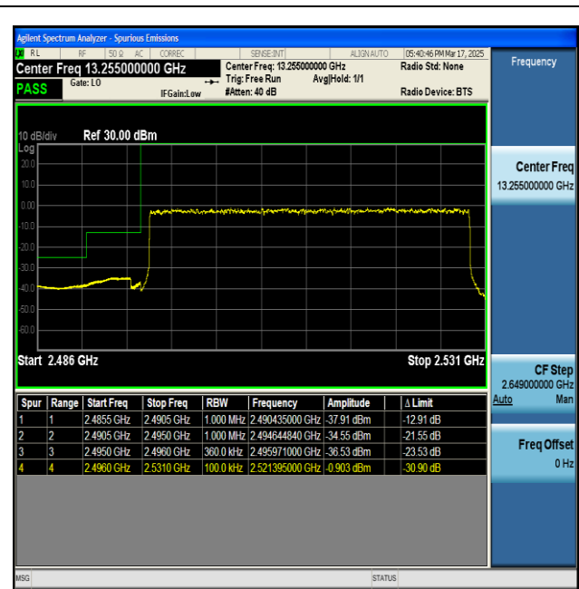
NTNV-n41-PC2-30-35-L-DFT-BPSK-Outer_Full-PASS
