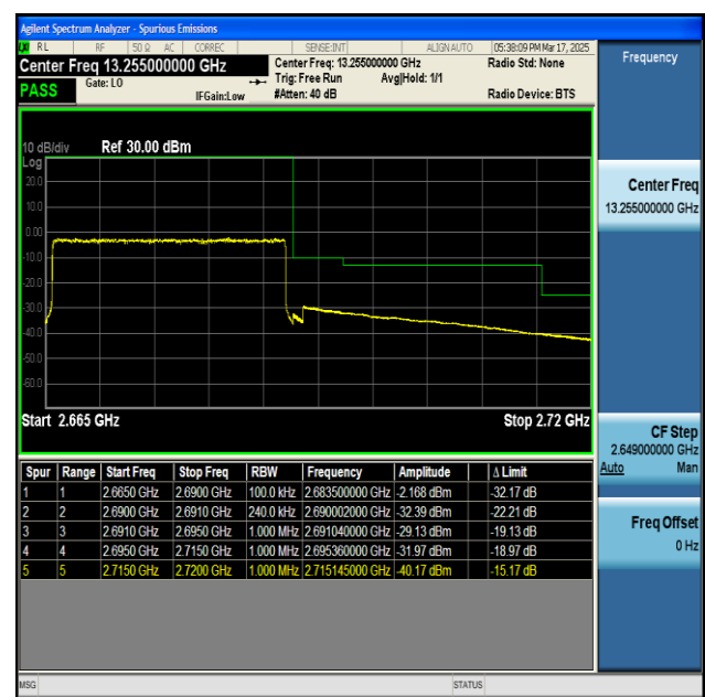
NTNV-n41-PC2-30-25-H-CP-QPSK-Outer_Full-PASS
