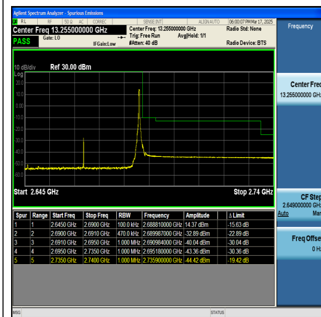
NTNV-n41-PC2-30-45-H-CP-QPSK-Edge_1RB_Right-PASS
