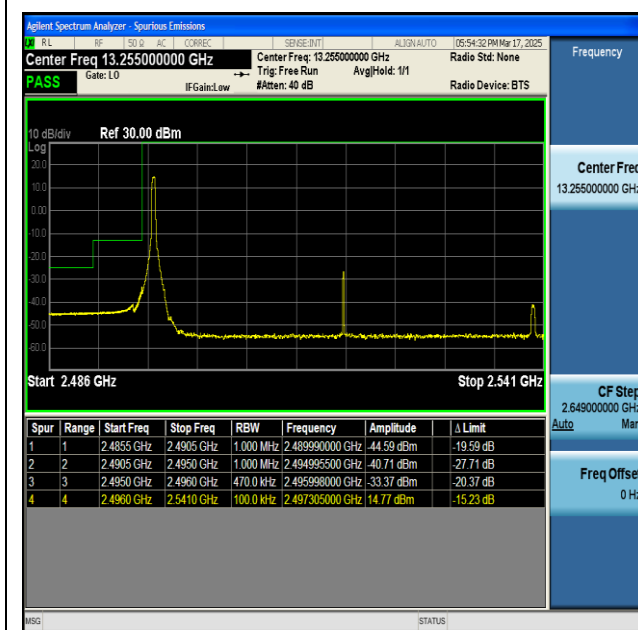
NTNV-n41-PC2-30-45-L-CP-QPSK-Edge_1RB_Left-PASS
