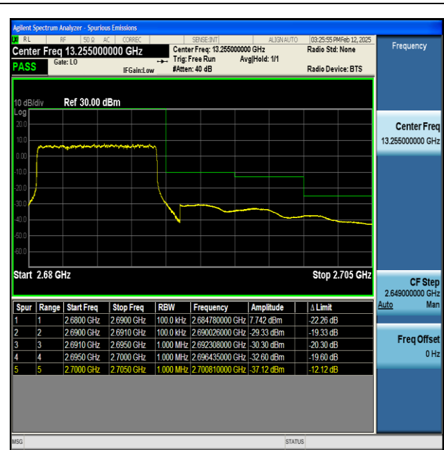
NTNV-n41-PC2-30-10-H-DFT-BPSK-Outer_Full-PASS
