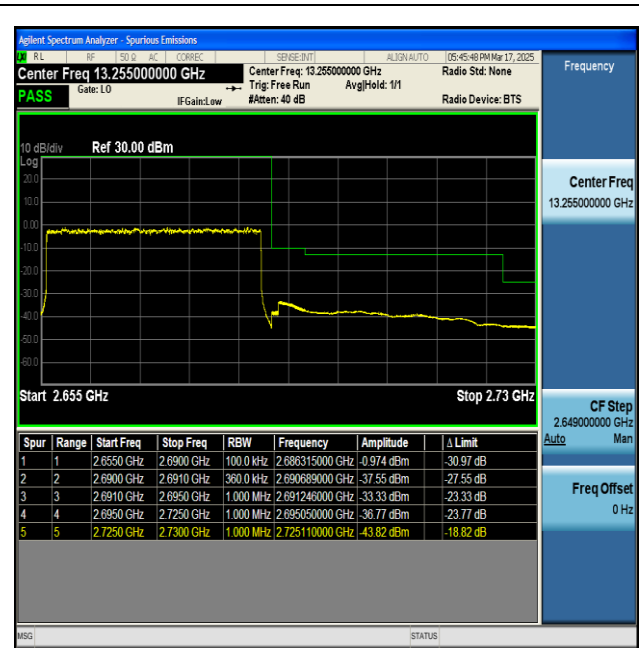
NTNV-n41-PC2-30-35-H-DFT-BPSK-Outer_Full-PASS
