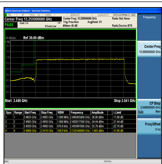
NTNV-n41-PC2-30-45-L-DFT-BPSK-Outer_Full-PASS
