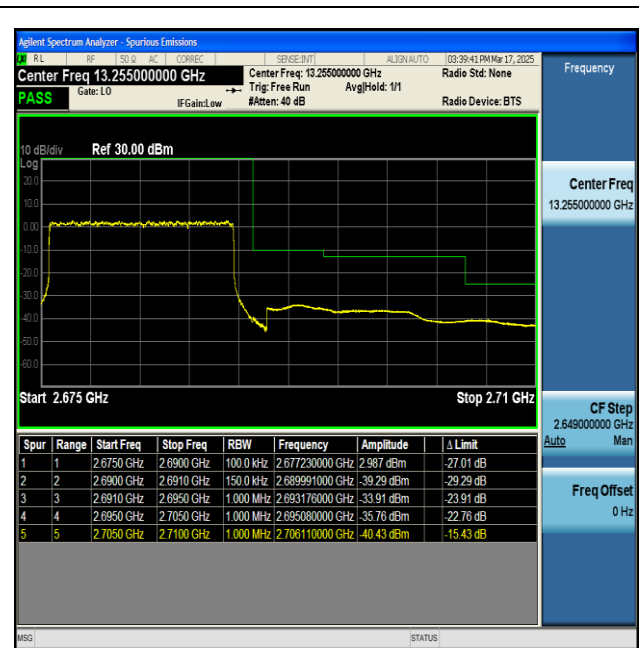
NTNV-n41-PC2-30-15-H-DFT-BPSK-Outer_Full-PASS
