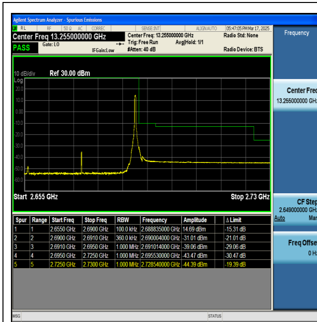
NTNV-n41-PC2-30-35-H-DFT-BPSK-Edge_1RB_Right-PASS
