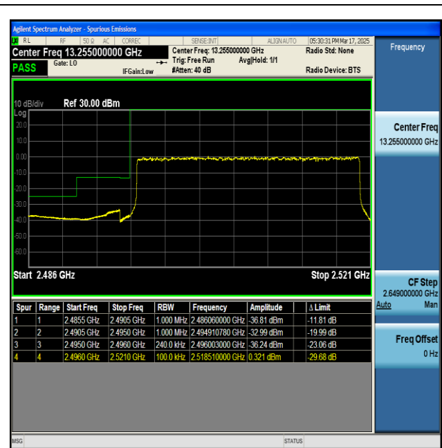
NTNV-n41-PC2-30-25-L-DFT-BPSK-Outer_Full-PASS
