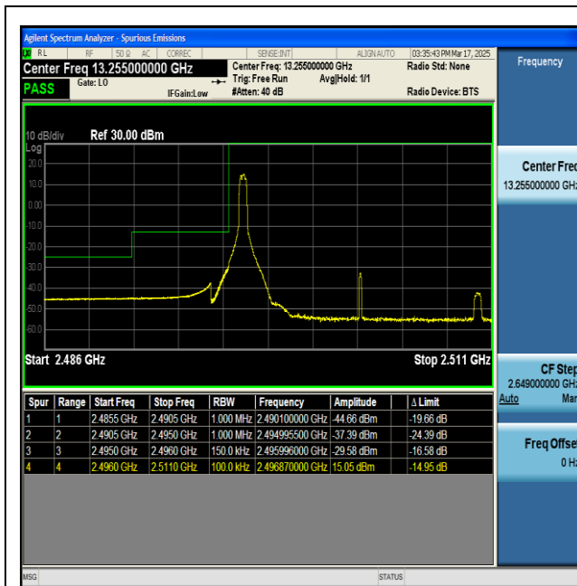
NTNV-n41-PC2-30-15-L-DFT-BPSK-Edge_1RB_Left-PASS
