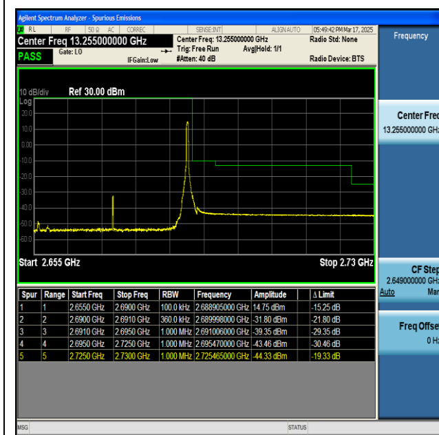
NTNV-n41-PC2-30-35-H-CP-QPSK-Edge_1RB_Right-PASS
