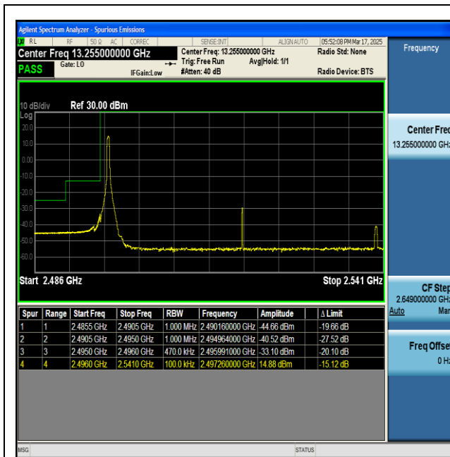
NTNV-n41-PC2-30-45-L-DFT-BPSK-Edge_1RB_Left-PASS
