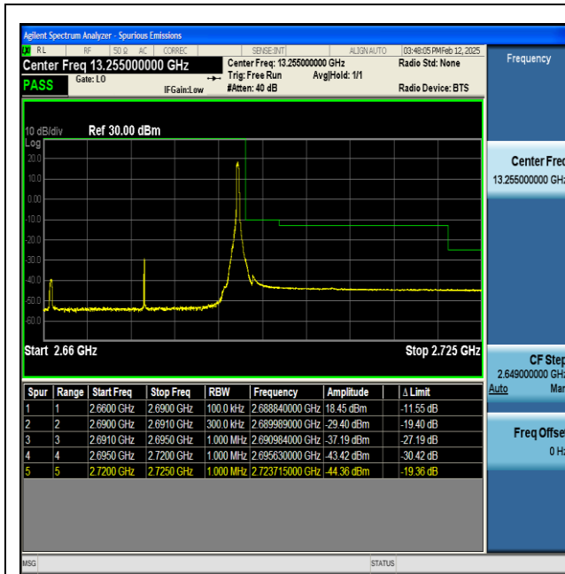
NTNV-n41-PC2-30-30-H-DFT-BPSK-Edge_1RB_Right-PASS
