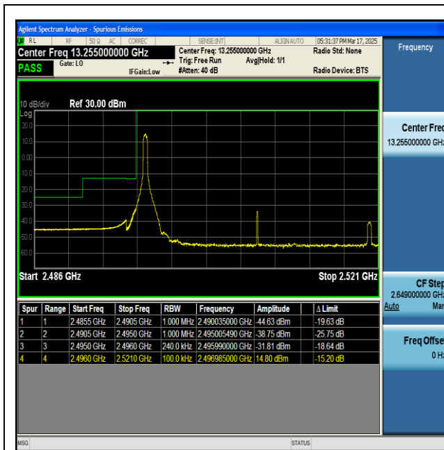
NTNV-n41-PC2-30-25-L-DFT-BPSK-Edge_1RB_Left-PASS
