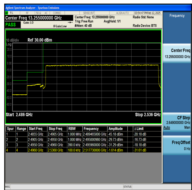
NTNV-n41-PC2-30-40-L-CP-QPSK-Outer_Full-PASS
