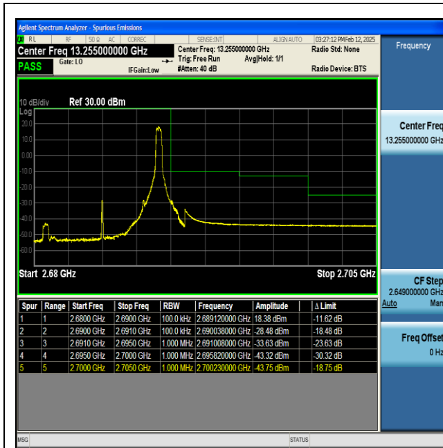
NTNV-n41-PC2-30-10-H-DFT-BPSK-Edge_1RB_Right-PASS
