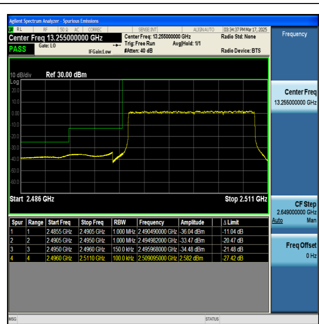
NTNV-n41-PC2-30-15-L-DFT-BPSK-Outer_Full-PASS
