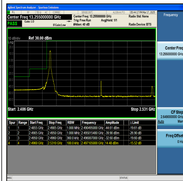
NTNV-n41-PC2-30-35-L-CP-QPSK-Edge_1RB_Left-PASS
