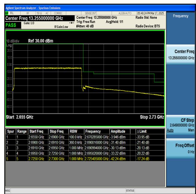
NTNV-n41-PC2-30-35-H-CP-QPSK-Outer_Full-PASS
