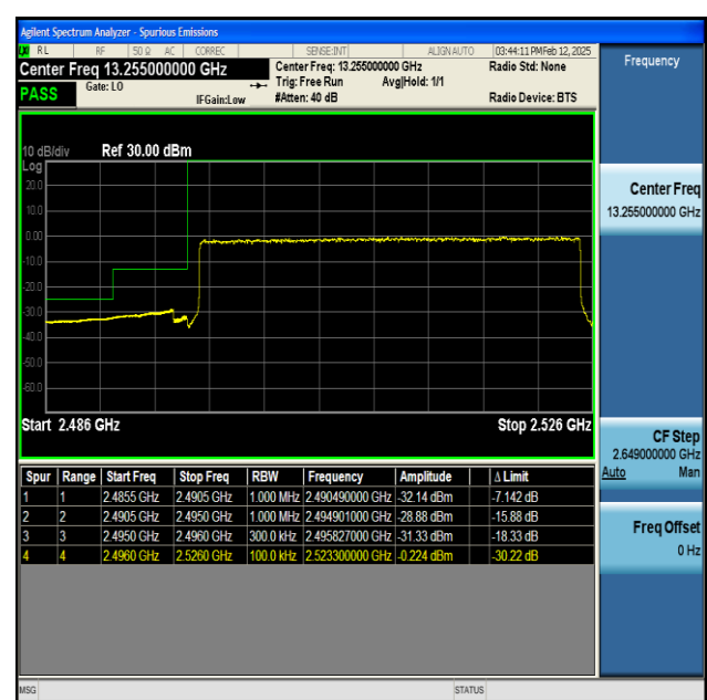
NTNV-n41-PC2-30-30-L-CP-QPSK-Outer_Full-PASS
