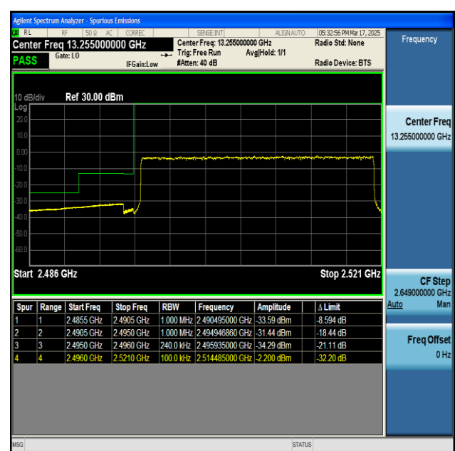
NTNV-n41-PC2-30-25-L-CP-QPSK-Outer_Full-PASS
