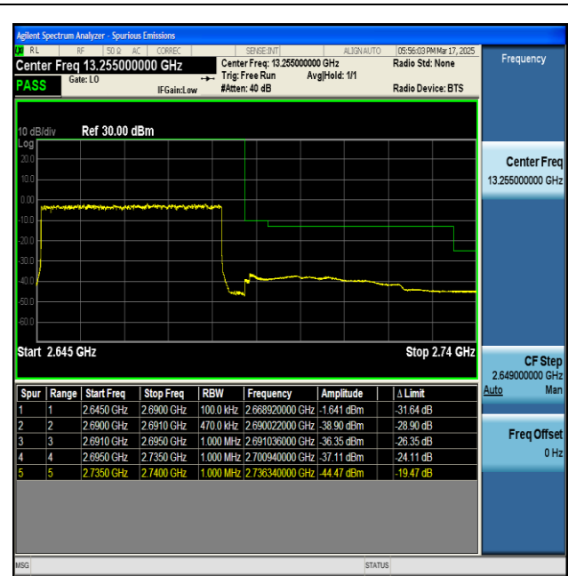
NTNV-n41-PC2-30-45-H-DFT-BPSK-Outer_Full-PASS
