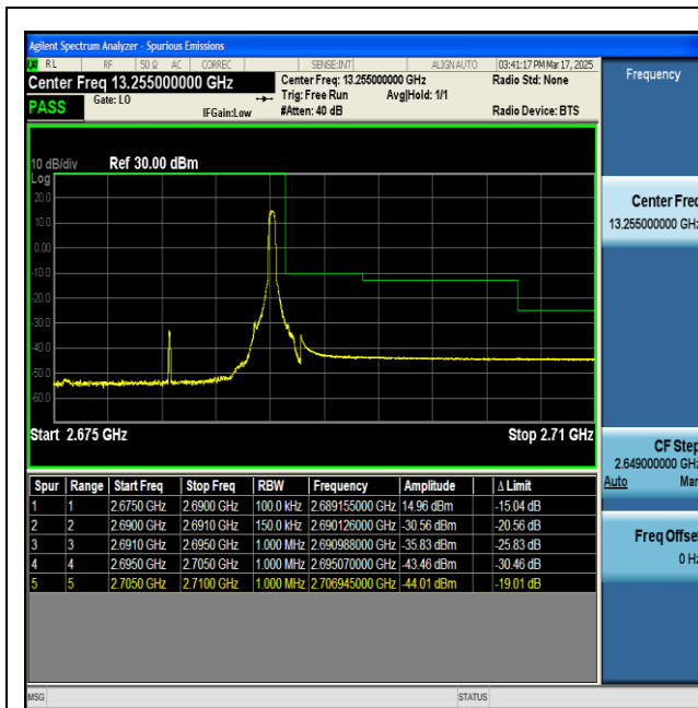
NTNV-n41-PC2-30-15-H-DFT-BPSK-Edge_1RB_Right-PASS
