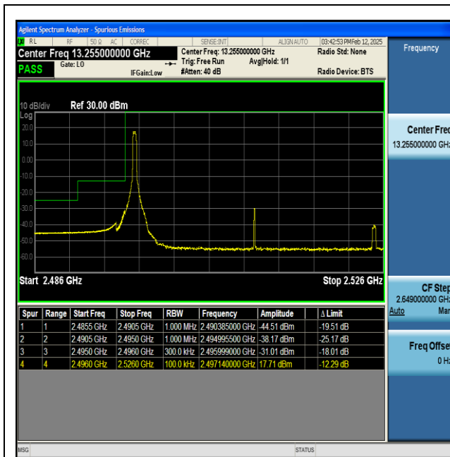
NTNV-n41-PC2-30-30-L-DFT-BPSK-Edge_1RB_Left-PASS
