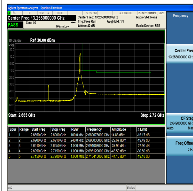
NTNV-n41-PC2-30-25-H-CP-QPSK-Edge_1RB_Right-PASS
