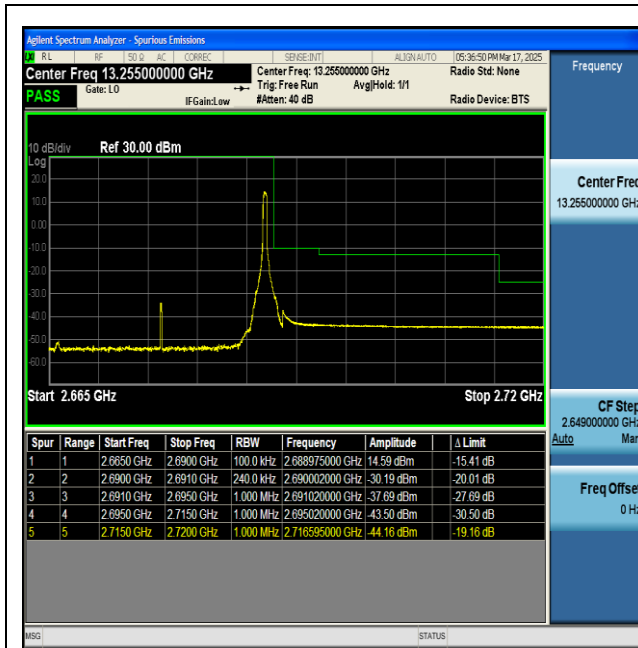
NTNV-n41-PC2-30-25-H-DFT-BPSK-Edge_1RB_Right-PASS
