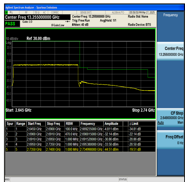
NTNV-n41-PC2-30-45-H-CP-QPSK-Outer_Full-PASS
