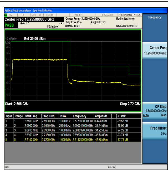
NTNV-n41-PC2-30-25-H-DFT-BPSK-Outer_Full-PASS
