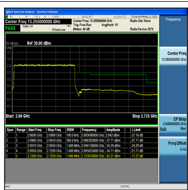
NTNV-n41-PC2-30-30-H-DFT-BPSK-Outer_Full-PASS
