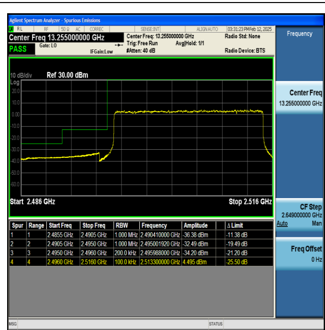
NTNV-n41-PC2-30-20-L-DFT-BPSK-Outer_Full-PASS
