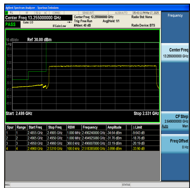
NTNV-n41-PC2-30-35-L-CP-QPSK-Outer_Full-PASS
