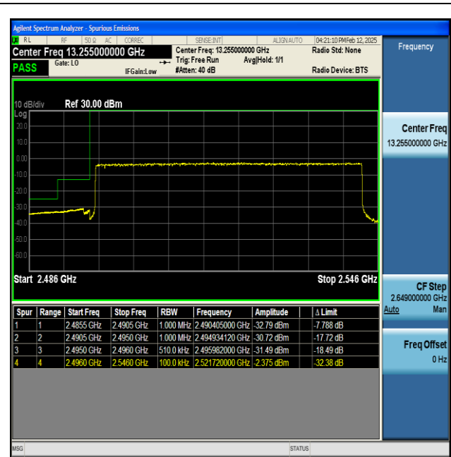
NTNV-n41-PC2-30-50-L-DFT-BPSK-Outer_Full-PASS
