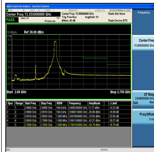
NTNV-n41-PC2-30-10-H-CP-QPSK-Edge_1RB_Right-PASS
