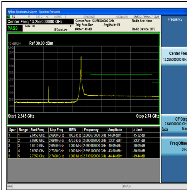
NTNV-n41-PC2-30-45-H-DFT-BPSK-Edge_1RB_Right-PASS
