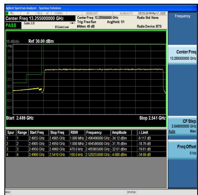
NTNV-n41-PC2-30-45-L-CP-QPSK-Outer_Full-PASS
