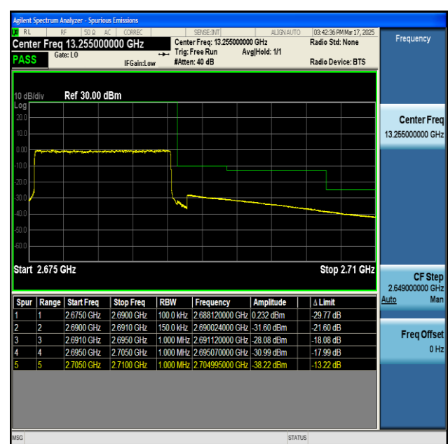
NTNV-n41-PC2-30-15-H-CP-QPSK-Outer_Full-PASS
