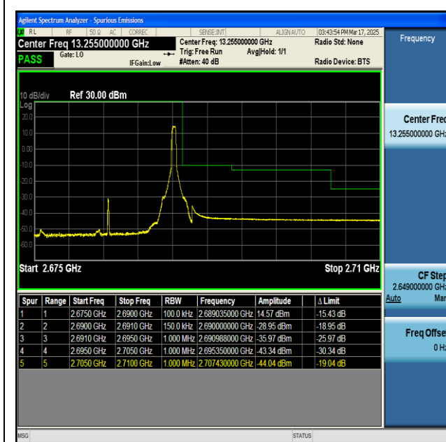
NTNV-n41-PC2-30-15-H-CP-QPSK-Edge_1RB_Right-PASS
