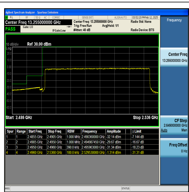
NTNV-n41-PC2-30-40-L-DFT-BPSK-Outer_Full-PASS
