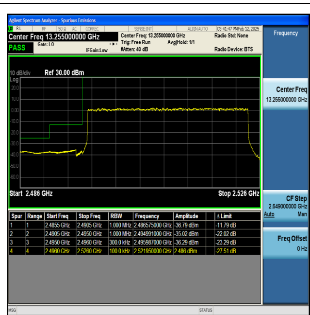
NTNV-n41-PC2-30-30-L-DFT-BPSK-Outer_Full-PASS
