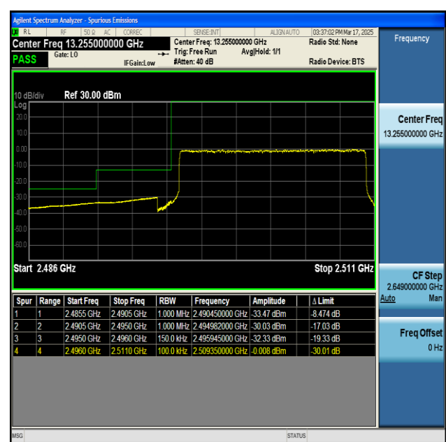
NTNV-n41-PC2-30-15-L-CP-QPSK-Outer_Full-PASS
