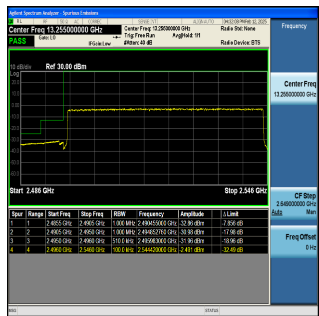
NTNV-n41-PC2-30-50-L-CP-QPSK-Outer_Full-PASS
