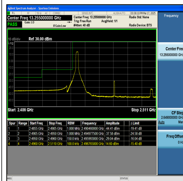
NTNV-n41-PC2-30-15-L-CP-QPSK-Edge_1RB_Left-PASS
