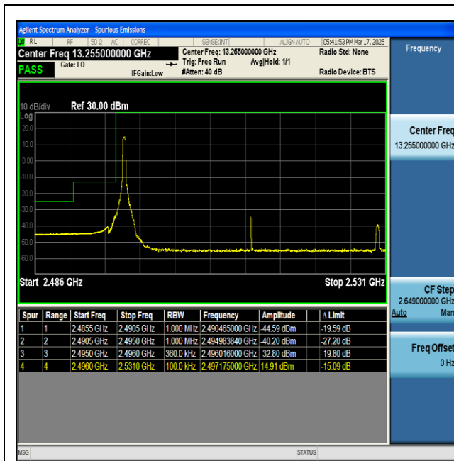
NTNV-n41-PC2-30-35-L-DFT-BPSK-Edge_1RB_Left-PASS
