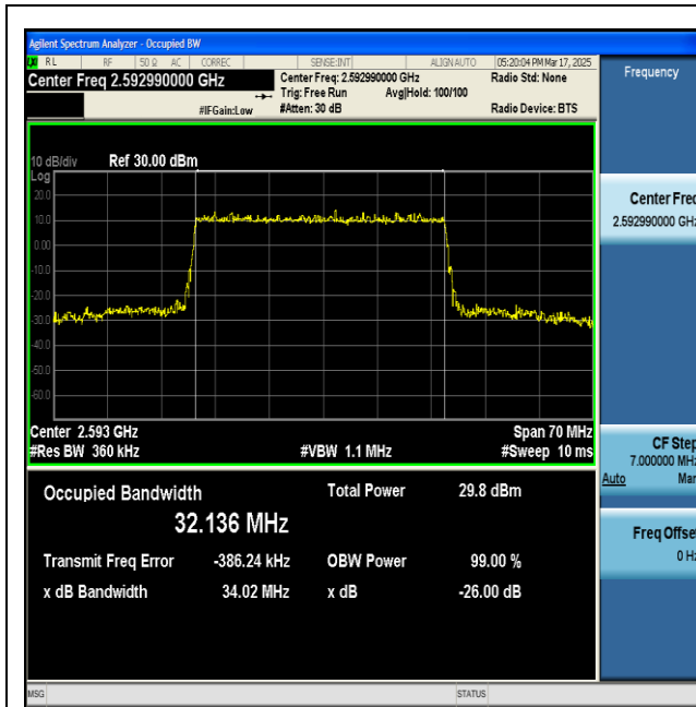
NTNV-n41-PC2-30-35-M-DFT-256QAM-Outer_Full-Ant1-PASS
