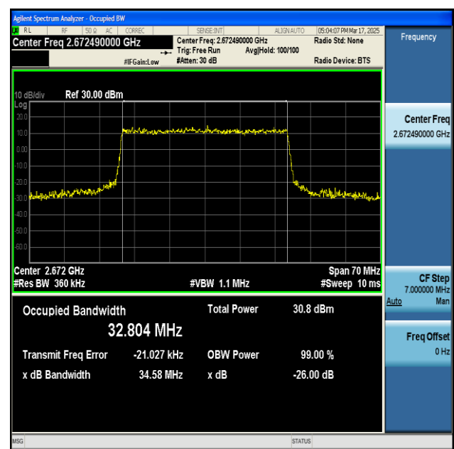
NTNV-n41-PC2-30-35-H-CP-16QAM-Outer_Full-Ant1- PASS
