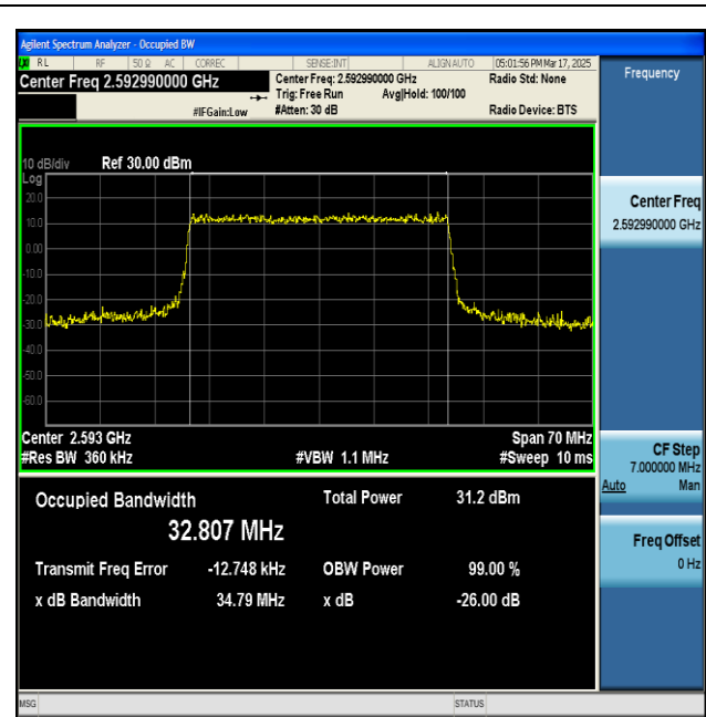
NTNV-n41-PC2-30-35-M-CP-QPSK-Outer_Full-Ant1-PASS
