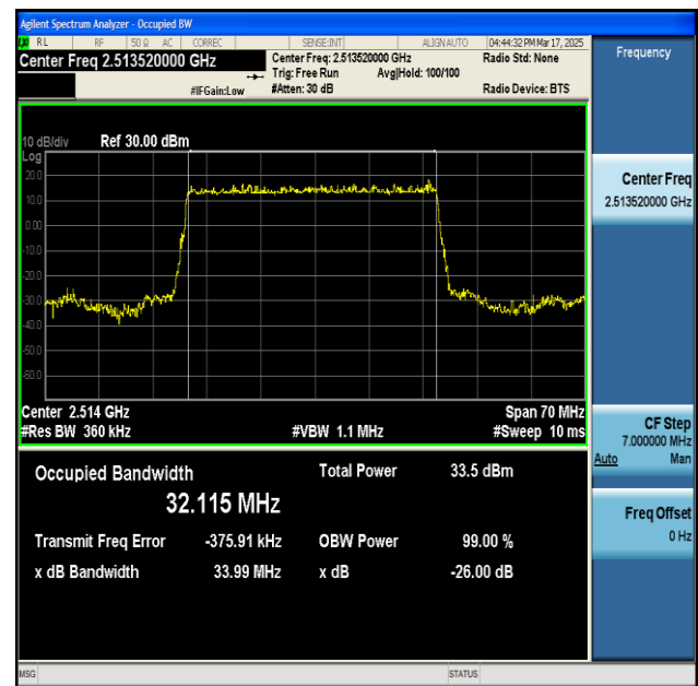
NTNV-n41-PC2-30-35-L-DFT-BPSK-Outer_Full-Ant1- PASS
