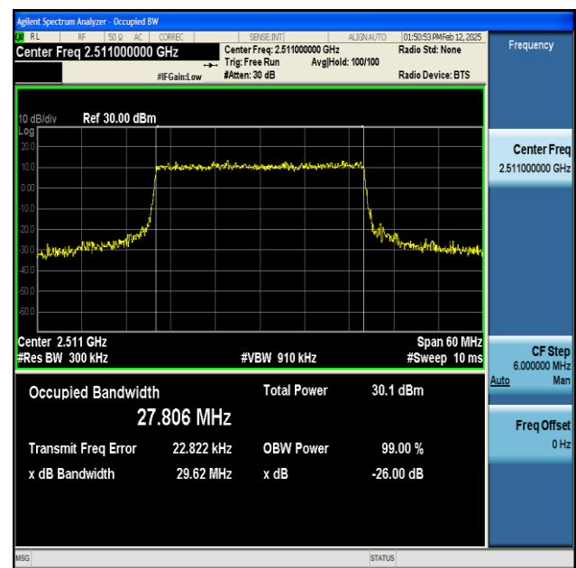
NTNV-n41-PC2-30-30-L-CP-64QAM-Outer_Full-Ant1-PASS
