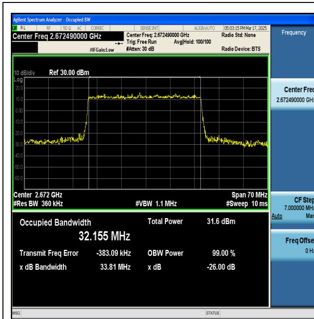
NTNV-n41-PC2-30-35-H-DFT-64QAM-Outer_Full-Ant1- PASS
