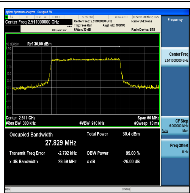
NTNV-n41-PC2-30-30-L-CP-QPSK-Outer_Full-Ant1-PASS
