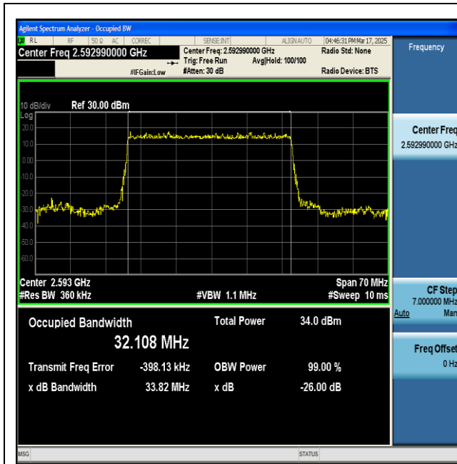
NTNV-n41-PC2-30-35-M-DFT-BPSK-Outer_Full-Ant1- PASS
