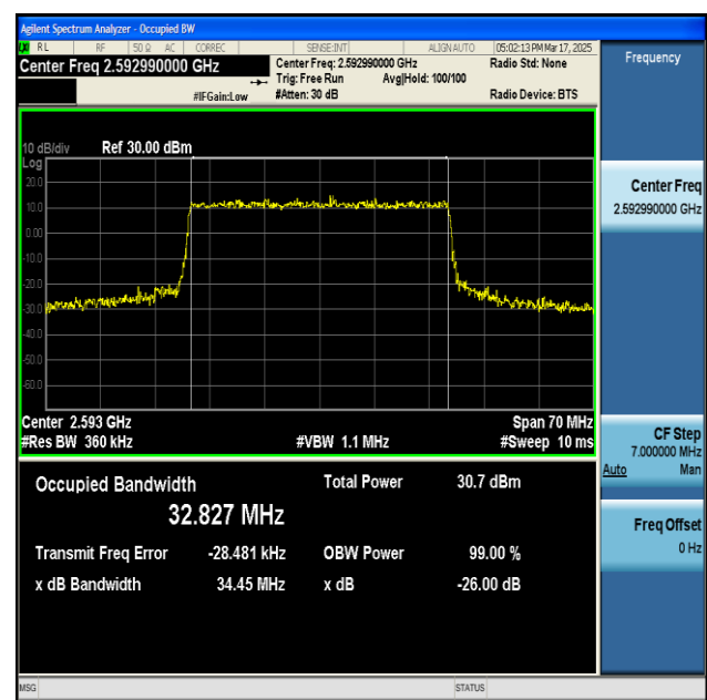
NTNV-n41-PC2-30-35-M-CP-64QAM-Outer_Full-Ant1-PASS
