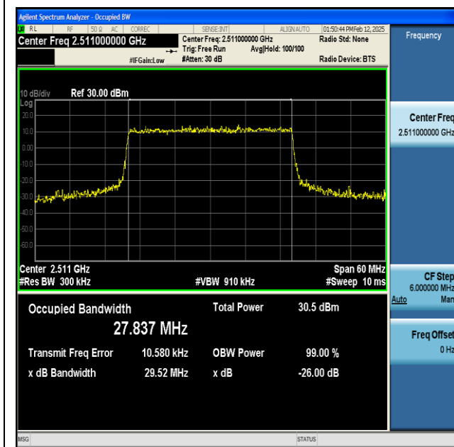
NTNV-n41-PC2-30-30-L-CP-16QAM-Outer_Full-Ant1-PASS
