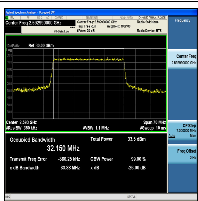
NTNV-n41-PC2-30-35-M-DFT-QPSK-Outer_Full-Ant1- PASS
