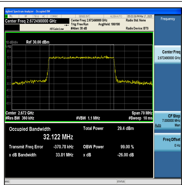
NTNV-n41-PC2-30-35-H-DFT-256QAM-Outer_Full-Ant1- PASS
