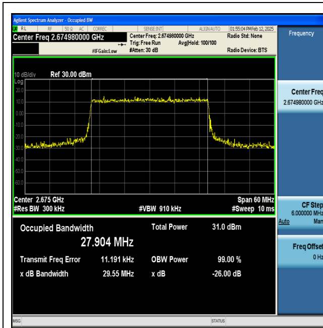
NTNV-n41-PC2-30-30-H-CP-16QAM-Outer_Full-Ant1- PASS
