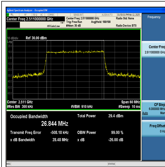
NTNV-n41-PC2-30-30-L-DFT-256QAM-Outer_Full-Ant1-PASS
