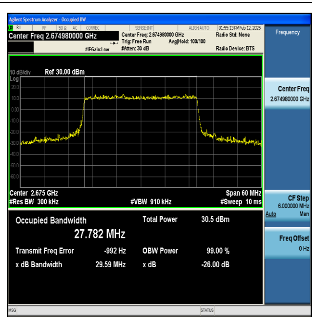
NTNV-n41-PC2-30-30-H-CP-64QAM-Outer_Full-Ant1- PASS
