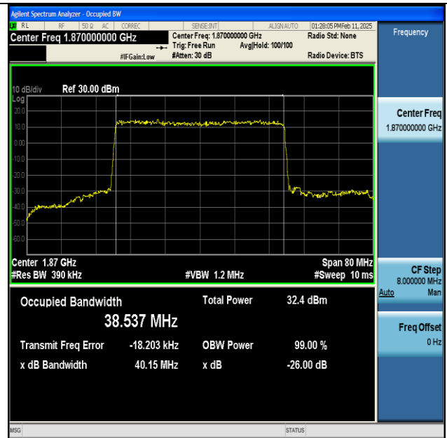
NTNV-n25-PC3-15-40-L-DFT-BPSK-Outer_Full-Ant1- PASS
