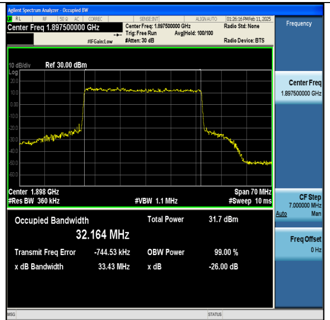
NTNV-n25-PC3-15-35-H-DFT-QPSK-Outet_Full-Ant1- PASS
