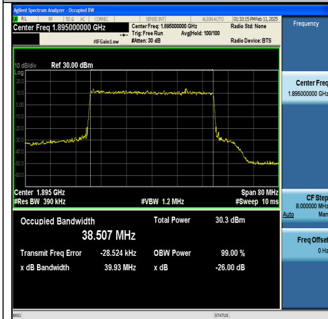
NTNV-n25-PC3-15-40-H-DFT-64QAM-Outer_Full-Ant1- PASS
