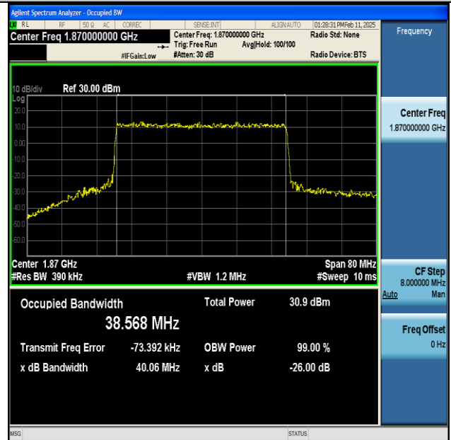
NTNV-n25-PC3-15-40-L-DFT-16QAM-Outer_Full-Ant1- PASS
