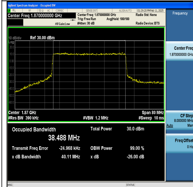
NTNV-n25-PC3-15-40-L-DFT-64QAM-Outer_Full-Ant1- PASS
