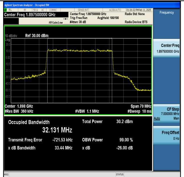
NTNV-n25-PC3-15-35-H-DFT-64QAM-Outet_Full-Ant1- PASS
