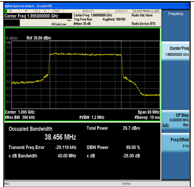
NTNV-n25-PC3-15-40-H-CP-16QAM-Outer_Full-Ant1-PASS
