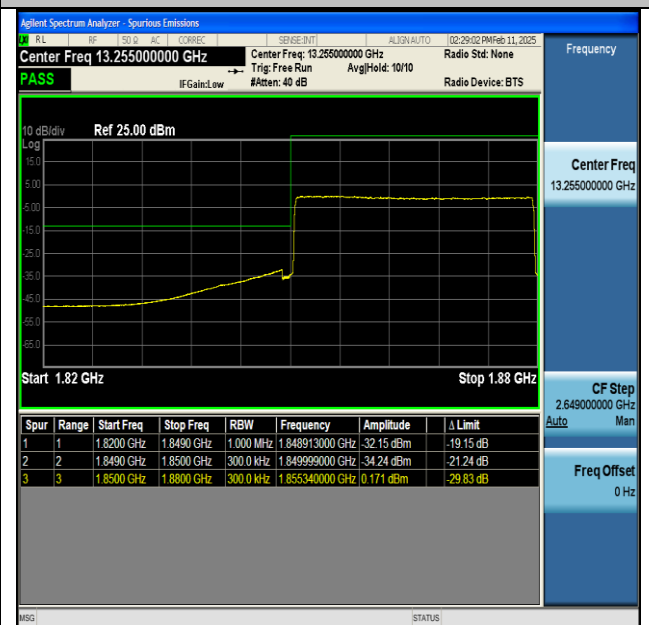
NTNV-n25-PC3-15-30-L-CP-QPSK-Outer_Full-PASS
