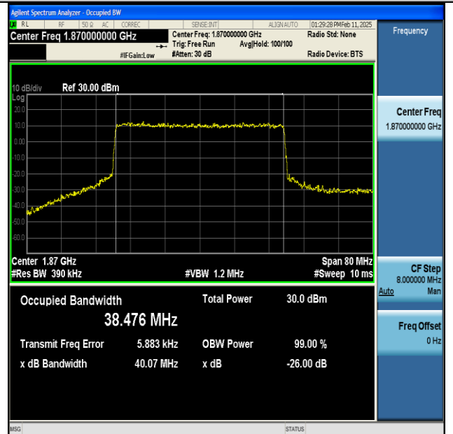
NTNV-n25-PC3-15-40-L-CP-16QAM-Outer_Full-Ant1- PASS
