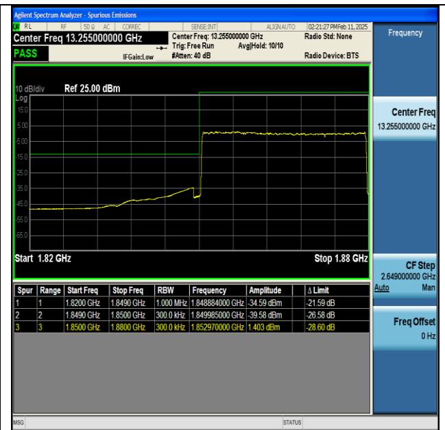
NTNV-n25-PC3-15-30-L-DFT-BPSK-Outer_Full-PASS
