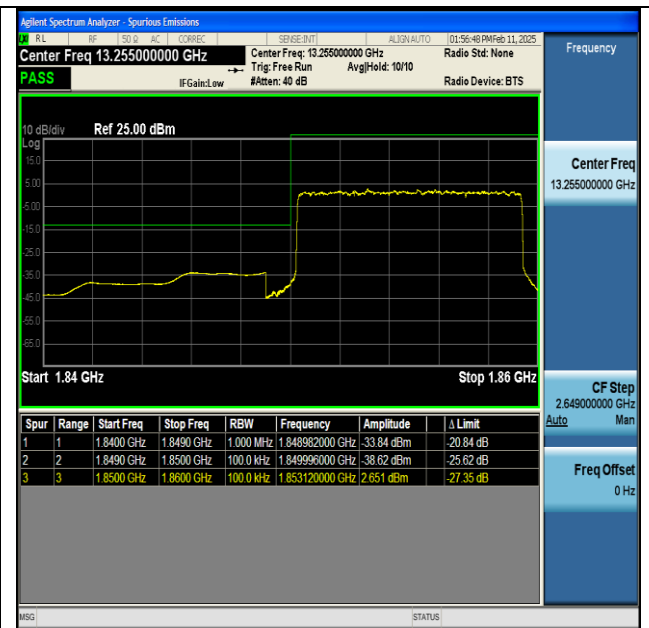
NTNV-n25-PC3-15-10-L-DFT-BPSK-Outer_Full-PASS
