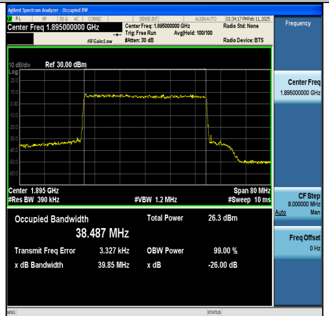
NTNV-n25-PC3-15-40-H-CP-256QAM-Outer_Full-Ant1-PASS
